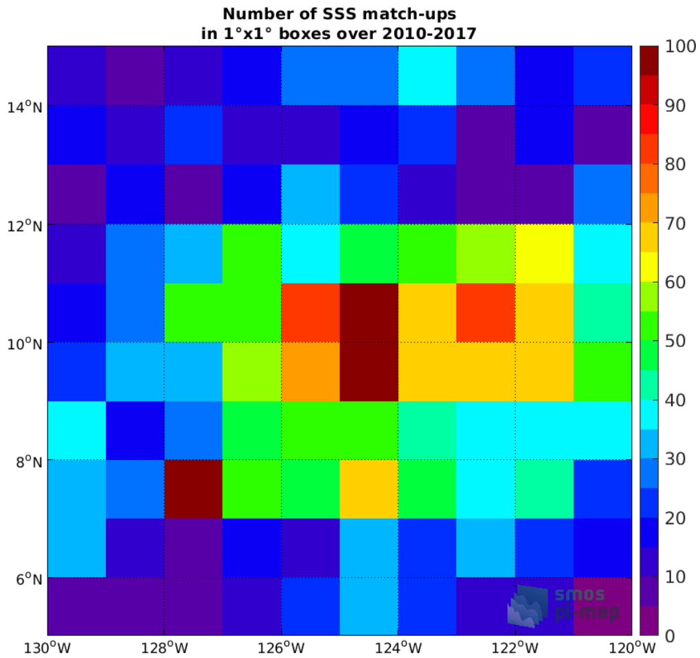
Figure 4: Number of SSS match-ups between Argo SSS and the SMOS L4 v2 Weekly (CATDS-CECOS-IFREMER) SSS product for the SPURS 2 Pi-MEP region over 1°x1° boxes and for the full satellite product period.
