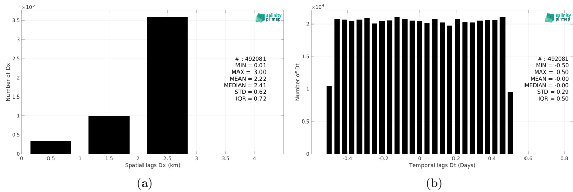
Figure 6: Histograms of the spatial (a) and temporal (b) lags between the location/time of the Waveglider (SPURS 2) measurement and the date of the corresponding SMOS SSS L4 v2 - Daily (BEC) SSS pixel.
