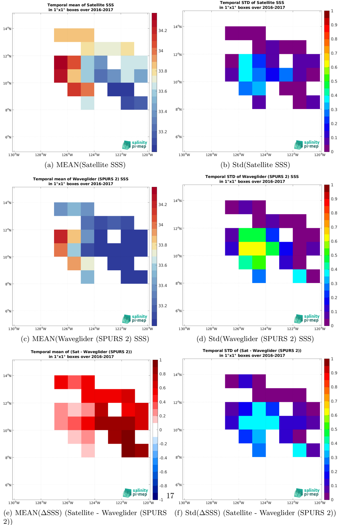
Figure 7: Temporal mean (left) and Std (right) of SSS from SMOS SSS L4 v2 - Daily (BEC) (top), Waveglider (SPURS 2) (middle), and of \Delta SSS (Satellite - Waveglider (SPURS 2)). Only match-up pairs are used to generate these maps.
