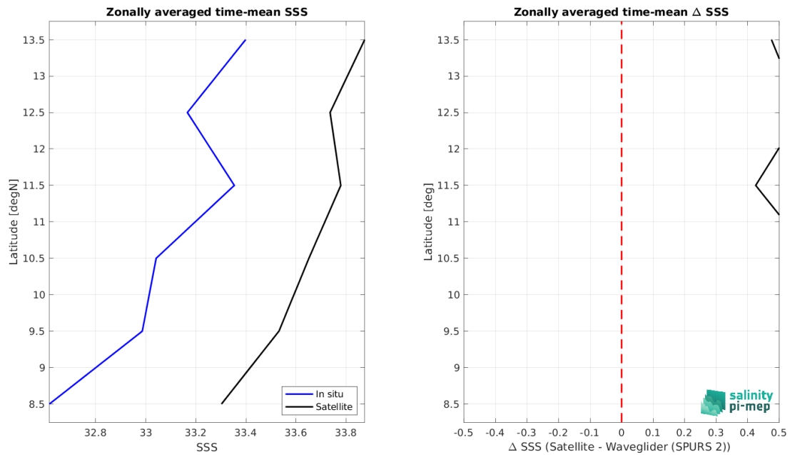
Figure 9: Left panel: Zonal mean SSS from SMOS SSS L4 v2 - Daily (BEC) satellite product (black) and from Waveglider (SPURS 2) (blue). Right panel: Zonal mean of \Delta SSS (Satellite - Waveglider (SPURS 2)) for all the collected Pi-MEP match-up pairs estimated over the full satellite product period.
