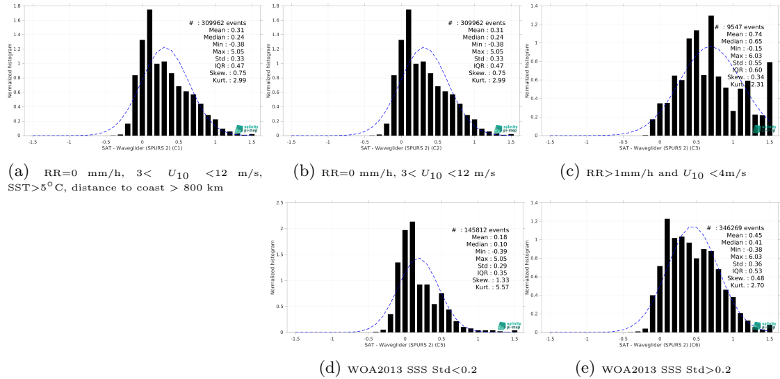
Figure 15: Normalized histogram of \Delta SSS (SMOS SSS L4 v2 - Daily (BEC) - Waveglider (SPURS 2)) for 5 different subdatasets corresponding to: RR=0 mm/h, 3 < U_{10} < 12 m/s, SST > 5°C, distance to coast > 800 km (a), RR=0 mm/h, 3 < U_{10} < 12 m/s (b), RR > 1mm/h and U_{10} < 4 m/s (c), WOA2013 SSS Std < 0.2 (d), WOA2013 SSS Std > 0.2 (e).
