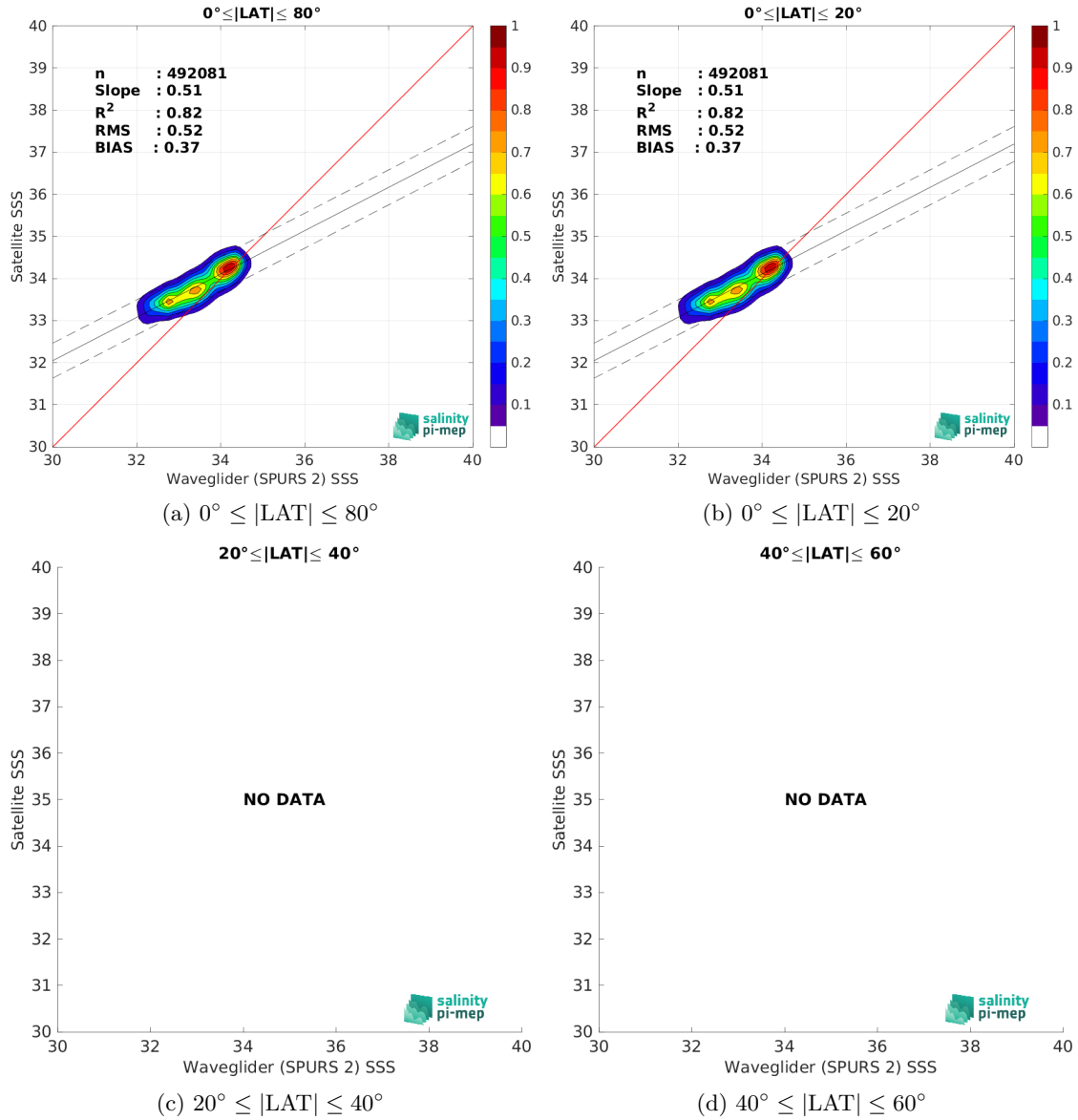
Figure 10: Contour maps of the concentration of SMOS SSS L4 v2 - Daily (BEC) SSS (y-axis) versus Waveglider (SPURS 2) SSS (x-axis) at match-up pairs for different latitude bands. For each plot, the red line shows x=y . The black thin and dashed lines indicate a linear fit through the data cloud and the \pm 95\% confidence levels, respectively. The number match-up pairs n , the slope and R^2 coefficient of the linear fit, the root mean square (RMS) and the mean bias between satellite and in situ data are indicated for each latitude band in each plots.
