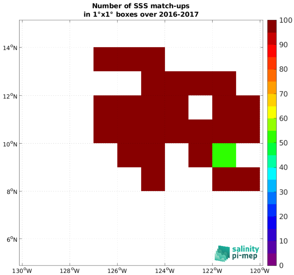
Figure 5: Number of SSS match-ups between Waveglider (SPURS 2) SSS and the SMOS SSS L4 v2 - Daily (BEC) SSS product for the SPURS 2 Pi-MEP region over 1^\circ \times 1^\circ boxes and for the full satellite product period.
