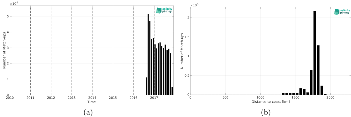
Figure 2: Number of match-ups between Waveglider (SPURS 2) and SMOS SSS L4 v2 - Daily (BEC) SSS as a function of time (a) and as function of the distance to coast (b) over the SPURS 2 Pi-MEP region and for the full satellite product period.
