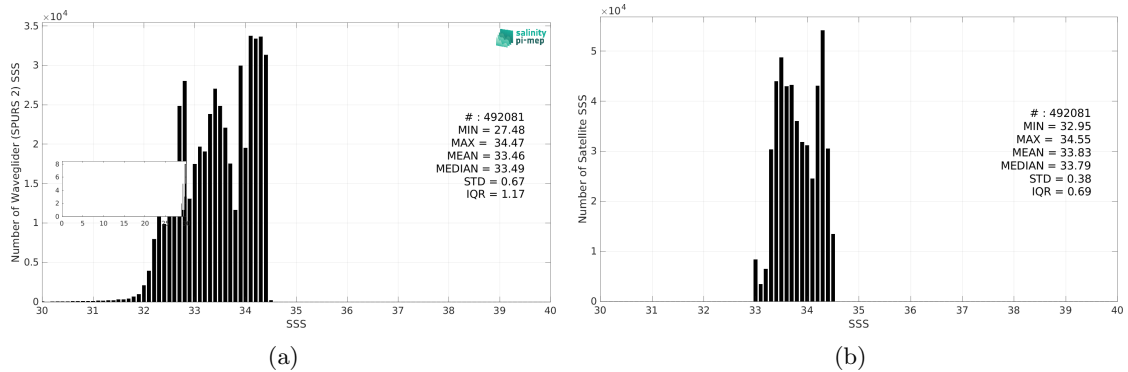
Figure 3: Histograms of SSS from Waveglider (SPURS 2) (a) and SMOS SSS L4 v2 - Daily (BEC) (b) considering all match-up pairs per bins of 0.1 over the SPURS 2 Pi-MEP region and for the full satellite product period.
