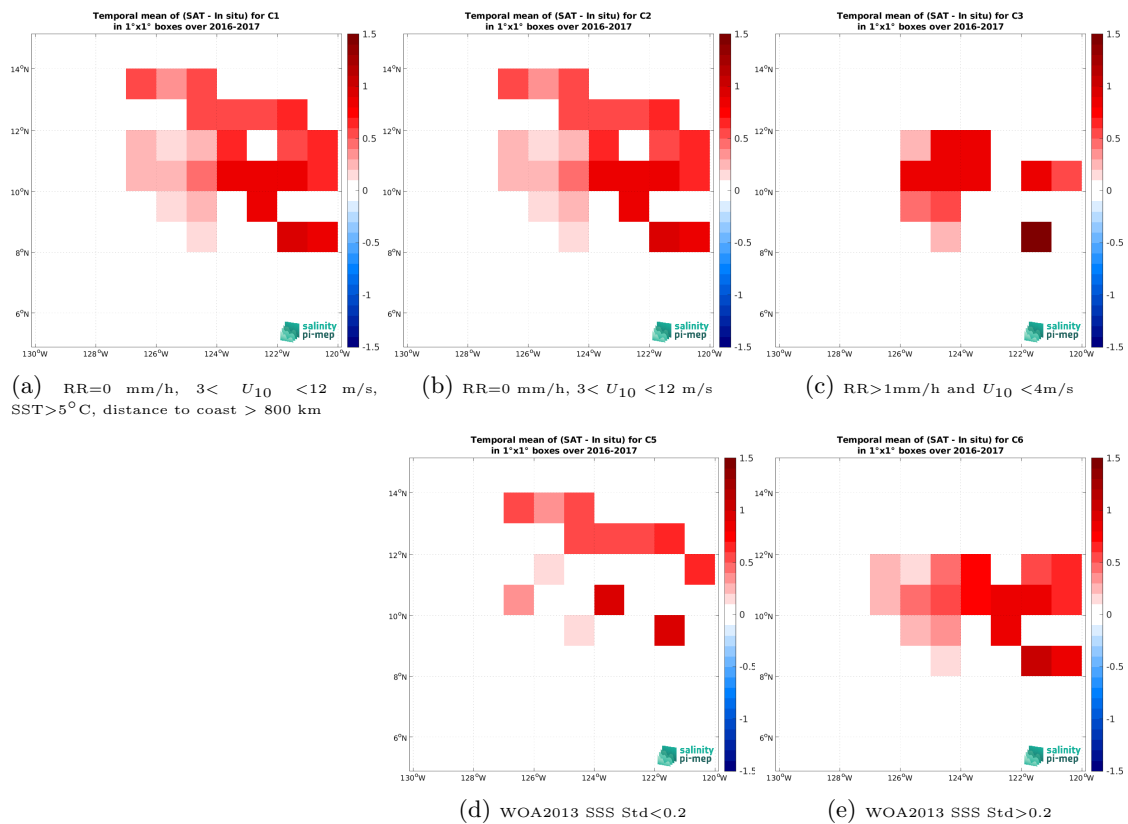
Figure 14: Temporal mean gridded over spatial boxes of size 1^\circ \times 1^\circ of \Delta SSS (SMOS SSS L4 v2 - Daily (BEC) - Waveglider (SPURS 2)) for 5 different subdatasets corresponding to:RR=0 mm/h, 3 < U_{10} < 12 m/s, SST > 5^\circ\text{C} , distance to coast > 800 km (a), RR=0 mm/h, 3 < U_{10} < 12 m/s (b), RR > 1 mm/h and U_{10} < 4 m/s (c), WOA2013 SSS Std < 0.2 (d), WOA2013 SSS Std > 0.2 (e).
