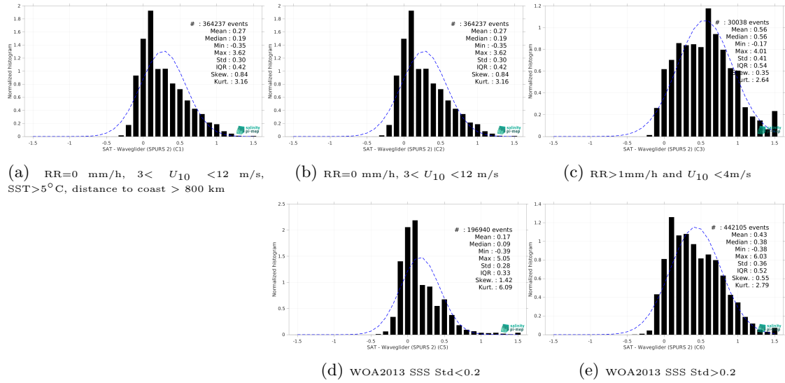
Figure 13: Normalized histogram of \Delta SSS (SMOS SSS L4 v2 - Daily (BEC) - Waveglider (SPURS 2)) for 5 different subdatasets corresponding to: RR=0 mm/h, 3 < U_{10} < 12 m/s, SST > 5°C, distance to coast > 800 km (a), RR=0 mm/h, 3 < U_{10} < 12 m/s (b), RR > 1mm/h and U_{10} < 4 m/s (c), WOA2013 SSS Std < 0.2 (d), WOA2013 SSS Std > 0.2 (e).
