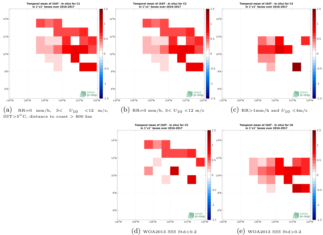
Figure 12: Temporal mean gridded over spatial boxes of size 1^\circ \times 1^\circ of \Delta SSS (SMOS SSS L4 v2 - Daily (BEC) - Waveglider (SPURS 2)) for 5 different subdatasets corresponding to:RR=0 mm/h, 3 < U_{10} < 12 m/s, SST >5^\circ C, distance to coast > 800 km (a), RR=0 mm/h, 3 < U_{10} < 12 m/s (b), RR >1 mm/h and U_{10} < 4 m/s (c), WOA2013 SSS Std <0.2 (d), WOA2013 SSS Std >0.2 (e).
