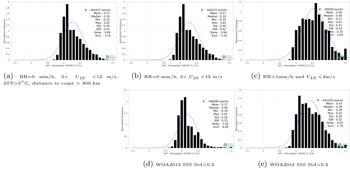
Figure 13: Normalized histogram of \Delta SSS (SMOS SSS L4 v2 - Daily (BEC) - Waveglider (SPURS 2)) for 5 different subdatasets corresponding to: RR=0 mm/h, 3 < U_{10} < 12 m/s, SST>5°C, distance to coast > 800 km (a), RR=0 mm/h, 3 < U_{10} < 12 m/s (b), RR>1mm/h and U_{10} < 4 m/s (c), WOA2013 SSS Std<0.2 (d), WOA2013 SSS Std>0.2 (e).
