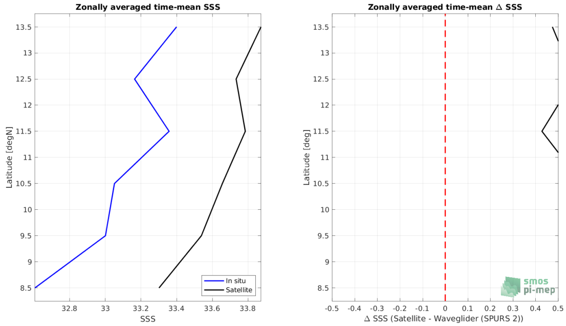
Figure 8: Left panel: Zonal mean SSS from SMOS SSS L4 v2 - Daily (BEC) satellite product (black) and from Waveglider (SPURS 2) (blue). Right panel: Zonal mean of \Delta SSS (Satellite - Waveglider (SPURS 2)) for all the collected Pi-MEP match-up pairs estimated over the full satellite product period.
