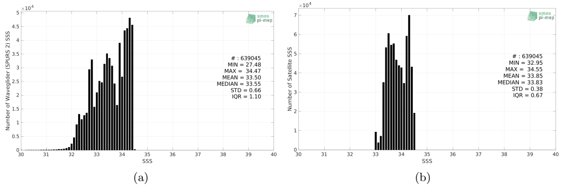
Figure 2: Histograms of SSS from Waveglider (SPURS 2) (a) and SMOS SSS L4 v2 - Daily (BEC) (b) considering all match-up pairs per bins of 0.1 over the SPURS 2 Pi-MEP region and for the full satellite product period.
