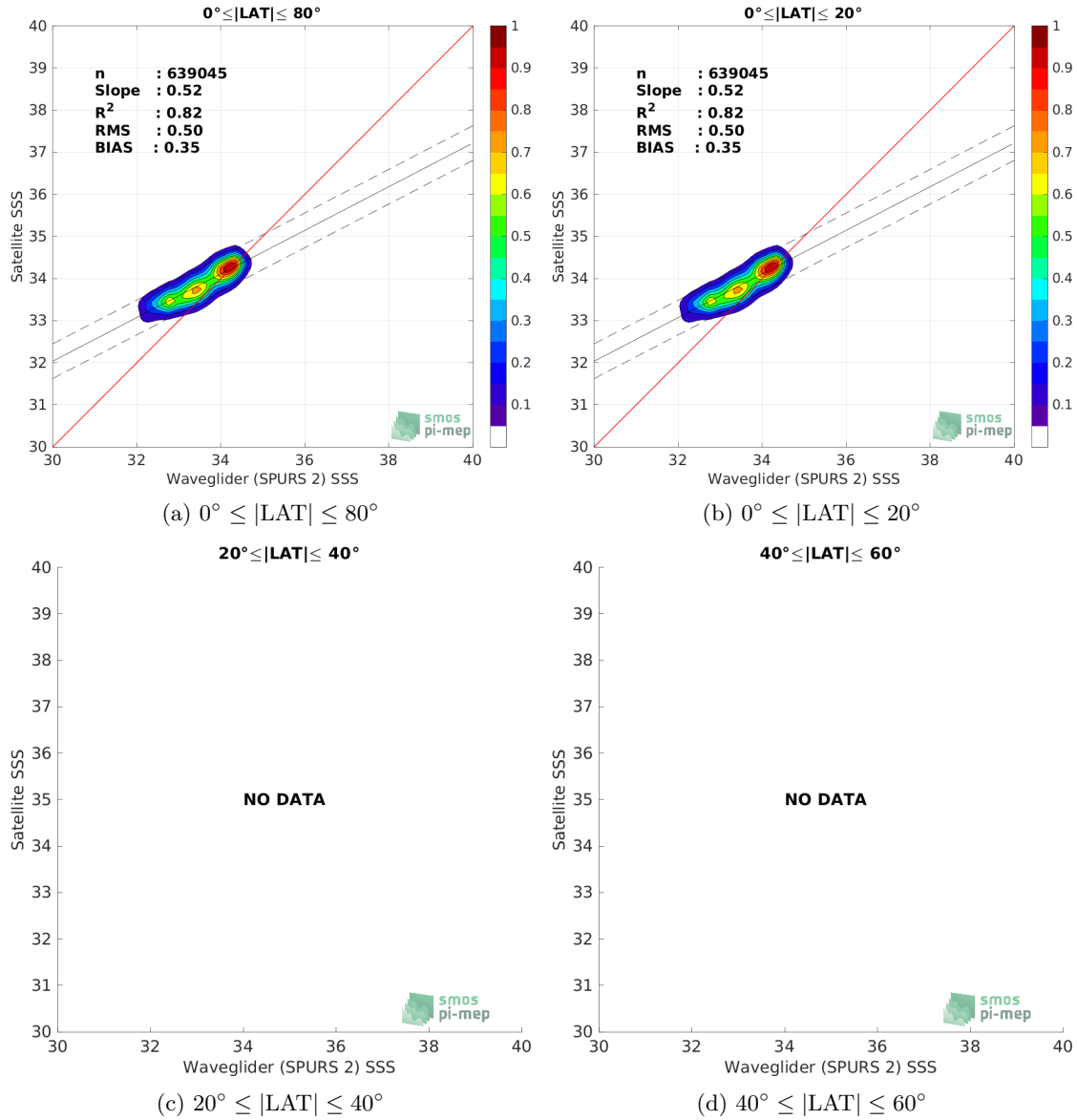
Figure 9: Contour maps of the concentration of SMOS SSS L4 v2 - Daily (BEC) SSS (y-axis) versus Waveglider (SPURS 2) SSS (x-axis) at match-up pairs for different latitude bands. For each plot, the red line shows x=y . The black thin and dashed lines indicate a linear fit through the data cloud and the \pm 95\% confidence levels, respectively. The number match-up pairs n , the slope and R^2 coefficient of the linear fit, the root mean square (RMS) and the mean bias between satellite and in situ data are indicated for each latitude band in each plots.
