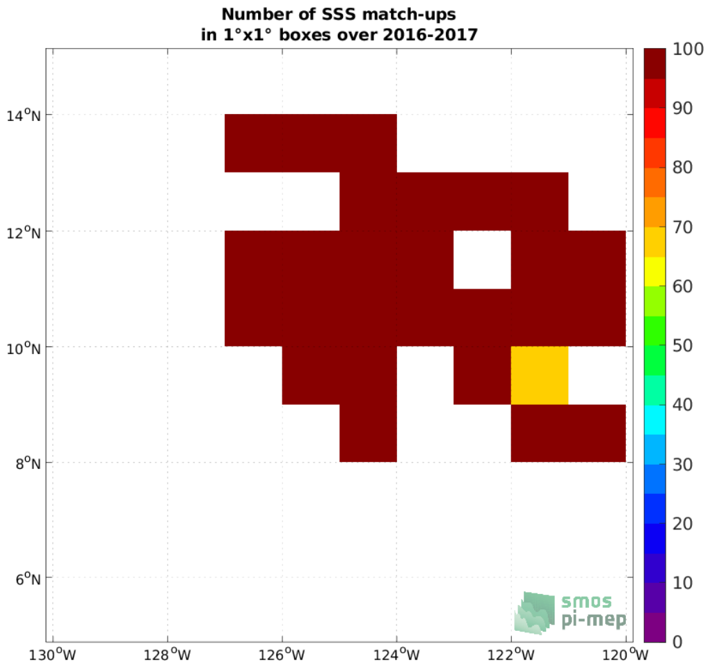
Figure 4: Number of SSS match-ups between Waveglider (SPURS 2) SSS and the SMOS SSS L4 v2 - Daily (BEC) SSS product for the SPURS 2 Pi-MEP region over 1°x1° boxes and for the full satellite product period.
