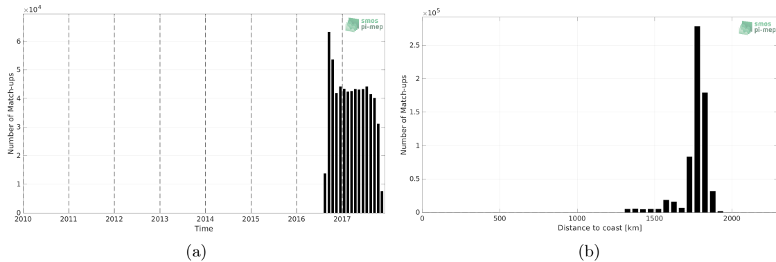
Figure 1: Number of match-ups between Waveglider (SPURS 2) and SMOS SSS L4 v2 - Daily (BEC) SSS as a function of time (a) and as function of the distance to coast (b) over the SPURS 2 Pi-MEP region and for the full satellite product period.
