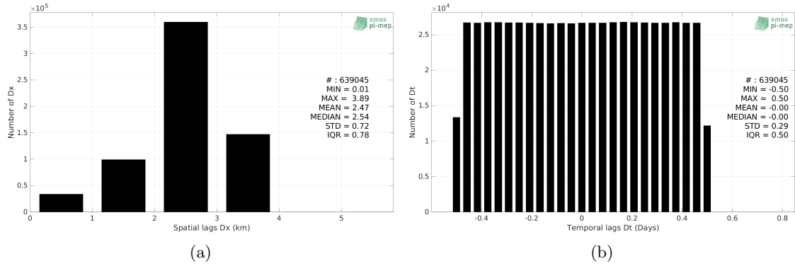
Figure 5: Histograms of the spatial (a) and temporal (b) lags between the location/time of the Waveglider (SPURS 2) measurement and the date of the corresponding SMOS SSS L4 v2 - Daily (BEC) SSS pixel.
