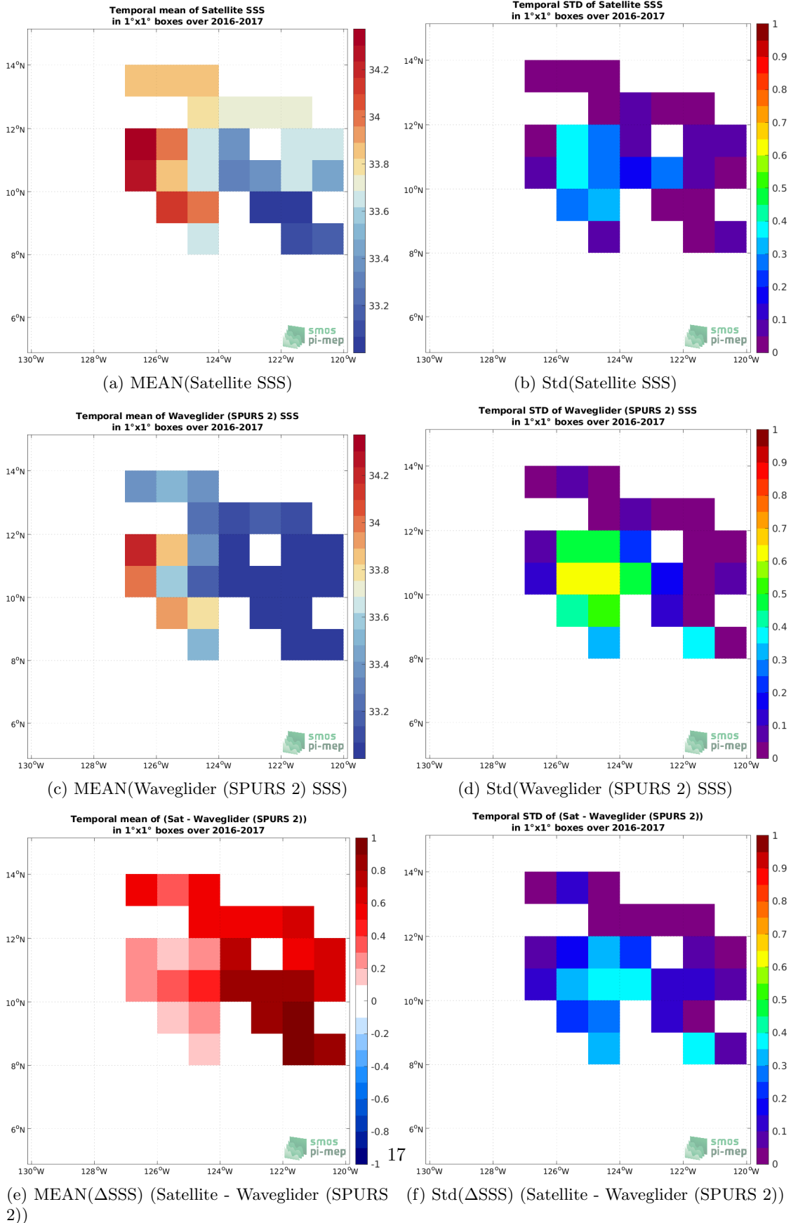
Figure 6: Temporal mean (left) and Std (right) of SSS from SMOS SSS L4 v2 - Daily (BEC) (top), Waveglider (SPURS 2) (middle), and of \Delta SSS (Satellite - Waveglider (SPURS 2)). Only match-up pairs are used to generate these maps.
