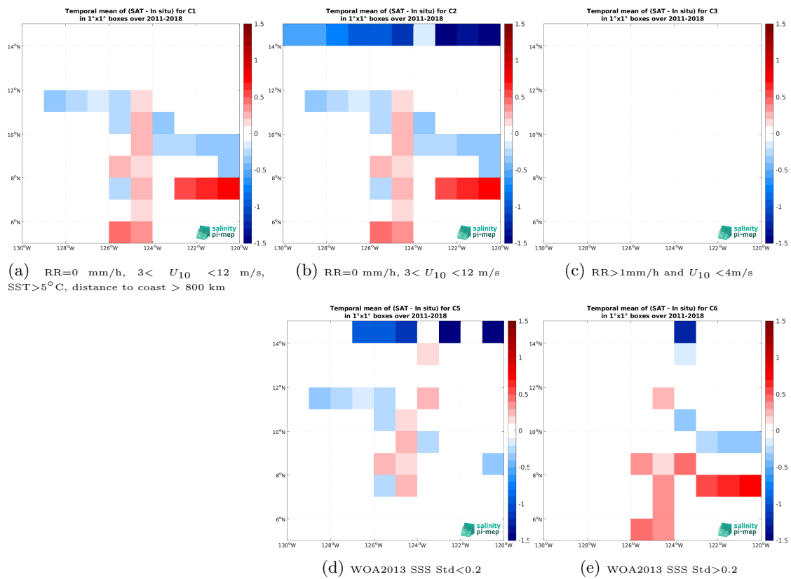
Figure 14: Temporal mean gridded over spatial boxes of size 1^\circ \times 1^\circ of \Delta\text{SSS} (SMOS SSS L4 v2 - Daily (BEC) - TSG (SAMOS)) for 5 different subdatasets corresponding to:RR=0 mm/h, 3 < U_{10} < 12 m/s, SST > 5°C, distance to coast > 800 km (a), RR=0 mm/h, 3 < U_{10} < 12 m/s (b), RR > 1mm/h and U_{10} < 4 m/s (c), WOA2013 SSS Std < 0.2 (d), WOA2013 SSS Std > 0.2 (e).
