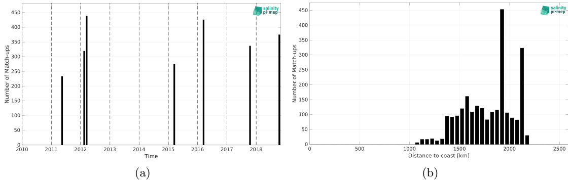
Figure 2: Number of match-ups between TSG (SAMOS) and SMOS SSS L4 v2 - Daily (BEC) SSS as a function of time (a) and as function of the distance to coast (b) over the SPURS 2 Pi-MEP region and for the full satellite product period.
