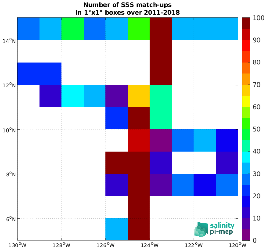
Figure 5: Number of SSS match-ups between TSG (SAMOS) SSS and the SMOS SSS L4 v2 - Daily (BEC) SSS product for the SPURS 2 Pi-MEP region over 1^\circ \times 1^\circ boxes and for the full satellite product period.
