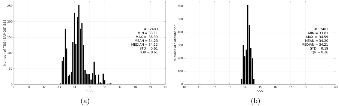
Figure 3: Histograms of SSS from TSG (SAMOS) (a) and SMOS SSS L4 v2 - Daily (BEC) (b) considering all match-up pairs per bins of 0.1 over the SPURS 2 Pi-MEP region and for the full satellite product period.
