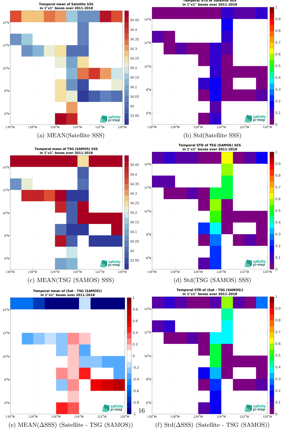
Figure 7: Temporal mean (left) and Std (right) of SSS from SMOS SSS L4 v2 - Daily (BEC) (top), TSG (SAMOS) (middle), and of \Delta SSS (Satellite - TSG (SAMOS)). Only match-up pairs are used to generate these maps.
