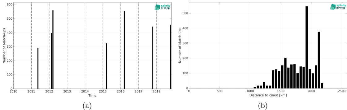
Figure 1: Number of match-ups between TSG (SAMOS) and SMOS SSS L4 v2 - Daily (BEC) SSS as a function of time (a) and as function of the distance to coast (b) over the SPURS 2 Pi-MEP region and for the full satellite product period.
