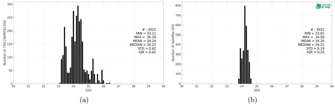
Figure 2: Histograms of SSS from TSG (SAMOS) (a) and SMOS SSS L4 v2 - Daily (BEC) (b) considering all match-up pairs per bins of 0.1 over the SPURS 2 Pi-MEP region and for the full satellite product period.
