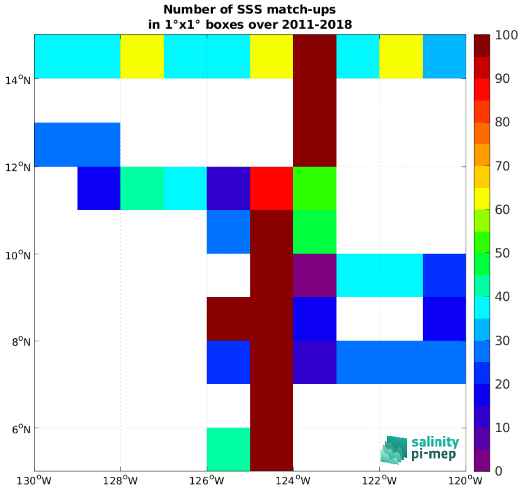
Figure 4: Number of SSS match-ups between TSG (SAMOS) SSS and the SMOS SSS L4 v2 - Daily (BEC) SSS product for the SPURS 2 Pi-MEP region over 1^\circ \times 1^\circ boxes and for the full satellite product period.
