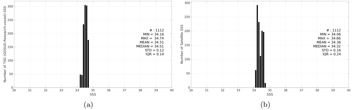
Figure 3: Histograms of SSS from TSG (GOSUD-Research-vessel) (a) and SMOS SSS L4 v2 - Daily (BEC) (b) considering all match-up pairs per bins of 0.1 over the SPURS 2 Pi-MEP region and for the full satellite product period.
