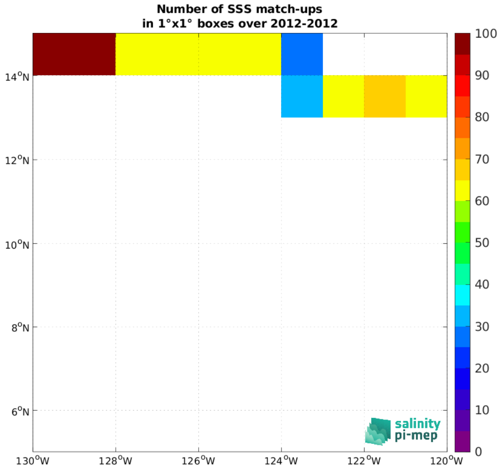
Figure 5: Number of SSS match-ups between TSG (GOSUD-Research-vessel) SSS and the SMOS SSS L4 v2 - Daily (BEC) SSS product for the SPURS 2 Pi-MEP region over 1^\circ \times 1^\circ boxes and for the full satellite product period.
