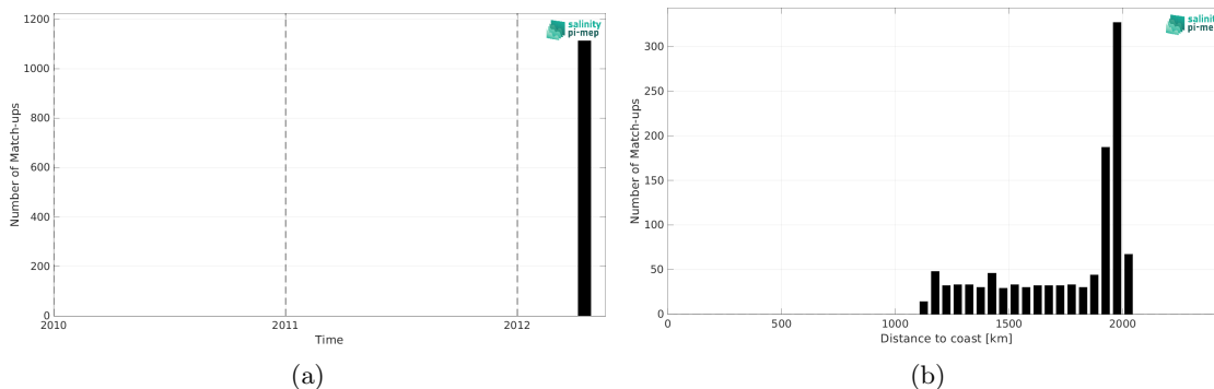
Figure 2: Number of match-ups between TSG (GOSUD-Research-vessel) and SMOS SSS L4 v2 - Daily (BEC) SSS as a function of time (a) and as function of the distance to coast (b) over the SPURS 2 Pi-MEP region and for the full satellite product period.
