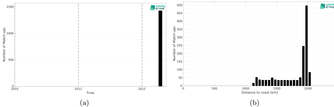
Figure 1: Number of match-ups between TSG (GOSUD-Research-vessel) and SMOS SSS L4 v2 - Daily (BEC) SSS as a function of time (a) and as function of the distance to coast (b) over the SPURS 2 Pi-MEP region and for the full satellite product period.
