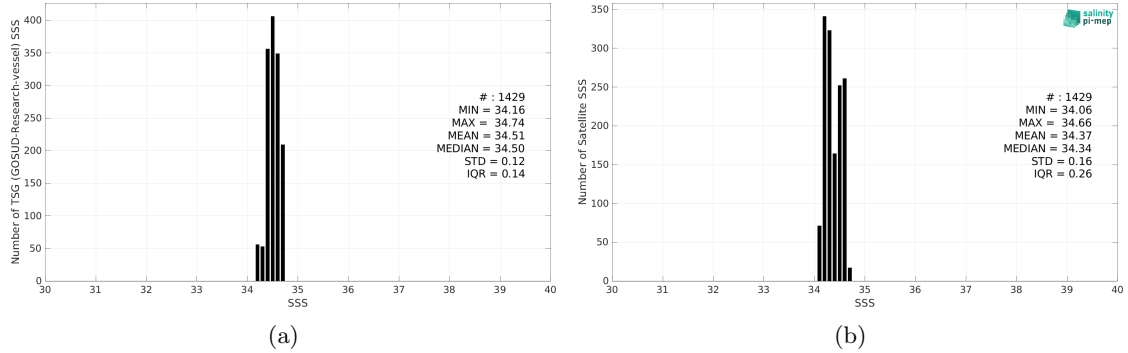
Figure 2: Histograms of SSS from TSG (GOSUD-Research-vessel) (a) and SMOS SSS L4 v2 - Daily (BEC) (b) considering all match-up pairs per bins of 0.1 over the SPURS 2 Pi-MEP region and for the full satellite product period.
