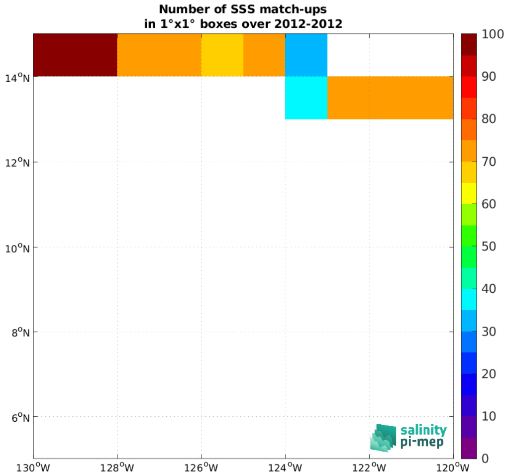
Figure 4: Number of SSS match-ups between TSG (GOSUD-Research-vessel) SSS and the SMOS SSS L4 v2 - Daily (BEC) SSS product for the SPURS 2 Pi-MEP region over 1^\circ \times 1^\circ boxes and for the full satellite product period.
