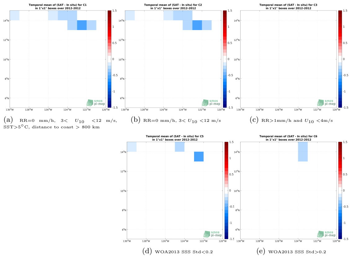
Figure 12: Temporal mean gridded over spatial boxes of size 1^\circ \times 1^\circ of \Delta\text{SSS} (SMOS SSS L4 v2 - Daily (BEC) - TSG (GOSUD-Research-vessel)) for 5 different subdatasets corresponding to:RR=0 mm/h, 3 < U_{10} < 12 m/s, SST >5^\circ\text{C} , distance to coast > 800 km (a), RR=0 mm/h, 3 < U_{10} < 12 m/s (b), RR >1 mm/h and U_{10} < 4 m/s (c), WOA2013 SSS Std <0.2 (d), WOA2013 SSS Std >0.2 (e).
