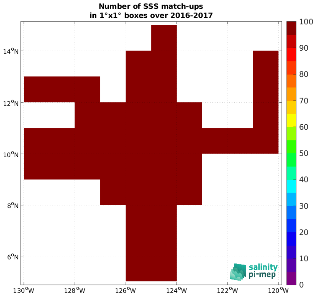
Figure 5: Number of SSS match-ups between Salinity Snake (SPURS 2) SSS and the SMOS SSS L4 v2 - Daily (BEC) SSS product for the SPURS 2 Pi-MEP region over 1^\circ \times 1^\circ boxes and for the full satellite product period.
