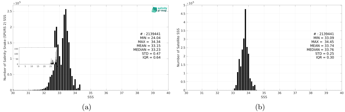
Figure 3: Histograms of SSS from Salinity Snake (SPURS 2) (a) and SMOS SSS L4 v2 - Daily (BEC) (b) considering all match-up pairs per bins of 0.1 over the SPURS 2 Pi-MEP region and for the full satellite product period.
