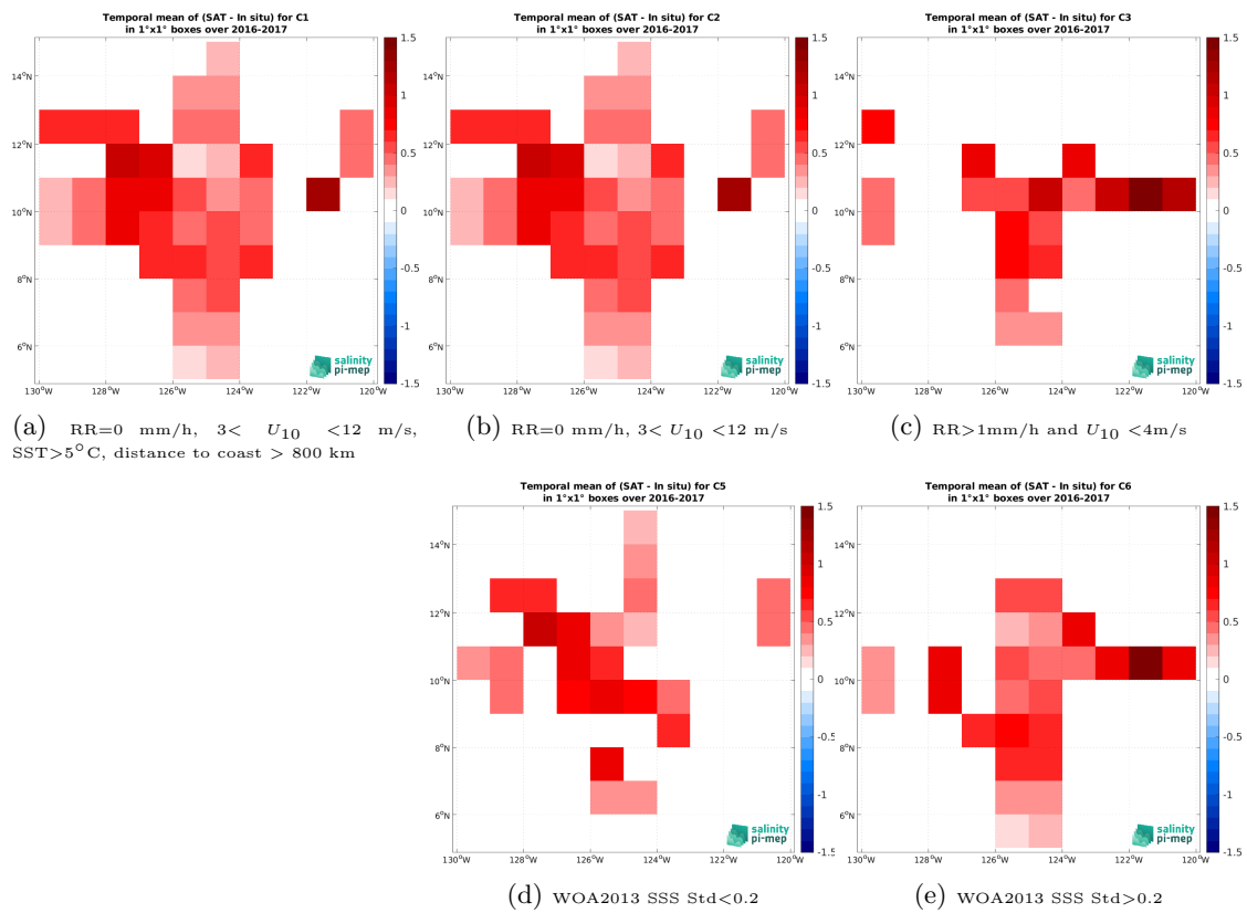
Figure 14: Temporal mean gridded over spatial boxes of size 1^\circ \times 1^\circ of \Delta SSS (SMOS SSS L4 v2 - Daily (BEC) - Salinity Snake (SPURS 2)) for 5 different subdatasets corresponding to:RR=0 mm/h, 3 < U_{10} < 12 m/s, SST > 5^\circ\text{C} , distance to coast > 800 km (a), RR=0 mm/h, 3 < U_{10} < 12 m/s (b), RR > 1 mm/h and U_{10} < 4 m/s (c), WOA2013 SSS Std < 0.2 (d), WOA2013 SSS Std > 0.2 (e).
