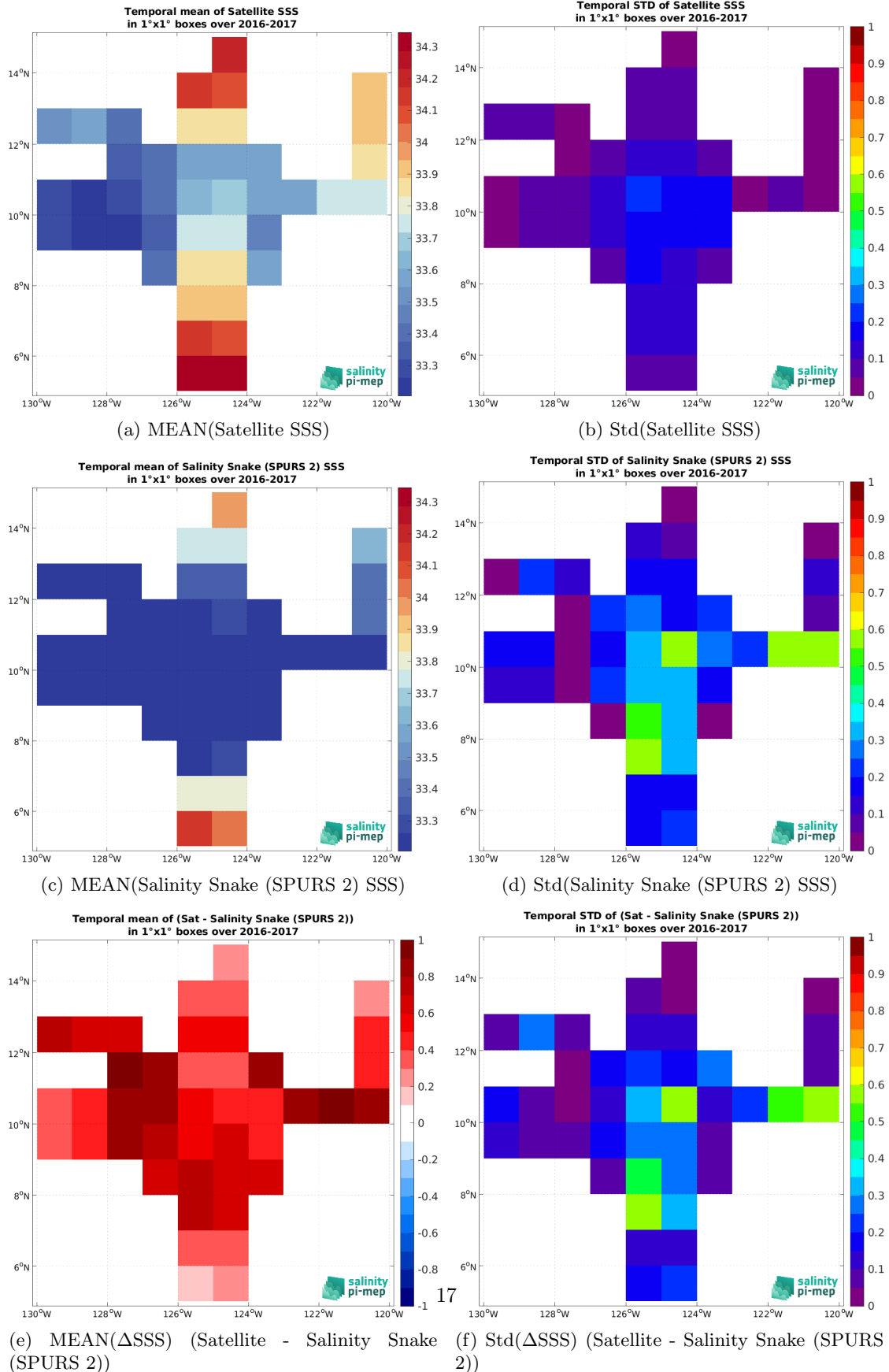
Figure 7: Temporal mean (left) and Std (right) of SSS from SMOS SSS L4 v2 - Daily (BEC) (top), Salinity Snake (SPURS 2) (middle), and of \Delta SSS (Satellite - Salinity Snake (SPURS 2)). Only match-up pairs are used to generate these maps.
