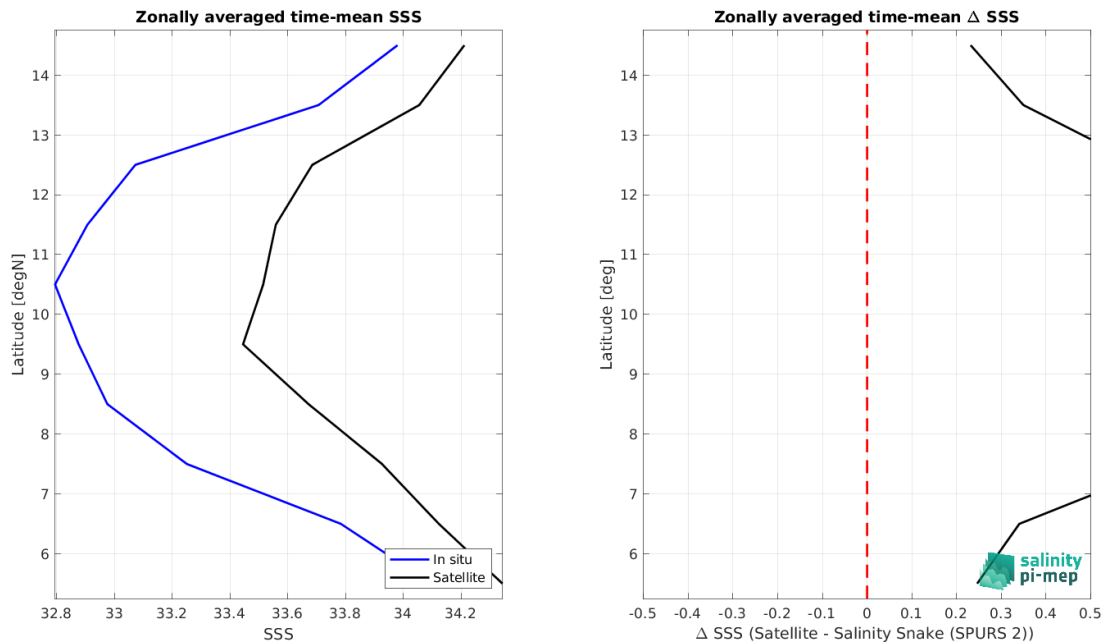
Figure 9: Left panel: Zonal mean SSS from SMOS SSS L4 v2 - Daily (BEC) satellite product (black) and from Salinity Snake (SPURS 2) (blue). Right panel: Zonal mean of \Delta SSS (Satellite - Salinity Snake (SPURS 2)) for all the collected Pi-MEP match-up pairs estimated over the full satellite product period.
