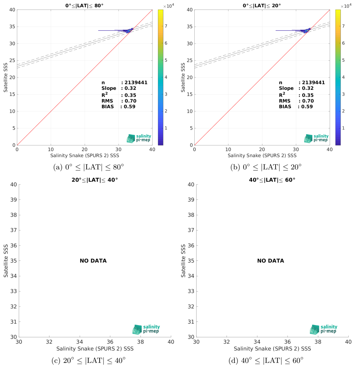
Figure 10: Contour maps of the concentration of SMOS SSS L4 v2 - Daily (BEC) SSS (y-axis) versus Salinity Snake (SPURS 2) SSS (x-axis) at match-up pairs for different latitude bands. For each plot, the red line shows x=y . The black thin and dashed lines indicate a linear fit through the data cloud and the \pm 95\% confidence levels, respectively. The number match-up pairs n , the slope and R^2 coefficient of the linear fit, the root mean square (RMS) and the mean bias between satellite and in situ data are indicated for each latitude band in each plots.
