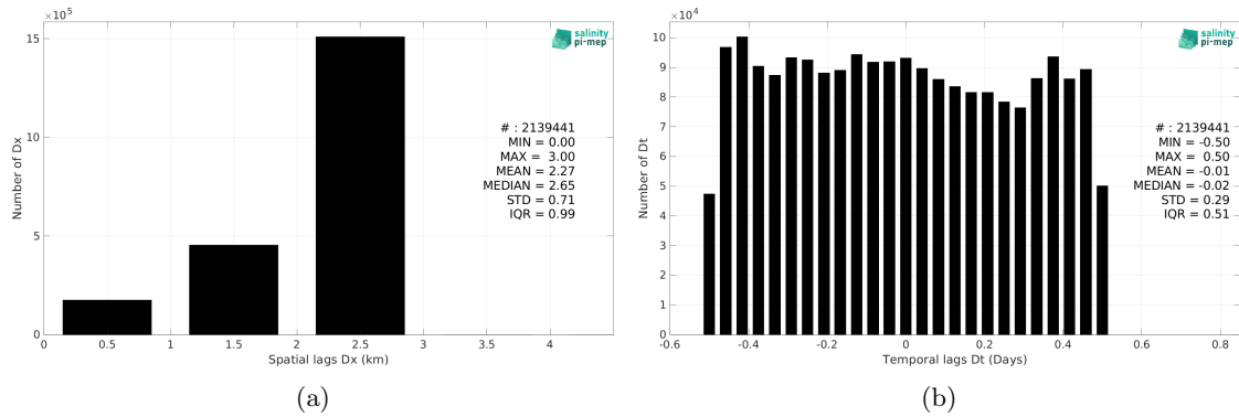
Figure 6: Histograms of the spatial (a) and temporal (b) lags between the location/time of the Salinity Snake (SPURS 2) measurement and the date of the corresponding SMOS SSS L4 v2 - Daily (BEC) SSS pixel.
