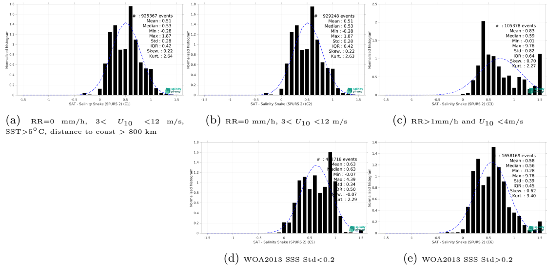
Figure 15: Normalized histogram of \Delta SSS (SMOS SSS L4 v2 - Daily (BEC) - Salinity Snake (SPURS 2)) for 5 different subdatasets corresponding to: RR=0 mm/h, 3 < U_{10} < 12 m/s, SST>5°C, distance to coast > 800 km (a), RR=0 mm/h, 3 < U_{10} < 12 m/s (b), RR>1mm/h and U_{10} < 4 m/s (c), WOA2013 SSS Std<0.2 (d), WOA2013 SSS Std>0.2 (e).
