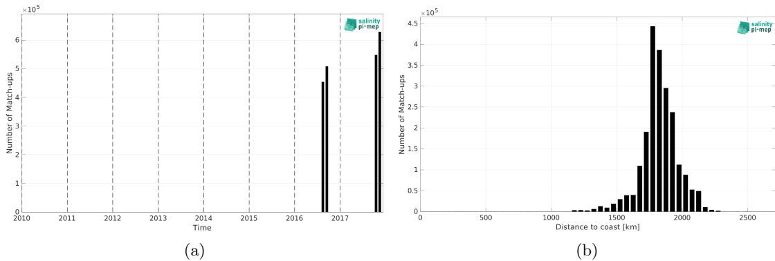
Figure 2: Number of match-ups between Salinity Snake (SPURS 2) and SMOS SSS L4 v2 - Daily (BEC) SSS as a function of time (a) and as function of the distance to coast (b) over the SPURS 2 Pi-MEP region and for the full satellite product period.
