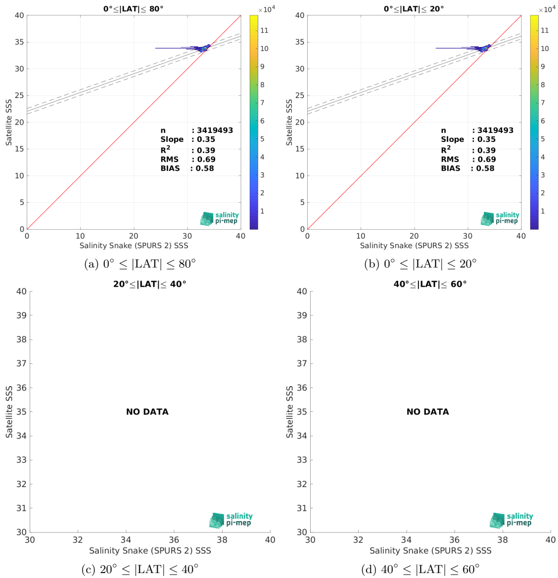
Figure 9: Contour maps of the concentration of SMOS SSS L4 v2 - Daily (BEC) SSS (y-axis) versus Salinity Snake (SPURS 2) SSS (x-axis) at match-up pairs for different latitude bands. For each plot, the red line shows x=y . The black thin and dashed lines indicate a linear fit through the data cloud and the \pm 95\% confidence levels, respectively. The number match-up pairs n , the slope and R^2 coefficient of the linear fit, the root mean square (RMS) and the mean bias between satellite and in situ data are indicated for each latitude band in each plots.
