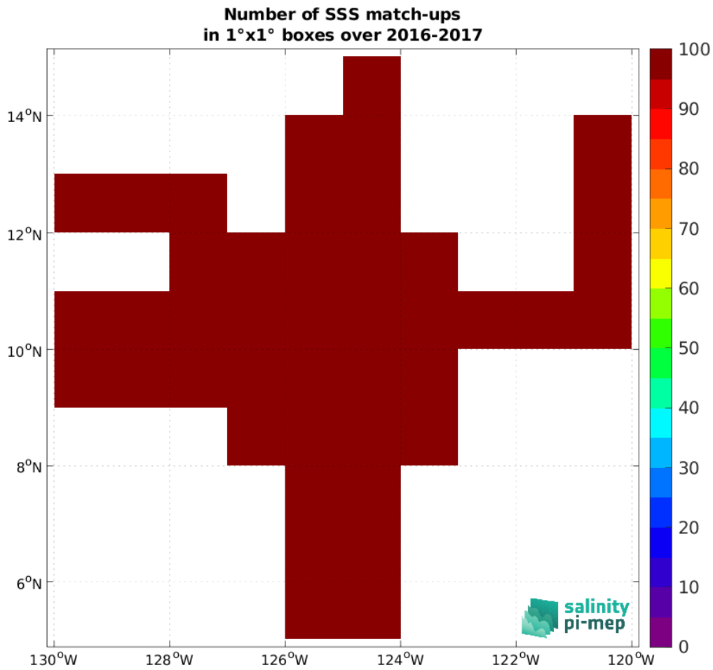
Figure 4: Number of SSS match-ups between Salinity Snake (SPURS 2) SSS and the SMOS SSS L4 v2 - Daily (BEC) SSS product for the SPURS 2 Pi-MEP region over 1^\circ \times 1^\circ boxes and for the full satellite product period.
