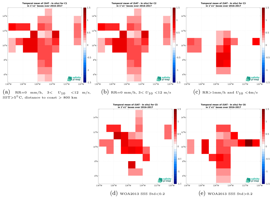
Figure 12: Temporal mean gridded over spatial boxes of size 1^\circ \times 1^\circ of \Delta SSS (SMOS SSS L4 v2 - Daily (BEC) - Salinity Snake (SPURS 2)) for 5 different subdatasets corresponding to:RR=0 mm/h, 3 < U_{10} < 12 m/s, SST > 5^\circ\text{C} , distance to coast > 800 km (a), RR=0 mm/h, 3 < U_{10} < 12 m/s (b), RR > 1 mm/h and U_{10} < 4 m/s (c), WOA2013 SSS Std < 0.2 (d), WOA2013 SSS Std > 0.2 (e).
