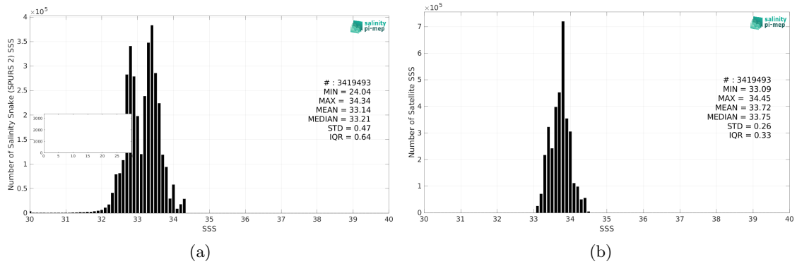
Figure 2: Histograms of SSS from Salinity Snake (SPURS 2) (a) and SMOS SSS L4 v2 - Daily (BEC) (b) considering all match-up pairs per bins of 0.1 over the SPURS 2 Pi-MEP region and for the full satellite product period.
