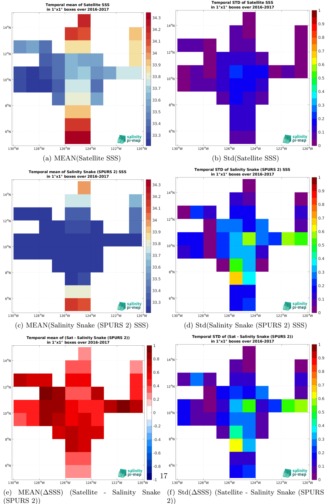
Figure 6: Temporal mean (left) and Std (right) of SSS from SMOS SSS L4 v2 - Daily (BEC) (top), Salinity Snake (SPURS 2) (middle), and of \Delta SSS (Satellite - Salinity Snake (SPURS 2)). Only match-up pairs are used to generate these maps.
