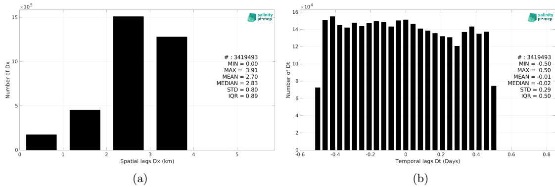
Figure 5: Histograms of the spatial (a) and temporal (b) lags between the location/time of the Salinity Snake (SPURS 2) measurement and the date of the corresponding SMOS SSS L4 v2 - Daily (BEC) SSS pixel.
