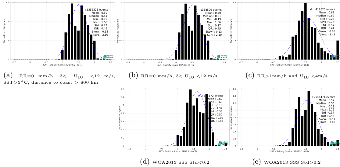
Figure 13: Normalized histogram of \Delta SSS (SMOS SSS L4 v2 - Daily (BEC) - Salinity Snake (SPURS 2)) for 5 different subdatasets corresponding to: RR=0 mm/h, 3 < U_{10} < 12 m/s, SST > 5°C, distance to coast > 800 km (a), RR=0 mm/h, 3 < U_{10} < 12 m/s (b), RR > 1mm/h and U_{10} < 4 m/s (c), WOA2013 SSS Std < 0.2 (d), WOA2013 SSS Std > 0.2 (e).
