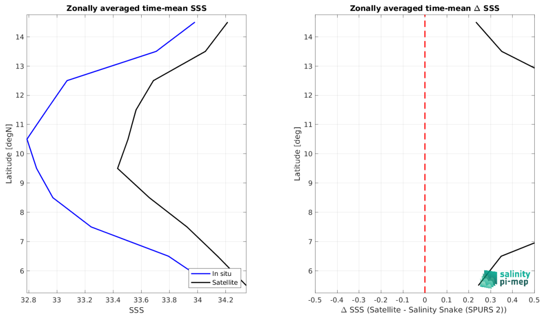
Figure 8: Left panel: Zonal mean SSS from SMOS SSS L4 v2 - Daily (BEC) satellite product (black) and from Salinity Snake (SPURS 2) (blue). Right panel: Zonal mean of \Delta SSS (Satellite - Salinity Snake (SPURS 2)) for all the collected Pi-MEP match-up pairs estimated over the full satellite product period.
