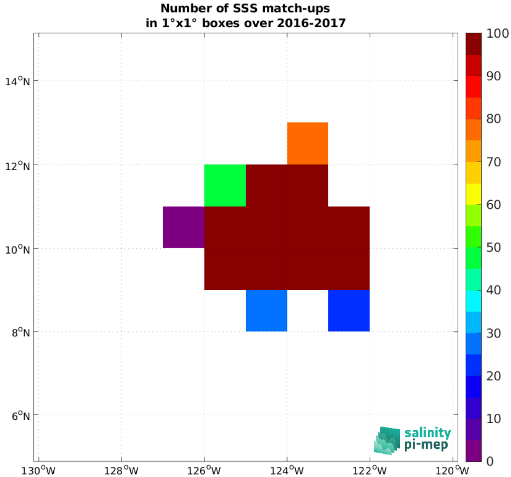
Figure 5: Number of SSS match-ups between Seagliders (SPURS 2) SSS and the SMOS SSS L4 v2 - Daily (BEC) SSS product for the SPURS 2 Pi-MEP region over 1^\circ \times 1^\circ boxes and for the full satellite product period.
