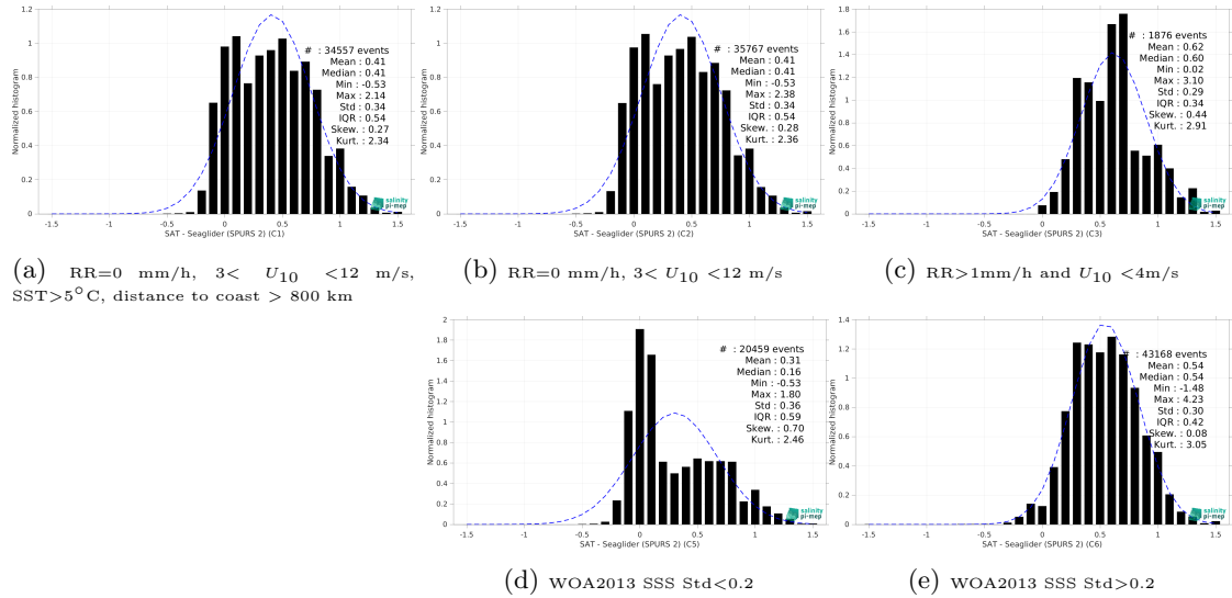
Figure 15: Normalized histogram of \Delta SSS (SMOS SSS L4 v2 - Daily (BEC) - Seaglider (SPURS 2)) for 5 different subdatasets corresponding to: RR=0 mm/h, 3 < U_{10} < 12 m/s, SST > 5°C, distance to coast > 800 km (a), RR=0 mm/h, 3 < U_{10} < 12 m/s (b), RR > 1mm/h and U_{10} < 4 m/s (c), WOA2013 SSS Std < 0.2 (d), WOA2013 SSS Std > 0.2 (e).
