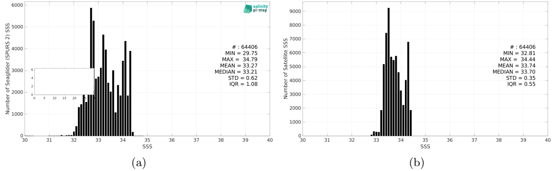
Figure 3: Histograms of SSS from Seaglider (SPURS 2) (a) and SMOS SSS L4 v2 - Daily (BEC) (b) considering all match-up pairs per bins of 0.1 over the SPURS 2 Pi-MEP region and for the full satellite product period.
