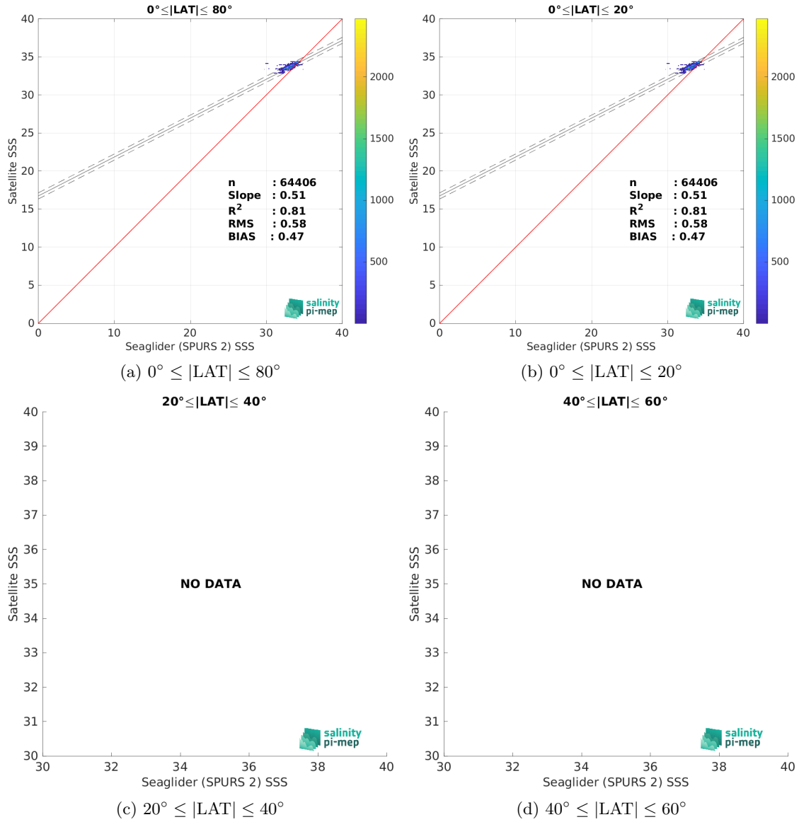
Figure 10: Contour maps of the concentration of SMOS SSS L4 v2 - Daily (BEC) SSS (y-axis) versus Seaglider (SPURS 2) SSS (x-axis) at match-up pairs for different latitude bands. For each plot, the red line shows x=y . The black thin and dashed lines indicate a linear fit through the data cloud and the \pm 95\% confidence levels, respectively. The number match-up pairs n , the slope and R^2 coefficient of the linear fit, the root mean square (RMS) and the mean bias between satellite and in situ data are indicated for each latitude band in each plots.
