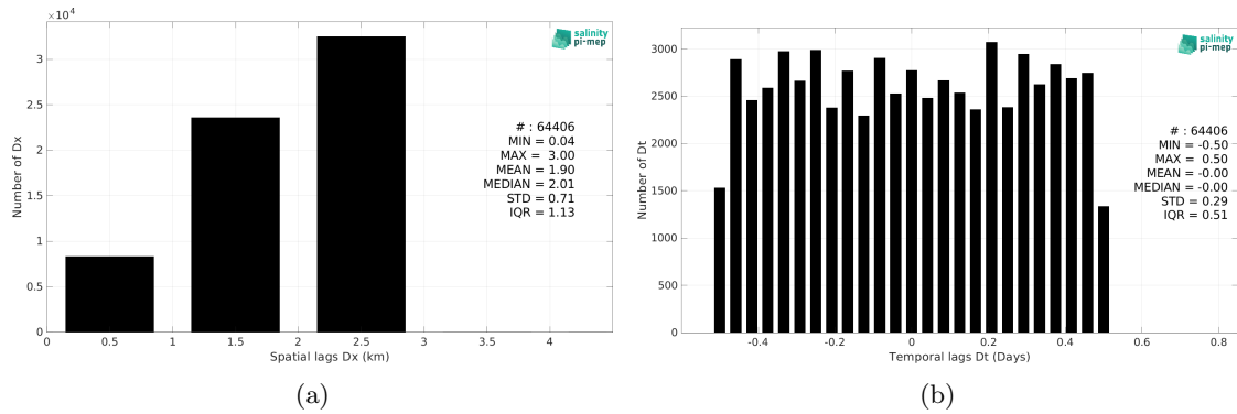
Figure 6: Histograms of the spatial (a) and temporal (b) lags between the location/time of the Seaglider (SPURS 2) measurement and the date of the corresponding SMOS SSS L4 v2 - Daily (BEC) SSS pixel.
