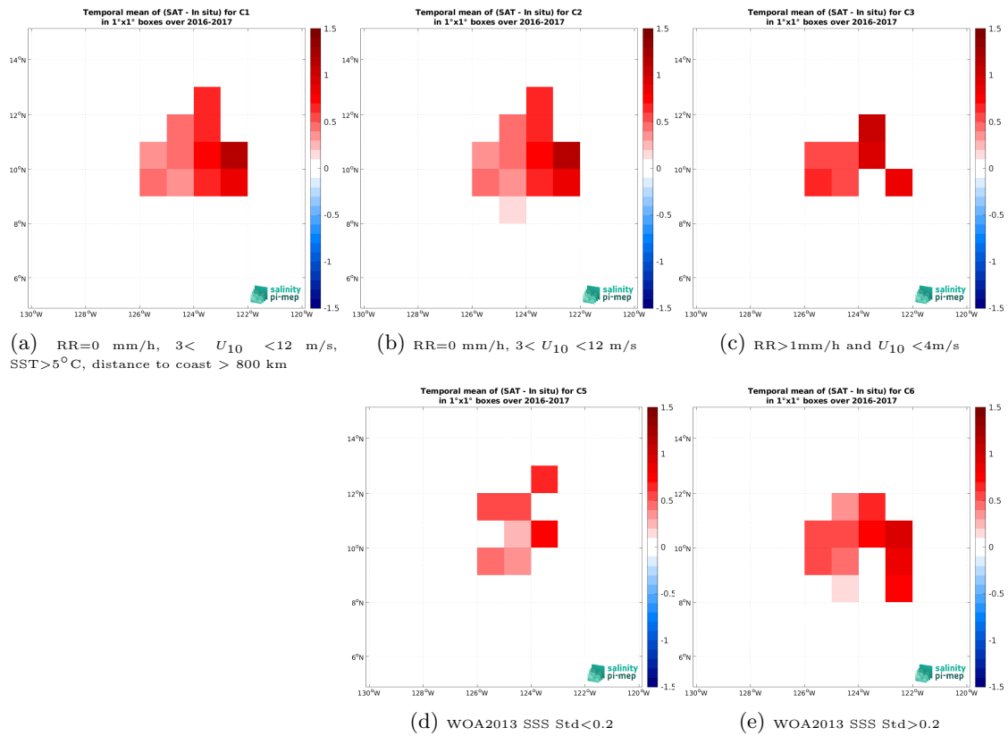
Figure 14: Temporal mean gridded over spatial boxes of size 1^\circ \times 1^\circ of \Delta SSS (SMOS SSS L4 v2 - Daily (BEC) - Seaglider (SPURS 2)) for 5 different subdatasets corresponding to:RR=0 mm/h, 3 < U_{10} < 12 m/s, SST > 5^\circ\text{C} , distance to coast > 800 km (a), RR=0 mm/h, 3 < U_{10} < 12 m/s (b), RR > 1 mm/h and U_{10} < 4 m/s (c), WOA2013 SSS Std < 0.2 (d), WOA2013 SSS Std > 0.2 (e).
