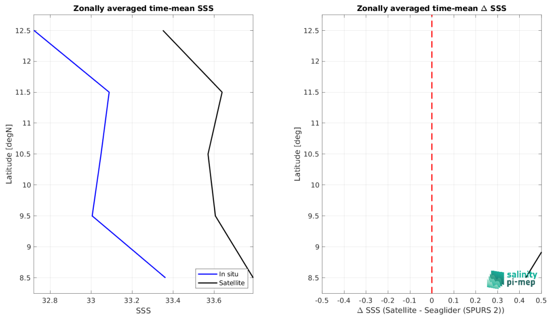
Figure 9: Left panel: Zonal mean SSS from SMOS SSS L4 v2 - Daily (BEC) satellite product (black) and from Seaglider (SPURS 2) (blue). Right panel: Zonal mean of \Delta SSS (Satellite - Seaglider (SPURS 2)) for all the collected Pi-MEP match-up pairs estimated over the full satellite product period.
