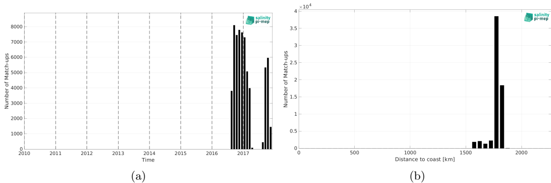
Figure 2: Number of match-ups between Seaglider (SPURS 2) and SMOS SSS L4 v2 - Daily (BEC) SSS as a function of time (a) and as function of the distance to coast (b) over the SPURS 2 Pi-MEP region and for the full satellite product period.
