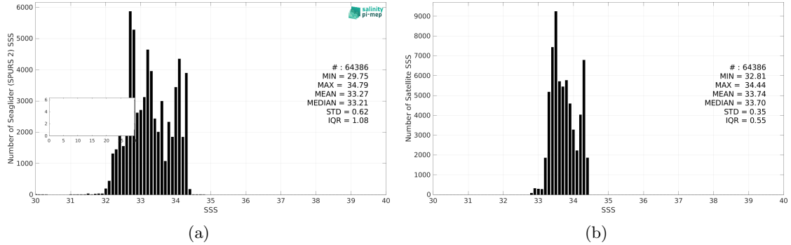
Figure 3: Histograms of SSS from Seagliders (SPURS 2) (a) and SMOS SSS L4 v2 - Daily (BEC) (b) considering all match-up pairs per bins of 0.1 over the SPURS 2 Pi-MEP region and for the full satellite product period.
