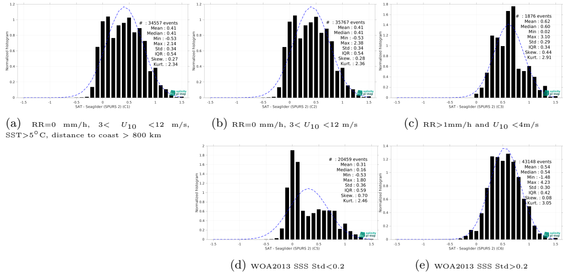
Figure 15: Normalized histogram of \Delta\text{SSS} (SMOS SSS L4 v2 - Daily (BEC) - Seaglider (SPURS 2)) for 5 different subdatasets corresponding to: RR=0 mm/h, 3 < U_{10} < 12 m/s, SST>5°C, distance to coast > 800 km (a), RR=0 mm/h, 3 < U_{10} < 12 m/s (b), RR>1mm/h and U_{10} < 4 m/s (c), WOA2013 SSS Std<0.2 (d), WOA2013 SSS Std>0.2 (e).
