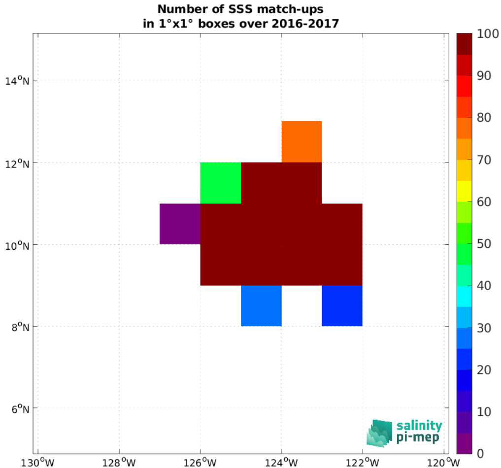
Figure 5: Number of SSS match-ups between Seaglider (SPURS 2) SSS and the SMOS SSS L4 v2 - Daily (BEC) SSS product for the SPURS 2 Pi-MEP region over 1^\circ \times 1^\circ boxes and for the full satellite product period.
