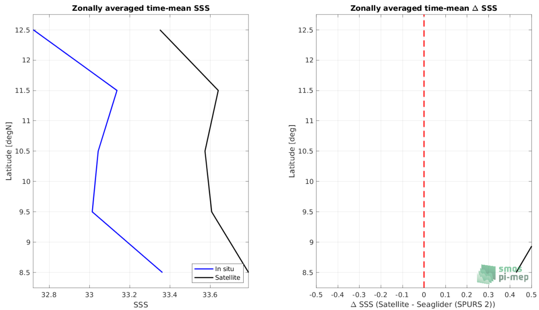
Figure 8: Left panel: Zonal mean SSS from SMOS SSS L4 v2 - Daily (BEC) satellite product (black) and from Seaglider (SPURS 2) (blue). Right panel: Zonal mean of \Delta SSS (Satellite - Seaglider (SPURS 2)) for all the collected Pi-MEP match-up pairs estimated over the full satellite product period.
