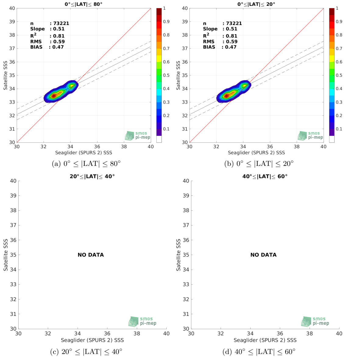
Figure 9: Contour maps of the concentration of SMOS SSS L4 v2 - Daily (BEC) SSS (y-axis) versus Seaglider (SPURS 2) SSS (x-axis) at match-up pairs for different latitude bands. For each plot, the red line shows x=y . The black thin and dashed lines indicate a linear fit through the data cloud and the \pm 95\% confidence levels, respectively. The number match-up pairs n , the slope and R^2 coefficient of the linear fit, the root mean square (RMS) and the mean bias between satellite and in situ data are indicated for each latitude band in each plots.
