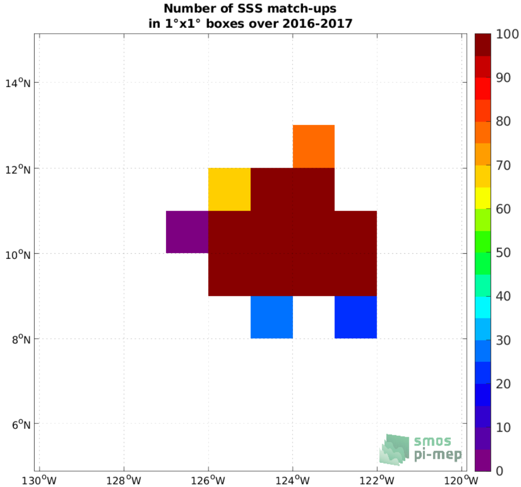
Figure 4: Number of SSS match-ups between Seaglider (SPURS 2) SSS and the SMOS SSS L4 v2 - Daily (BEC) SSS product for the SPURS 2 Pi-MEP region over 1^\circ \times 1^\circ boxes and for the full satellite product period.
