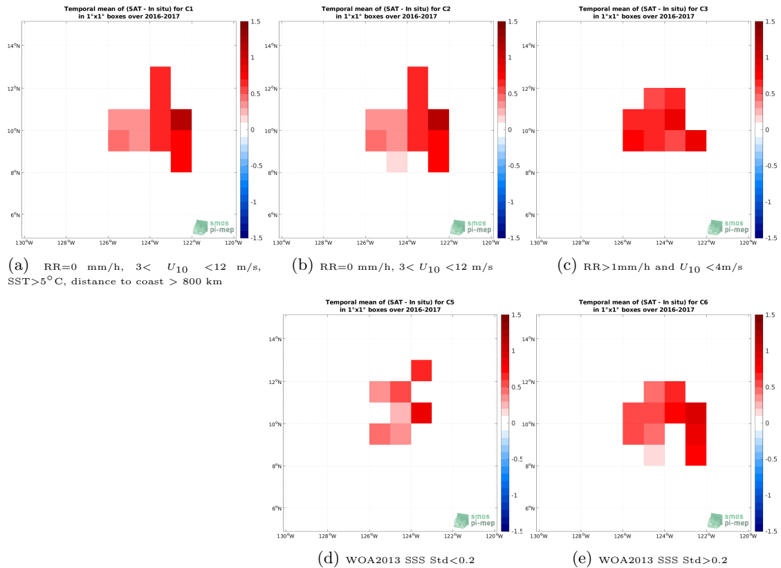
Figure 12: Temporal mean gridded over spatial boxes of size 1^\circ \times 1^\circ of \Delta SSS (SMOS SSS L4 v2 - Daily (BEC) - Seaglider (SPURS 2)) for 5 different subdatasets corresponding to:RR=0 mm/h, 3 < U_{10} < 12 m/s, SST >5^\circ C, distance to coast > 800 km (a), RR=0 mm/h, 3 < U_{10} < 12 m/s (b), RR >1 mm/h and U_{10} < 4 m/s (c), WOA2013 SSS Std <0.2 (d), WOA2013 SSS Std >0.2 (e).
