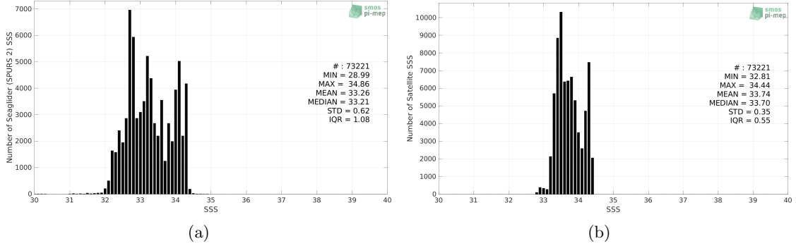
Figure 2: Histograms of SSS from Seaglider (SPURS 2) (a) and SMOS SSS L4 v2 - Daily (BEC) (b) considering all match-up pairs per bins of 0.1 over the SPURS 2 Pi-MEP region and for the full satellite product period.
