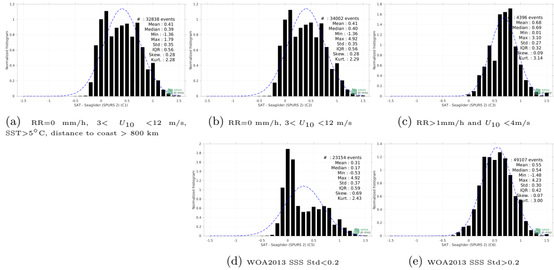
Figure 13: Normalized histogram of \Delta SSS (SMOS SSS L4 v2 - Daily (BEC) - Seaglider (SPURS 2)) for 5 different subdatasets corresponding to: RR=0 mm/h, 3 < U_{10} < 12 m/s, SST > 5°C, distance to coast > 800 km (a), RR=0 mm/h, 3 < U_{10} < 12 m/s (b), RR > 1mm/h and U_{10} < 4 m/s (c), WOA2013 SSS Std < 0.2 (d), WOA2013 SSS Std > 0.2 (e).
