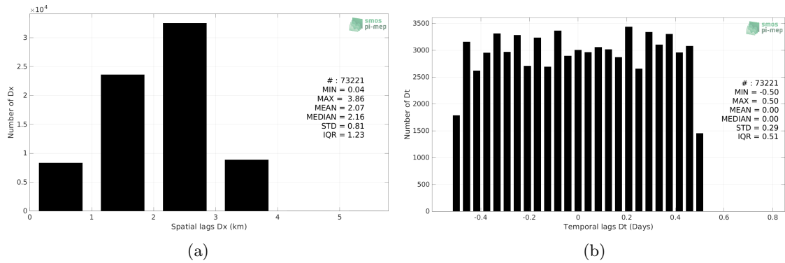
Figure 5: Histograms of the spatial (a) and temporal (b) lags between the location/time of the Seaglider (SPURS 2) measurement and the date of the corresponding SMOS SSS L4 v2 - Daily (BEC) SSS pixel.
