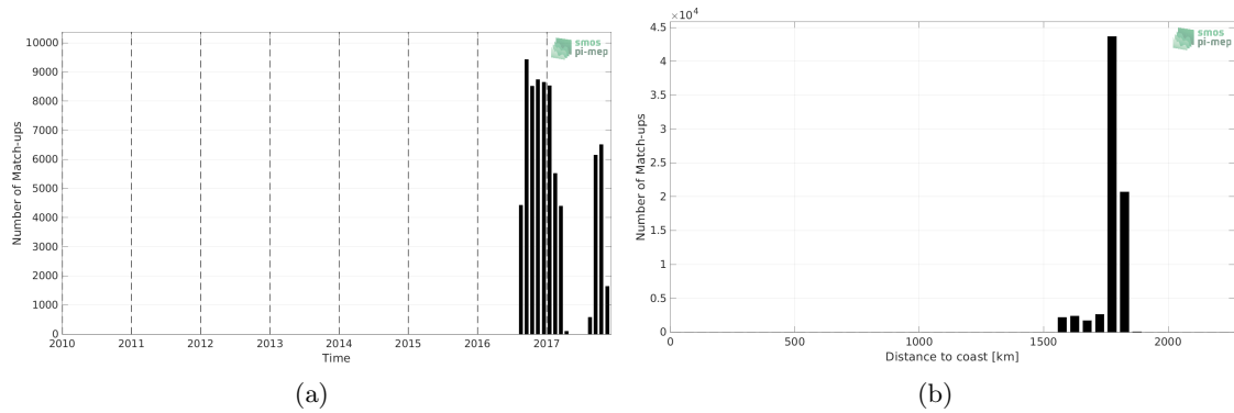
Figure 1: Number of match-ups between Seaglider (SPURS 2) and SMOS SSS L4 v2 - Daily (BEC) SSS as a function of time (a) and as function of the distance to coast (b) over the SPURS 2 Pi-MEP region and for the full satellite product period.
