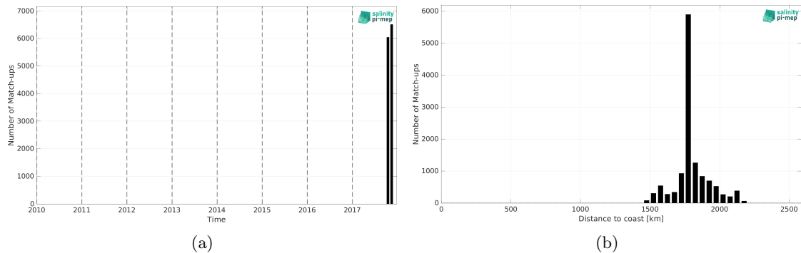
Figure 2: Number of match-ups between Saildrone and SMOS SSS L4 v2 - Daily (BEC) SSS as a function of time (a) and as function of the distance to coast (b) over the SPURS 2 Pi-MEP region and for the full satellite product period.
