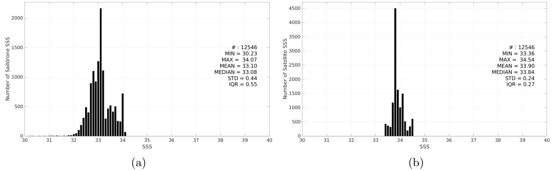
Figure 3: Histograms of SSS from Saildrone (a) and SMOS SSS L4 v2 - Daily (BEC) (b) considering all match-up pairs per bins of 0.1 over the SPURS 2 Pi-MEP region and for the full satellite product period.
