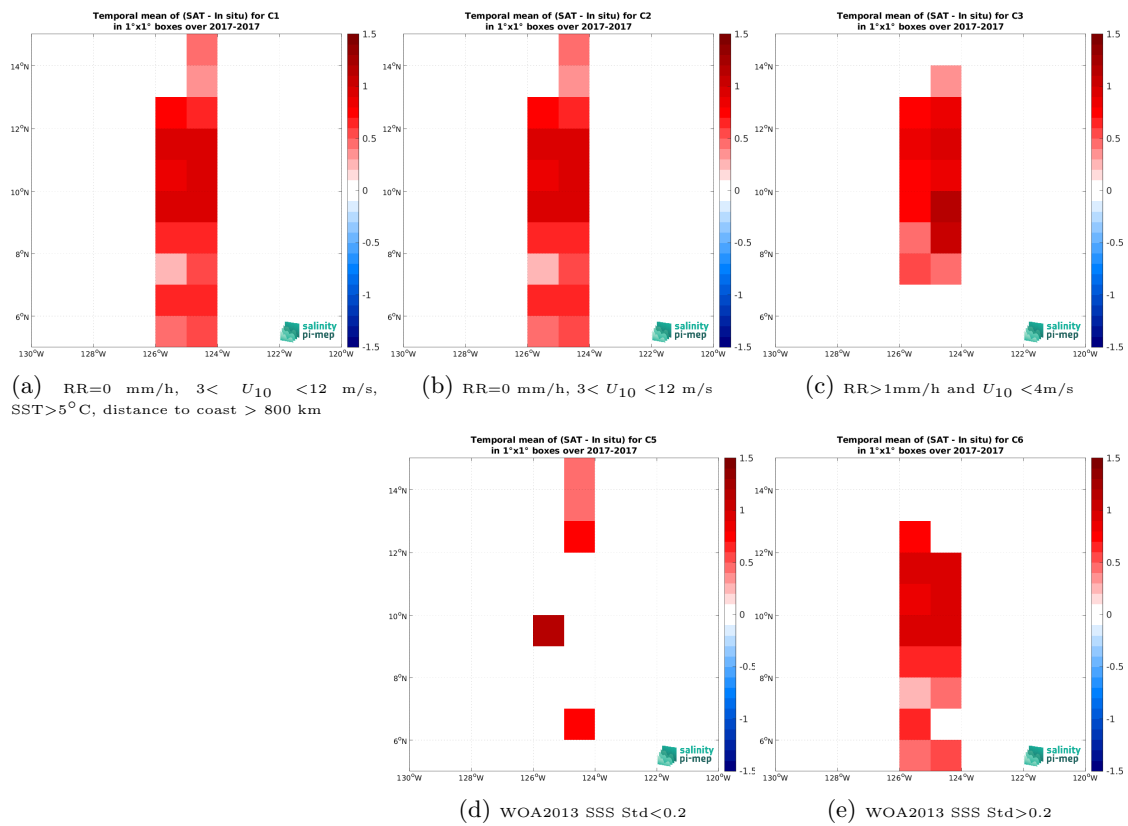
Figure 14: Temporal mean gridded over spatial boxes of size 1^\circ \times 1^\circ of \Delta SSS (SMOS SSS L4 v2 - Daily (BEC) - Sairdrone) for 5 different subdatasets corresponding to:RR=0 mm/h, 3 < U_{10} < 12 m/s, SST >5^\circ\text{C} , distance to coast > 800 km (a), RR=0 mm/h, 3 < U_{10} < 12 m/s (b), RR >1 mm/h and U_{10} < 4 m/s (c), WOA2013 SSS Std <0.2 (d), WOA2013 SSS Std >0.2 (e).
