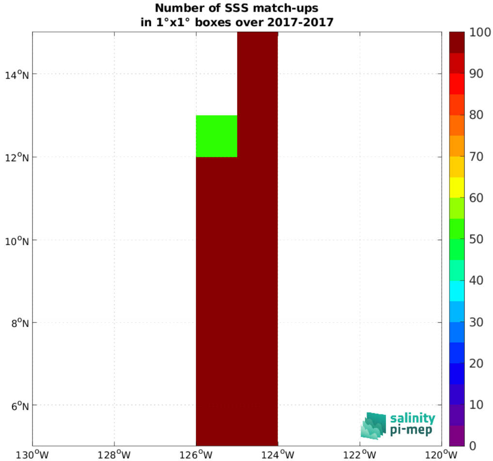
Figure 5: Number of SSS match-ups between Saildrone SSS and the SMOS SSS L4 v2 - Daily (BEC) SSS product for the SPURS 2 Pi-MEP region over 1^\circ \times 1^\circ boxes and for the full satellite product period.
