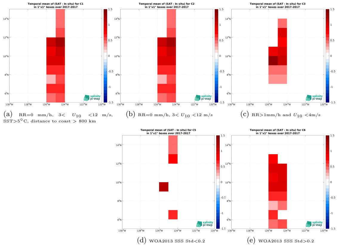
Figure 12: Temporal mean gridded over spatial boxes of size 1^\circ \times 1^\circ of \Delta SSS (SMOS SSS L4 v2 - Daily (BEC) - Sairdrone) for 5 different subdatasets corresponding to:RR=0 mm/h, 3 < U_{10} < 12 m/s, SST >5^\circ\text{C} , distance to coast > 800 km (a), RR=0 mm/h, 3 < U_{10} < 12 m/s (b), RR >1 mm/h and U_{10} < 4 m/s (c), WOA2013 SSS Std <0.2 (d), WOA2013 SSS Std >0.2 (e).
