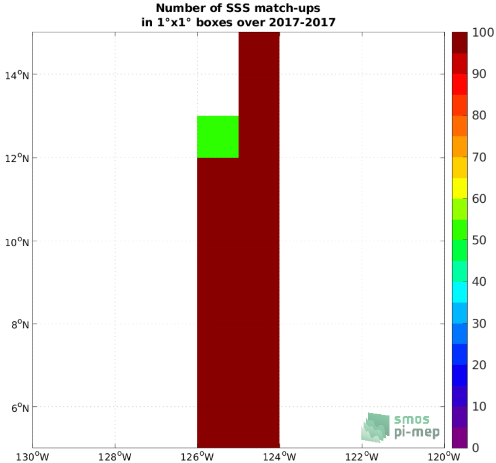
Figure 4: Number of SSS match-ups between Saildrone SSS and the SMOS SSS L4 v2 - Daily (BEC) SSS product for the SPURS 2 Pi-MEP region over 1^\circ \times 1^\circ boxes and for the full satellite product period.
