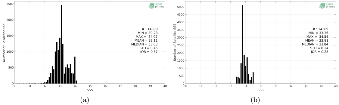
Figure 2: Histograms of SSS from Saildrone (a) and SMOS SSS L4 v2 - Daily (BEC) (b) considering all match-up pairs per bins of 0.1 over the SPURS 2 Pi-MEP region and for the full satellite product period.
