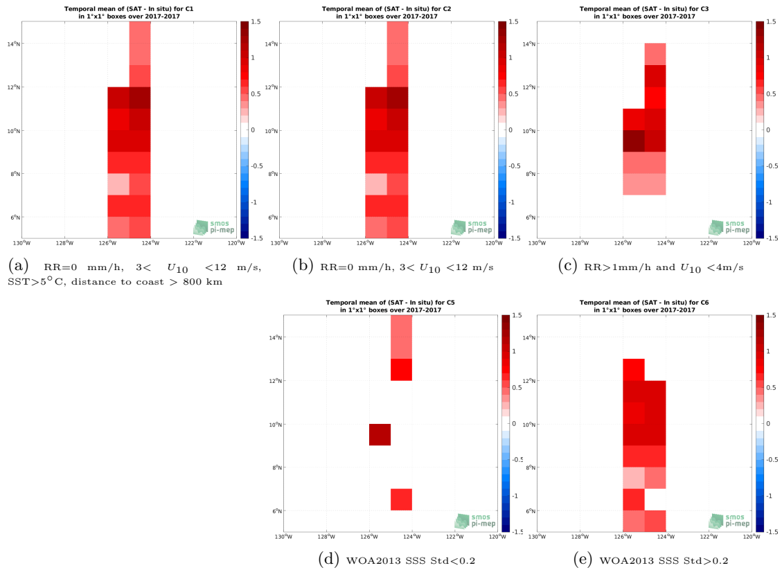
Figure 12: Temporal mean gridded over spatial boxes of size 1^\circ \times 1^\circ of \Delta\text{SSS} (SMOS SSS L4 v2 - Daily (BEC) - Sairdrone) for 5 different subdatasets corresponding to:RR=0 mm/h, 3 < U_{10} < 12 m/s, SST >5^\circ\text{C} , distance to coast > 800 km (a), RR=0 mm/h, 3 < U_{10} < 12 m/s (b), RR >1 mm/h and U_{10} < 4 m/s (c), WOA2013 SSS Std <0.2 (d), WOA2013 SSS Std >0.2 (e).
