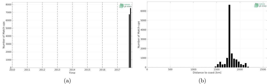
Figure 1: Number of match-ups between Saildrone and SMOS SSS L4 v2 - Daily (BEC) SSS as a function of time (a) and as function of the distance to coast (b) over the SPURS 2 Pi-MEP region and for the full satellite product period.
