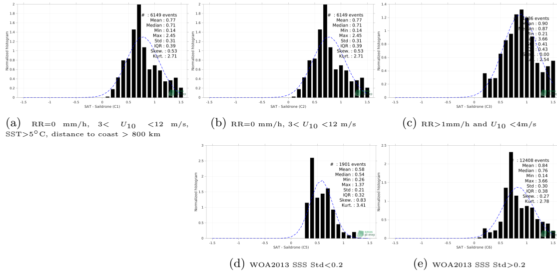
Figure 13: Normalized histogram of \Delta SSS (SMOS SSS L4 v2 - Daily (BEC) - Saildrone) for 5 different subdatasets corresponding to: RR=0 mm/h, 3 < U_{10} < 12 m/s, SST>5°C, distance to coast > 800 km (a), RR=0 mm/h, 3 < U_{10} < 12 m/s (b), RR>1mm/h and U_{10} < 4 m/s (c), WOA2013 SSS Std<0.2 (d), WOA2013 SSS Std>0.2 (e).
