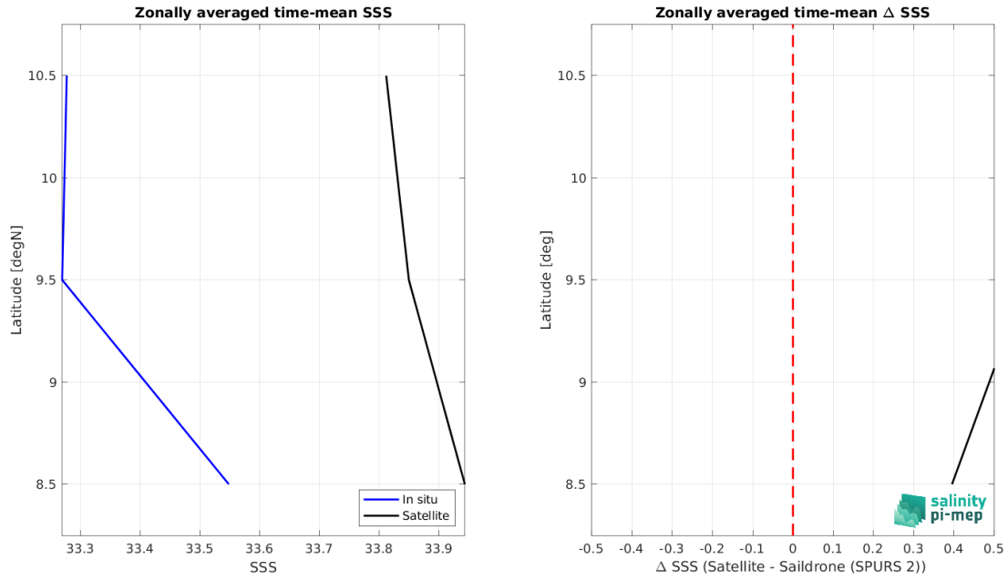
Figure 9: Left panel: Zonal mean SSS from SMOS SSS L4 v2 - Daily (BEC) satellite product (black) and from Sairdrone (SPURS 2) (blue). Right panel: Zonal mean of \Delta SSS (Satellite - Sairdrone (SPURS 2)) for all the collected Pi-MEP match-up pairs estimated over the full satellite product period.
