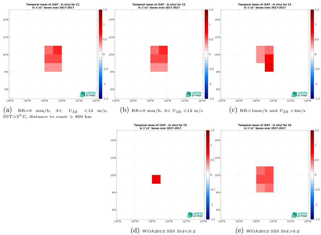
Figure 14: Temporal mean gridded over spatial boxes of size 1^\circ \times 1^\circ of \Delta SSS (SMOS SSS L4 v2 - Daily (BEC) - Sailability (SPURS 2)) for 5 different subdatasets corresponding to: RR=0 mm/h, 3 < U_{10} < 12 m/s, SST > 5^\circ\text{C} , distance to coast > 800 km (a), RR=0 mm/h, 3 < U_{10} < 12 m/s (b), RR > 1 mm/h and U_{10} < 4 m/s (c), WOA2013 SSS Std < 0.2 (d), WOA2013 SSS Std > 0.2 (e).
