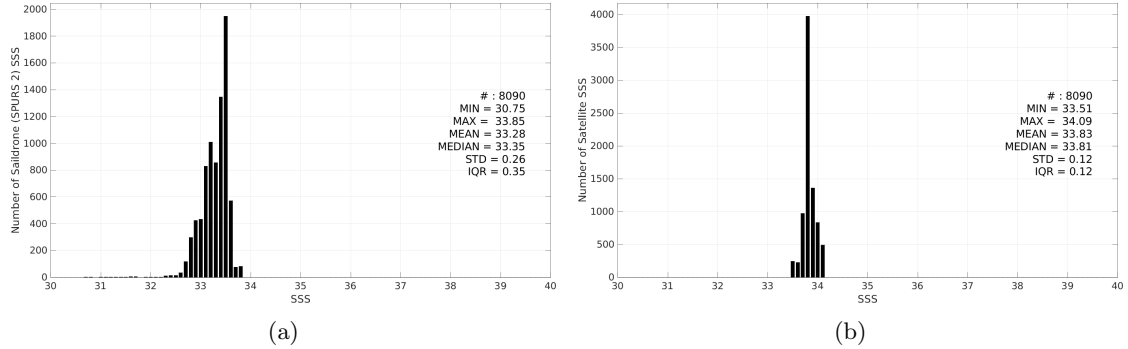
Figure 3: Histograms of SSS from Saildrone (SPURS 2) (a) and SMOS SSS L4 v2 - Daily (BEC) (b) considering all match-up pairs per bins of 0.1 over the SPURS 2 Pi-MEP region and for the full satellite product period.
