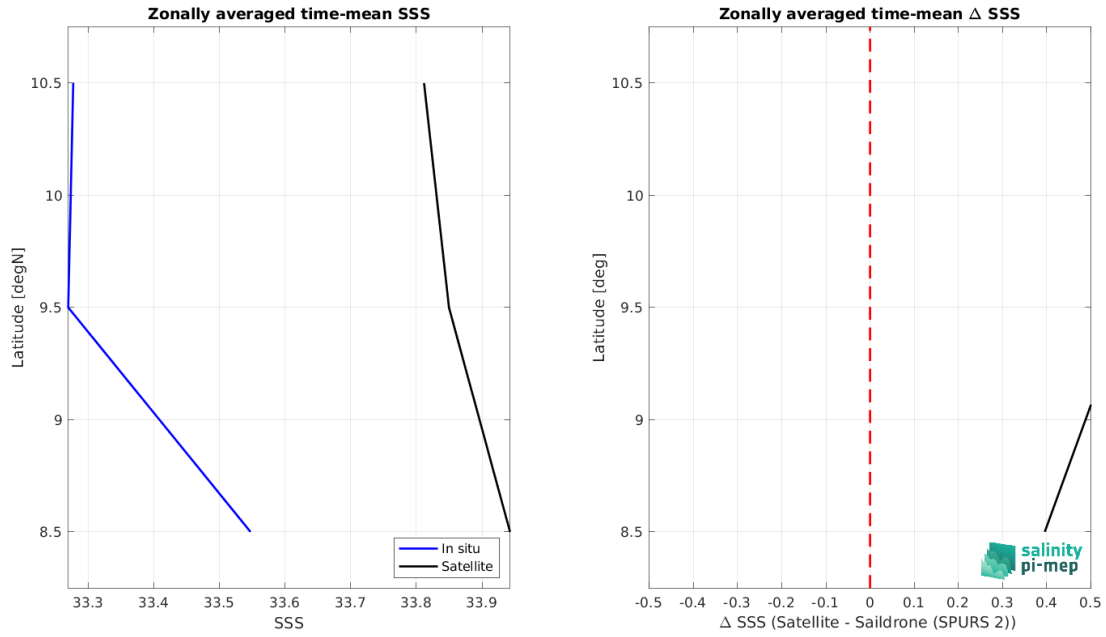
Figure 9: Left panel: Zonal mean SSS from SMOS SSS L4 v2 - Daily (BEC) satellite product (black) and from Sairdron (SPURS 2) (blue). Right panel: Zonal mean of \Delta SSS (Satellite - Sairdron (SPURS 2)) for all the collected Pi-MEP match-up pairs estimated over the full satellite product period.
