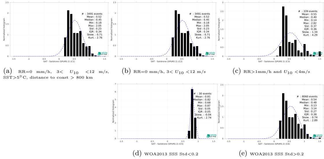
Figure 15: Normalized histogram of \Delta SSS (SMOS SSS L4 v2 - Daily (BEC) - Saildrone (SPURS 2)) for 5 different subdatasets corresponding to: RR=0 mm/h, 3 < U_{10} < 12 m/s, SST > 5°C, distance to coast > 800 km (a), RR=0 mm/h, 3 < U_{10} < 12 m/s (b), RR > 1mm/h and U_{10} < 4 m/s (c), WOA2013 SSS Std < 0.2 (d), WOA2013 SSS Std > 0.2 (e).
