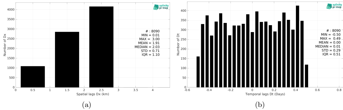
Figure 6: Histograms of the spatial (a) and temporal (b) lags between the location/time of the Sairdrone (SPURS 2) measurement and the date of the corresponding SMOS SSS L4 v2 - Daily (BEC) SSS pixel.
