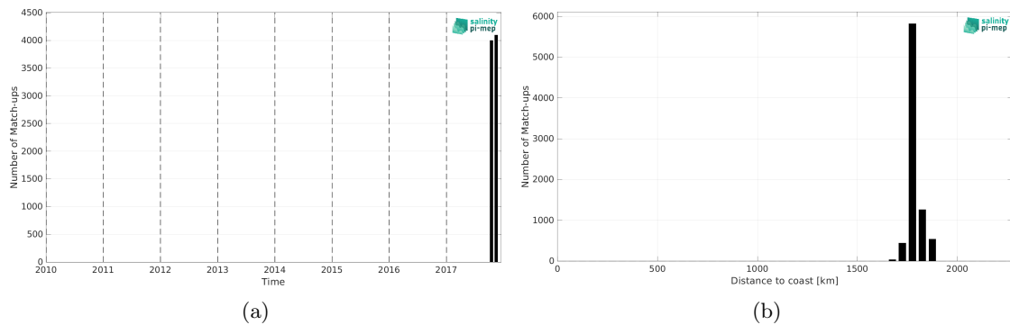
Figure 2: Number of match-ups between Saildrone (SPURS 2) and SMOS SSS L4 v2 - Daily (BEC) SSS as a function of time (a) and as function of the distance to coast (b) over the SPURS 2 Pi-MEP region and for the full satellite product period.
