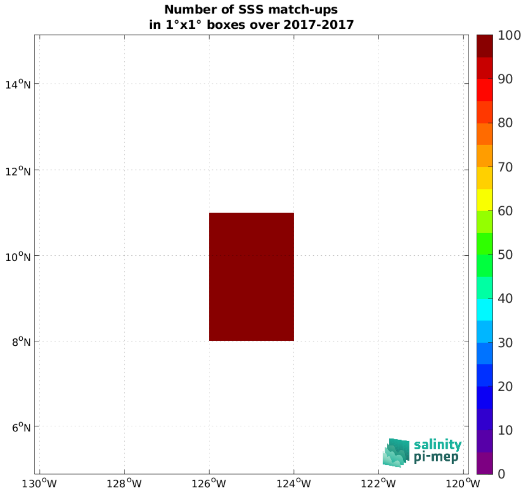
Figure 5: Number of SSS match-ups between Saildrone (SPURS 2) SSS and the SMOS SSS L4 v2 - Daily (BEC) SSS product for the SPURS 2 Pi-MEP region over 1^\circ \times 1^\circ boxes and for the full satellite product period.
