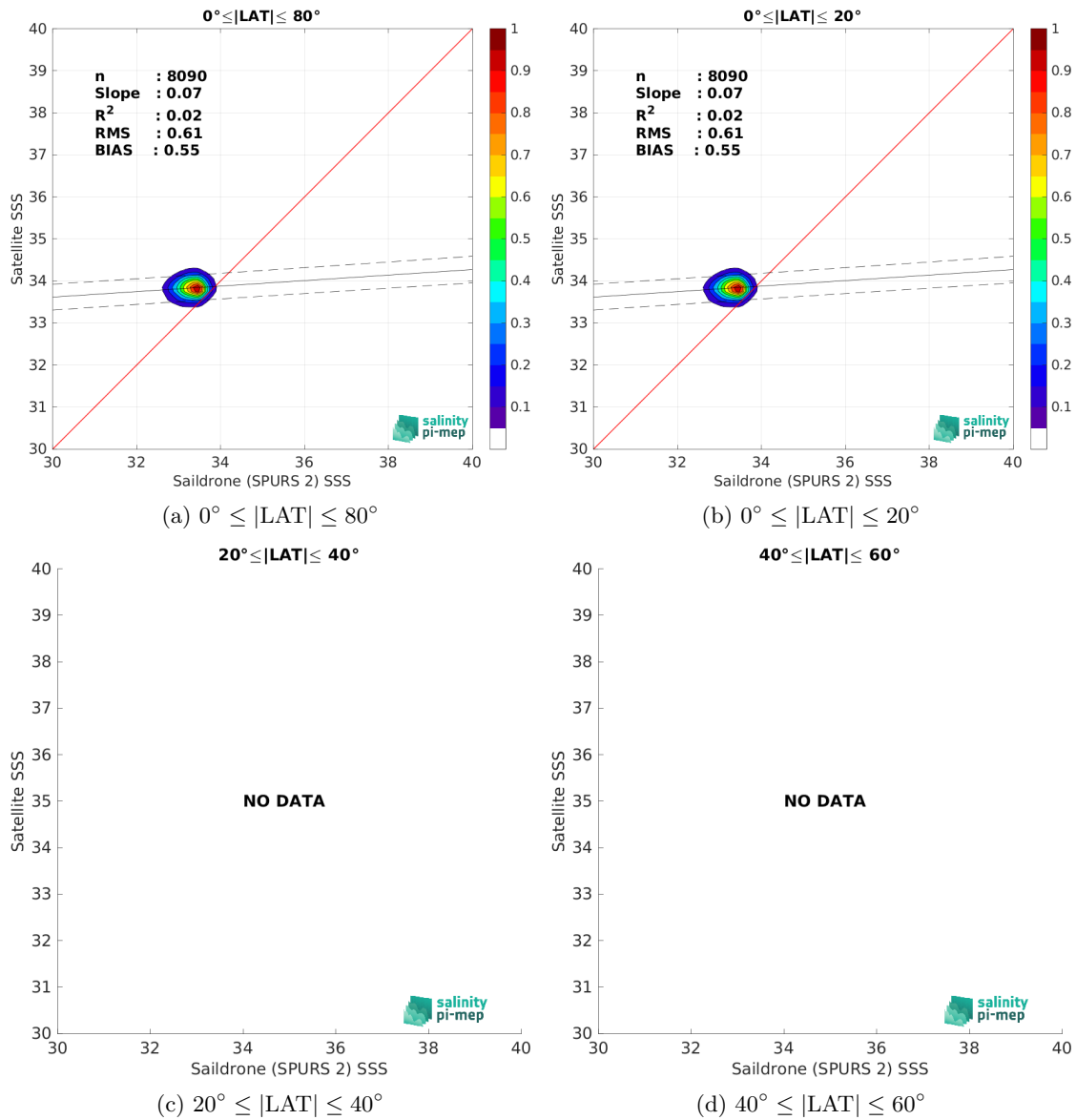
Figure 10: Contour maps of the concentration of SMOS SSS L4 v2 - Daily (BEC) SSS (y-axis) versus Saildrone (SPURS 2) SSS (x-axis) at match-up pairs for different latitude bands. For each plot, the red line shows x=y . The black thin and dashed lines indicate a linear fit through the data cloud and the \pm 95\% confidence levels, respectively. The number match-up pairs n , the slope and R^2 coefficient of the linear fit, the root mean square (RMS) and the mean bias between satellite and in situ data are indicated for each latitude band in each plots.
