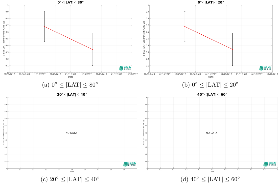
Figure 10: Monthly median (red curves) of \Delta SSS (Satellite - Sailability (SPURS 2)) and \pm 1 Std (black vertical thick bars) as function of time for all the collected Pi-MEP match-up pairs estimated over the SPURS 2 Pi-MEP region and for the full satellite product period are shown for different latitude bands: (a) 80°S-80°N, (b) 20°S-20°N, (c) 40°S-20°S and 20°N-40°N and (d) 60°S-40°S and 40°N-60°N.
