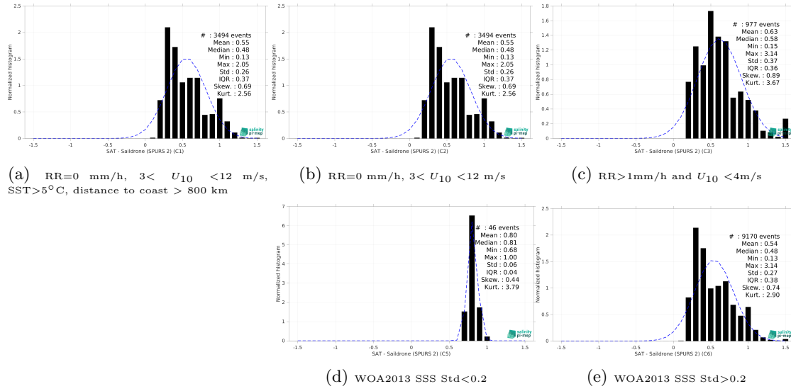
Figure 13: Normalized histogram of \Delta SSS (SMOS SSS L4 v2 - Daily (BEC) - Saildrone (SPURS 2)) for 5 different subdatasets corresponding to: RR=0 mm/h, 3 < U_{10} < 12 m/s, SST>5°C, distance to coast > 800 km (a), RR=0 mm/h, 3 < U_{10} < 12 m/s (b), RR>1mm/h and U_{10} < 4 m/s (c), WOA2013 SSS Std<0.2 (d), WOA2013 SSS Std>0.2 (e).
