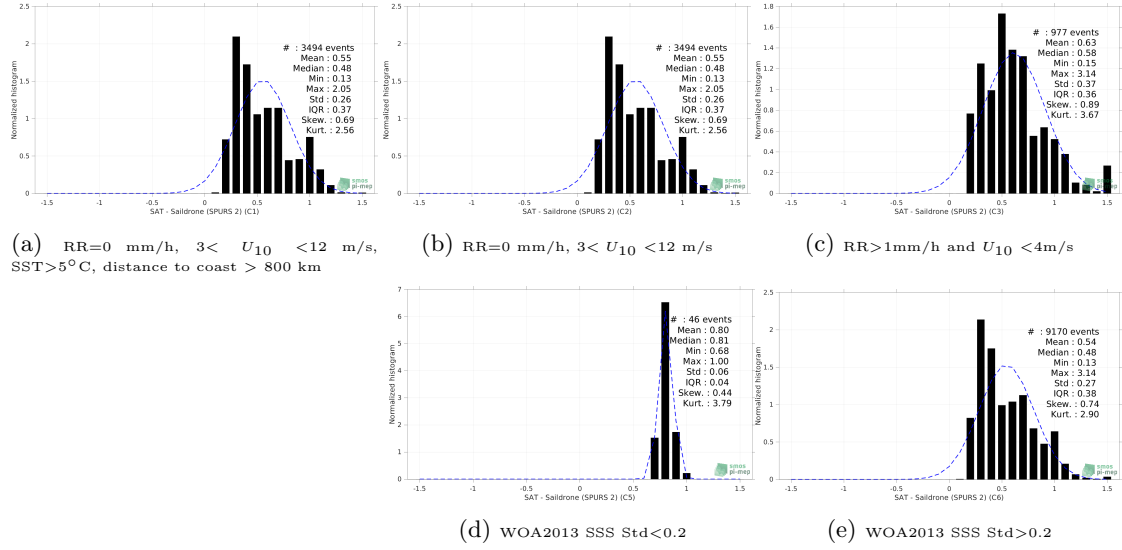
Figure 13: Normalized histogram of \Delta SSS (SMOS SSS L4 v2 - Daily (BEC) - Saildrone (SPURS 2)) for 5 different subdatasets corresponding to: RR=0 mm/h, 3 < U_{10} < 12 m/s, SST > 5°C, distance to coast > 800 km (a), RR=0 mm/h, 3 < U_{10} < 12 m/s (b), RR > 1mm/h and U_{10} < 4 m/s (c), WOA2013 SSS Std < 0.2 (d), WOA2013 SSS Std > 0.2 (e).
