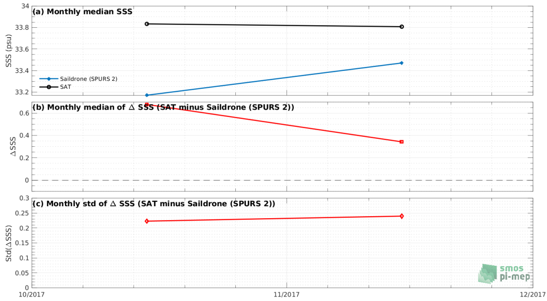
Figure 7: Time series of the monthly median SSS (top), median of \Delta SSS (Satellite - Saildrone (SPURS 2)) and Std of \Delta SSS (Satellite - Saildrone (SPURS 2)) over the SPURS 2 Pi-MEP region considering all match-ups collected by the Pi-MEP.
