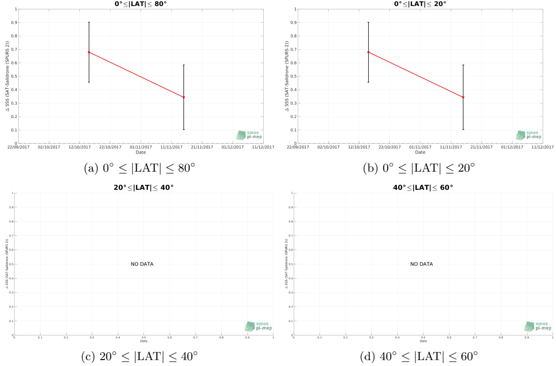
Figure 10: Monthly median (red curves) of \Delta\text{SSS} (Satellite - Saildrone (SPURS 2)) and \pm 1 Std (black vertical thick bars) as function of time for all the collected Pi-MEP match-up pairs estimated over the SPURS 2 Pi-MEP region and for the full satellite product period are shown for different latitude bands: (a) 80°S-80°N, (b) 20°S-20°N, (c) 40°S-20°S and 20°N-40°N and (d) 60°S-40°S and 40°N-60°N.
