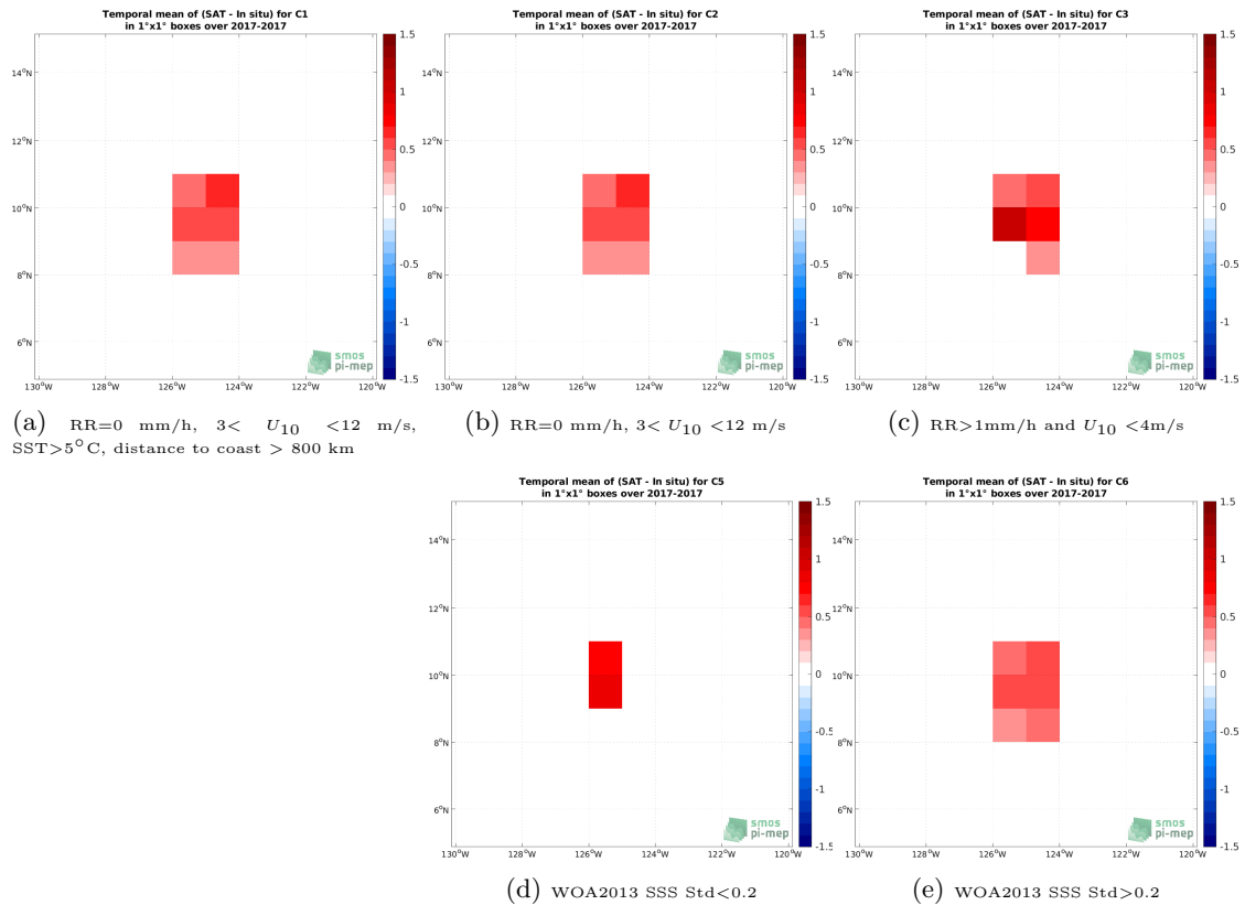
Figure 12: Temporal mean gridded over spatial boxes of size 1^\circ \times 1^\circ of \Delta SSS (SMOS SSS L4 v2 - Daily (BEC) - Sairdrone (SPURS 2)) for 5 different subdatasets corresponding to:RR=0 mm/h, 3 < U_{10} < 12 m/s, SST >5^\circ C, distance to coast > 800 km (a), RR=0 mm/h, 3 < U_{10} < 12 m/s (b), RR >1 mm/h and U_{10} < 4 m/s (c), WOA2013 SSS Std <0.2 (d), WOA2013 SSS Std >0.2 (e).
