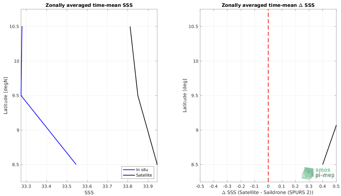
Figure 8: Left panel: Zonal mean SSS from SMOS SSS L4 v2 - Daily (BEC) satellite product (black) and from Sairdrone (SPURS 2) (blue). Right panel: Zonal mean of \Delta SSS (Satellite - Sairdrone (SPURS 2)) for all the collected Pi-MEP match-up pairs estimated over the full satellite product period.
