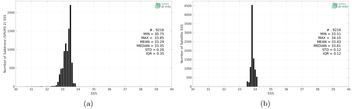
Figure 2: Histograms of SSS from Saildrone (SPURS 2) (a) and SMOS SSS L4 v2 - Daily (BEC) (b) considering all match-up pairs per bins of 0.1 over the SPURS 2 Pi-MEP region and for the full satellite product period.
