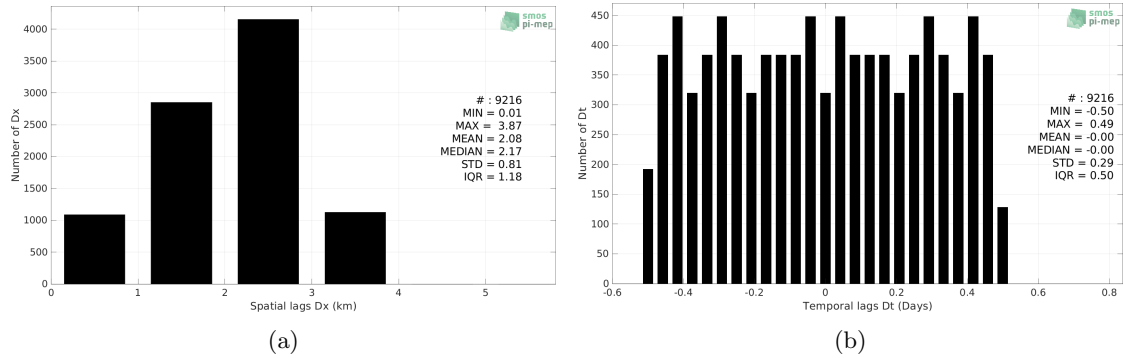
Figure 5: Histograms of the spatial (a) and temporal (b) lags between the location/time of the Sairdrone (SPURS 2) measurement and the date of the corresponding SMOS SSS L4 v2 - Daily (BEC) SSS pixel.
