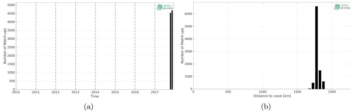
Figure 1: Number of match-ups between Saildrone (SPURS 2) and SMOS SSS L4 v2 - Daily (BEC) SSS as a function of time (a) and as function of the distance to coast (b) over the SPURS 2 Pi-MEP region and for the full satellite product period.
