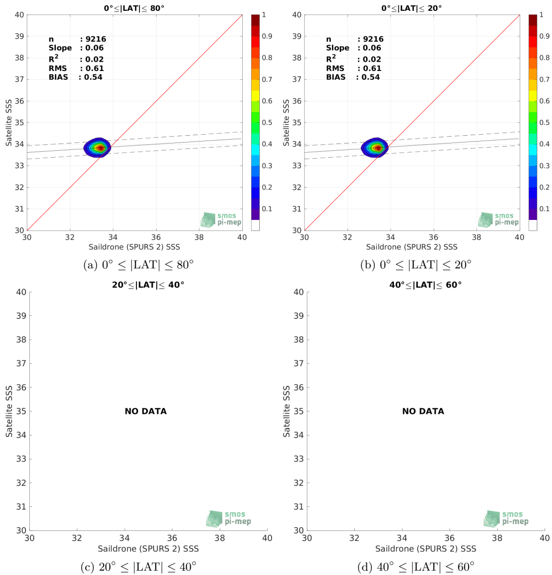
Figure 9: Contour maps of the concentration of SMOS SSS L4 v2 - Daily (BEC) SSS (y-axis) versus Saildrone (SPURS 2) SSS (x-axis) at match-up pairs for different latitude bands. For each plot, the red line shows x=y . The black thin and dashed lines indicate a linear fit through the data cloud and the \pm 95\% confidence levels, respectively. The number match-up pairs n , the slope and R^2 coefficient of the linear fit, the root mean square (RMS) and the mean bias between satellite and in situ data are indicated for each latitude band in each plots.
