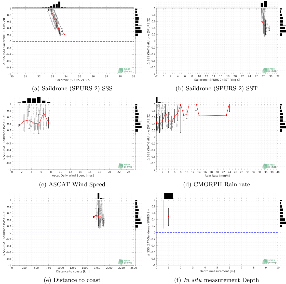
Figure 11: \Delta SSS (Satellite - Saildrone (SPURS 2)) sorted as function of Saildrone (SPURS 2) SSS values a), Saildrone (SPURS 2) SST b), ASCAT Wind speed c), CMORPH rain rate d), distance to coast (e) and in situ measurement depth (f). In all plots the median and Std of \Delta SSS for each bin is indicated by the red curves and black vertical thick bars ( \pm 1 Std)
