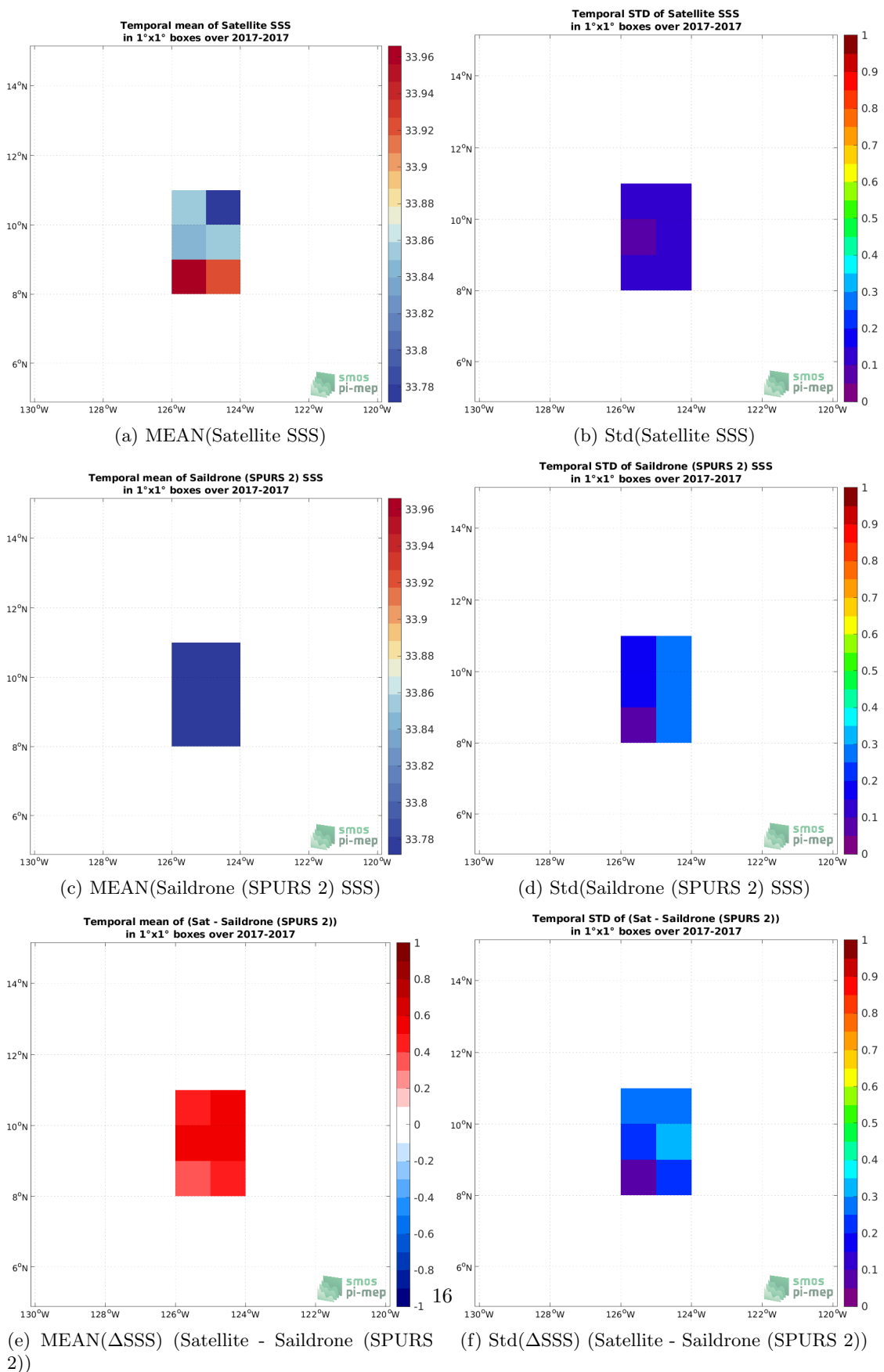
Figure 6: Temporal mean (left) and Std (right) of SSS from SMOS SSS L4 v2 - Daily (BEC) (top), Saildrone (SPURS 2) (middle), and of \Delta SSS (Satellite - Saildrone (SPURS 2)). Only match-up pairs are used to generate these maps.
