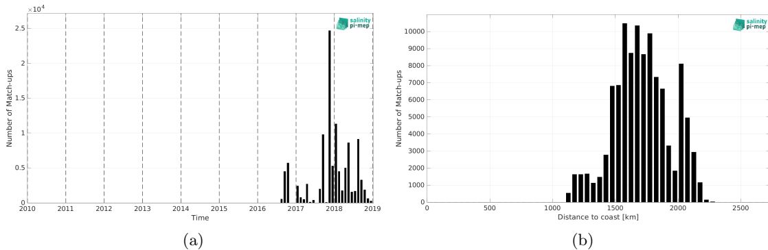
Figure 2: Number of match-ups between Surface drifters and SMOS SSS L4 v2 - Daily (BEC) SSS as a function of time (a) and as function of the distance to coast (b) over the SPURS 2 Pi-MEP region and for the full satellite product period.
