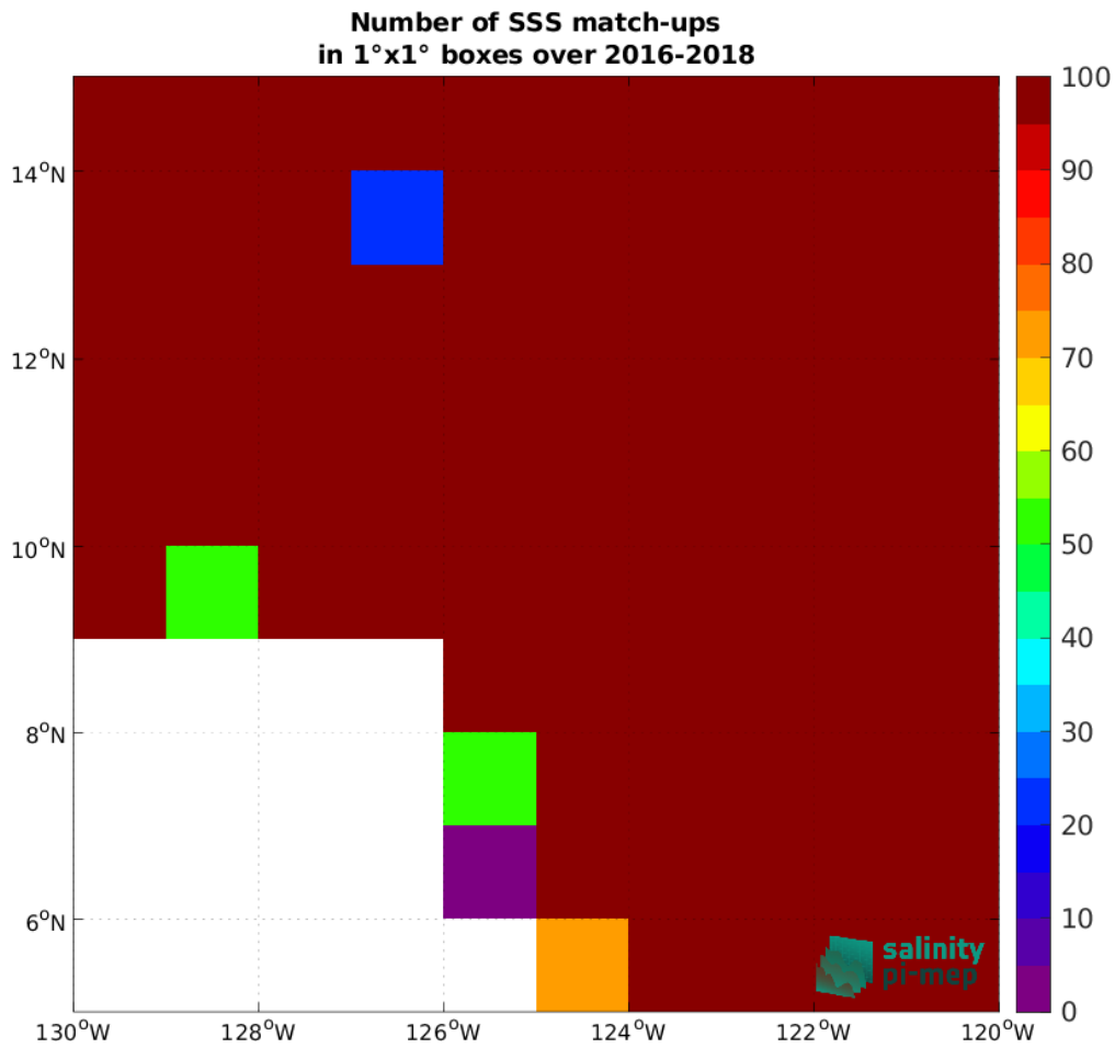
Figure 4: Number of SSS match-ups between Surface drifters SSS and the SMOS SSS L4 v2 - Daily (BEC) SSS product for the SPURS 2 Pi-MEP region over 1°x1° boxes and for the full satellite product period.
