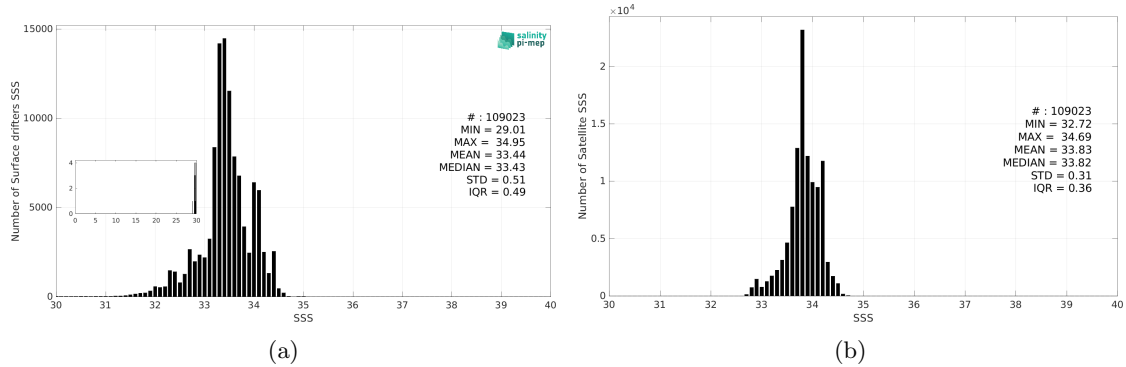
Figure 3: Histograms of SSS from Surface drifters (a) and SMOS SSS L4 v2 - Daily (BEC) (b) considering all match-up pairs per bins of 0.1 over the SPURS 2 Pi-MEP region and for the full satellite product period.
