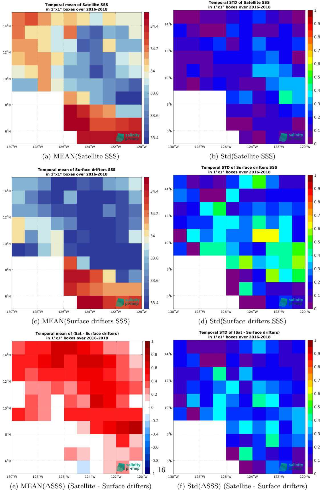
Figure 6: Temporal mean (left) and Std (right) of SSS from SMOS SSS L4 v2 - Daily (BEC) (top), Surface drifters (middle), and of \Delta SSS (Satellite - Surface drifters). Only match-up pairs are used to generate these maps.
