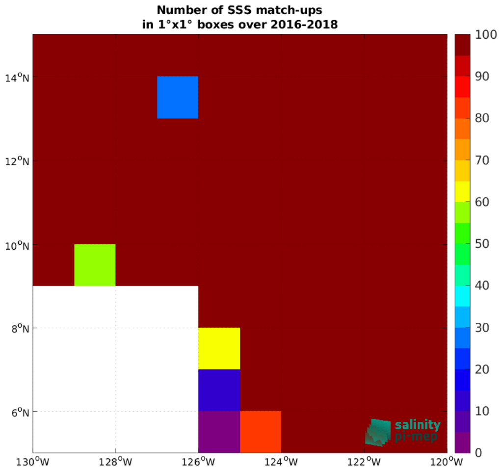
Figure 3: Number of SSS match-ups between Surface drifters SSS and the SMOS SSS L4 v2 - Daily (BEC) SSS product for the SPURS 2 Pi-MEP region over 1°x1° boxes and for the full satellite product period.
