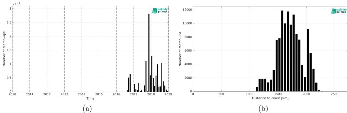
Figure 1: Number of match-ups between Surface drifters and SMOS SSS L4 v2 - Daily (BEC) SSS as a function of time (a) and as function of the distance to coast (b) over the SPURS 2 Pi-MEP region and for the full satellite product period.
