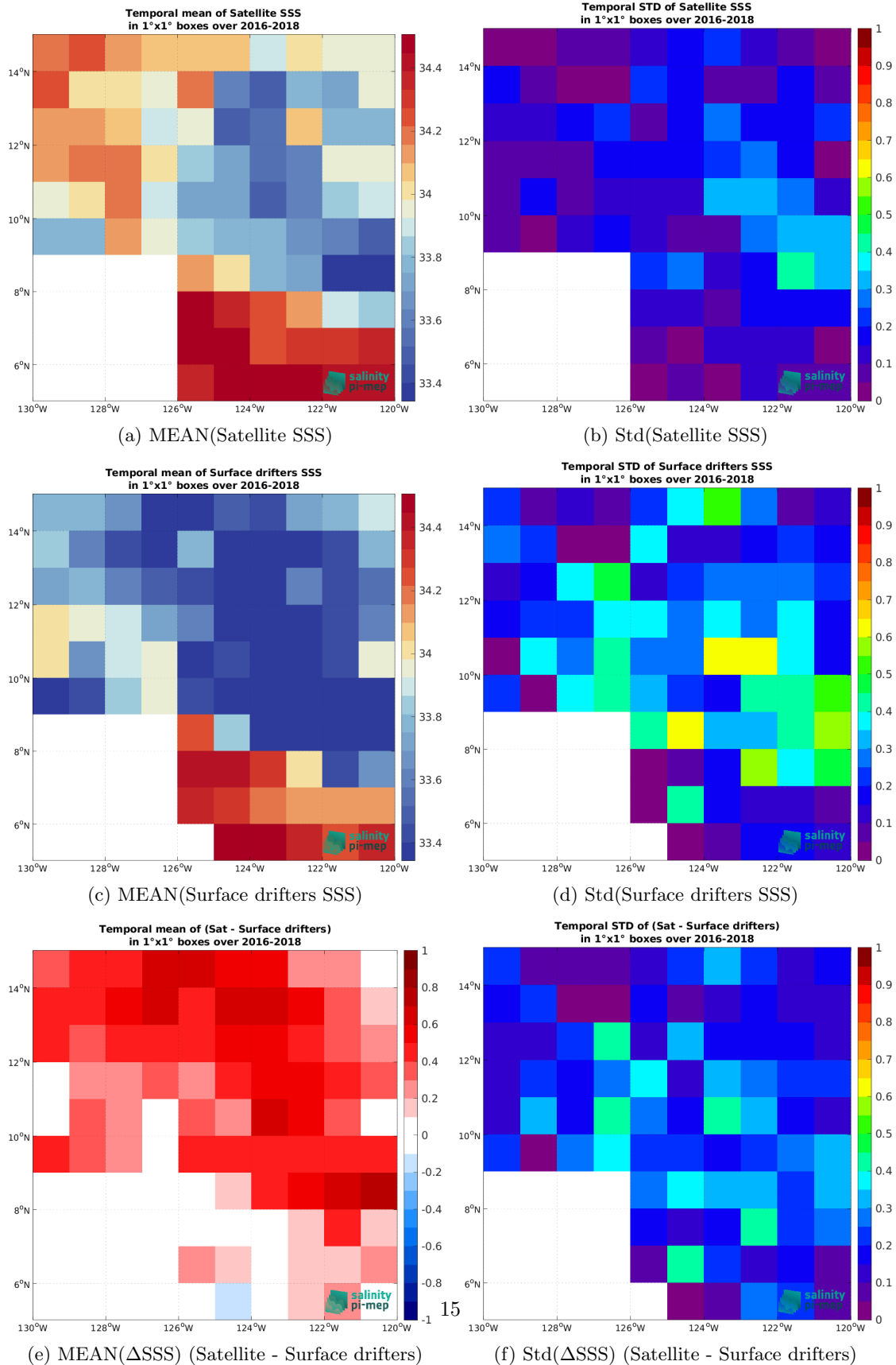
Figure 5: Temporal mean (left) and Std (right) of SSS from SMOS SSS L4 v2 - Daily (BEC) (top), Surface drifters (middle), and of \Delta SSS (Satellite - Surface drifters). Only match-up pairs are used to generate these maps.
