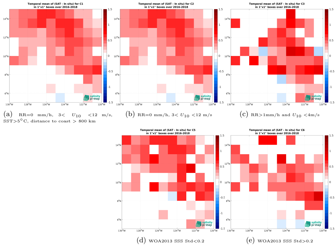
Figure 11: Temporal mean gridded over spatial boxes of size 1^\circ \times 1^\circ of \Delta\text{SSS} (SMOS SSS L4 v2 - Daily (BEC) - Surface drifters) for 5 different subdatasets corresponding to:RR=0 mm/h, 3 < U_{10} < 12 m/s, SST >5^\circ\text{C} , distance to coast > 800 km (a), RR=0 mm/h, 3 < U_{10} < 12 m/s (b), RR >1 mm/h and U_{10} < 4 m/s (c), WOA2013 SSS Std <0.2 (d), WOA2013 SSS Std >0.2 (e).
