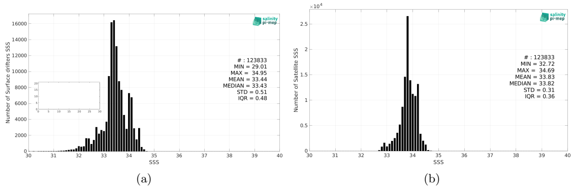
Figure 2: Histograms of SSS from Surface drifters (a) and SMOS SSS L4 v2 - Daily (BEC) (b) considering all match-up pairs per bins of 0.1 over the SPURS 2 Pi-MEP region and for the full satellite product period.
