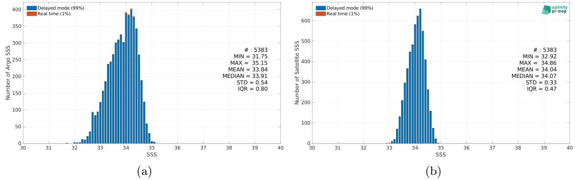
Figure 2: Histograms of SSS from Argo (a) and SMOS SSS L4 v2 - Daily (BEC) (b) considering all match-up pairs per bins of 0.1 over the SPURS 2 Pi-MEP region and for the full satellite product period.
