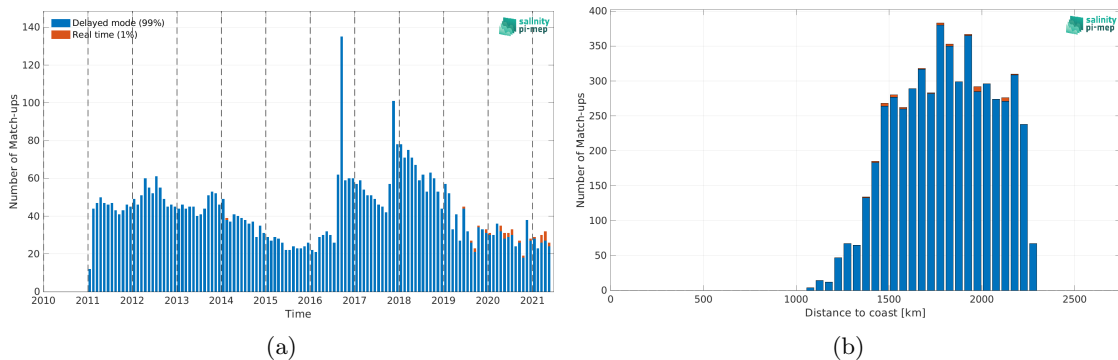
Figure 1: Number of match-ups between Argo and SMOS SSS L4 v2 - Daily (BEC) SSS as a function of time (a) and as function of the distance to coast (b) over the SPURS 2 Pi-MEP region and for the full satellite product period.
