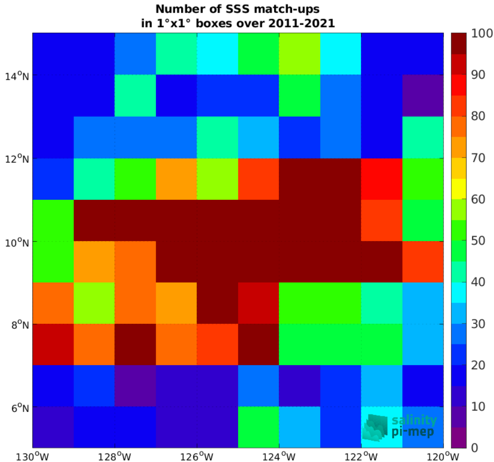
Figure 4: Number of SSS match-ups between Argo SSS and the SMOS SSS L4 v2 - Daily (BEC) SSS product for the SPURS 2 Pi-MEP region over 1^\circ \times 1^\circ boxes and for the full satellite product period.
