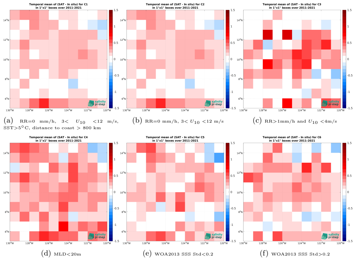
Figure 12: Temporal mean gridded over spatial boxes of size 1^\circ \times 1^\circ of \Delta SSS (SMOS SSS L4 v2 - Daily (BEC) - Argo) for 6 different subdatasets corresponding to:RR=0 mm/h, 3 < U_{10} < 12 m/s, SST >5^\circ C, distance to coast > 800 km (a), RR=0 mm/h, 3 < U_{10} < 12 m/s (b), RR >1 mm/h and U_{10} < 4 m/s (c),MLD <20 m (d),WOA2013 SSS Std <0.2 (e),WOA2013 SSS Std >0.2 (f).
