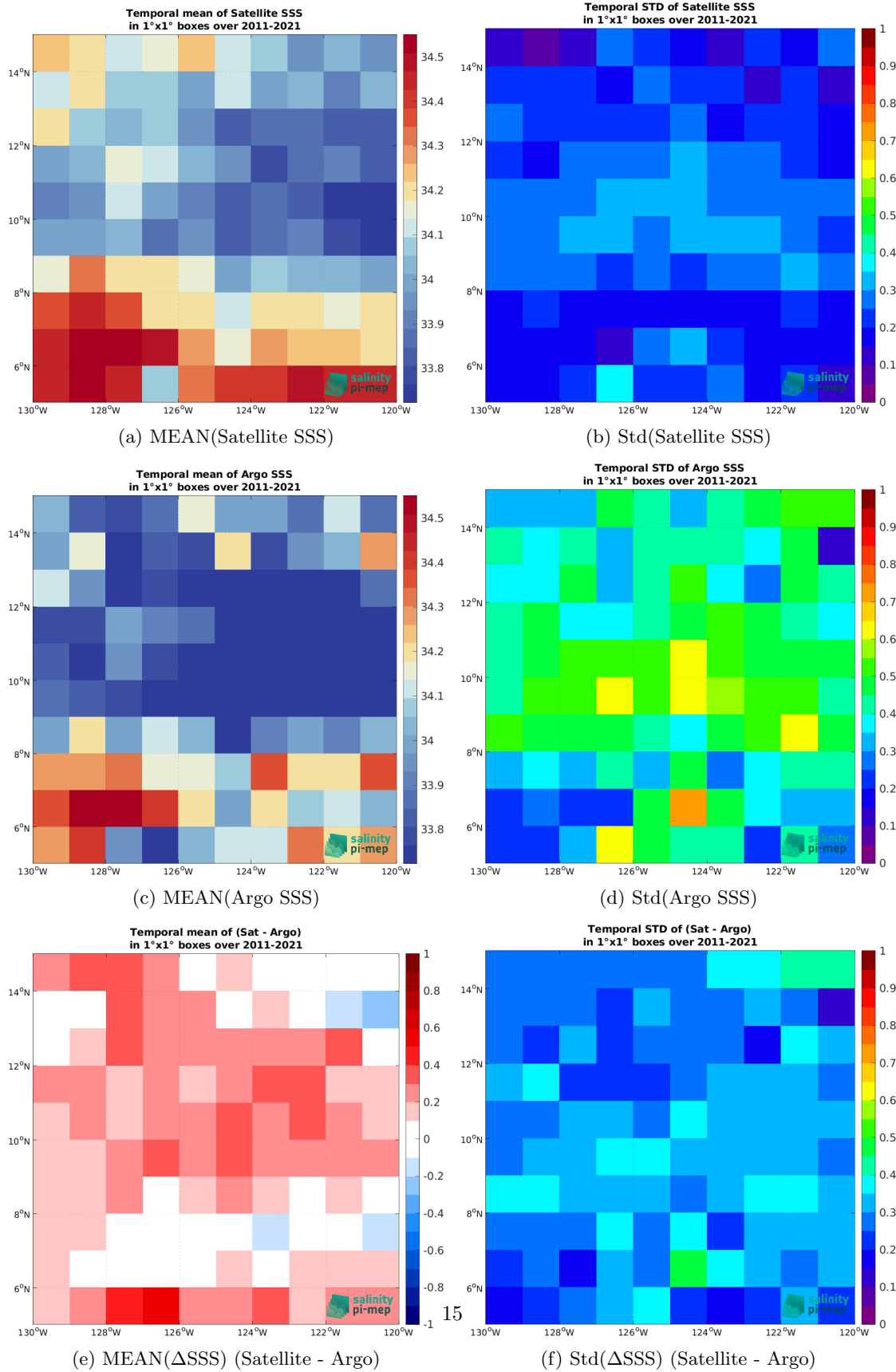
Figure 6: Temporal mean (left) and Std (right) of SSS from SMOS SSS L4 v2 - Daily (BEC) (top), Argo (middle), and of \Delta SSS (Satellite - Argo). Only match-up pairs are used to generate these maps.
