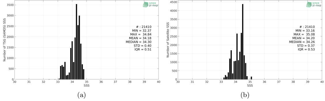
Figure 2: Histograms of SSS from TSG (SAMOS) (a) and SMOS SSS L3 v3 Monthly (ICDC) (b) considering all match-up pairs per bins of 0.1 over the SPURS 2 Pi-MEP region and for the full satellite product period.
