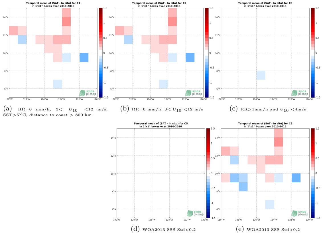
Figure 12: Temporal mean gridded over spatial boxes of size 1^\circ \times 1^\circ of \Delta SSS (SMOS SSS L3 v3 Monthly (ICDC) - TSG (SAMOS)) for 5 different subdatasets corresponding to:RR=0 mm/h, 3 < U_{10} < 12 m/s, SST >5^\circ\text{C} , distance to coast > 800 km (a), RR=0 mm/h, 3 < U_{10} < 12 m/s (b), RR >1 mm/h and U_{10} < 4 m/s (c), WOA2013 SSS Std <0.2 (d), WOA2013 SSS Std >0.2 (e).
