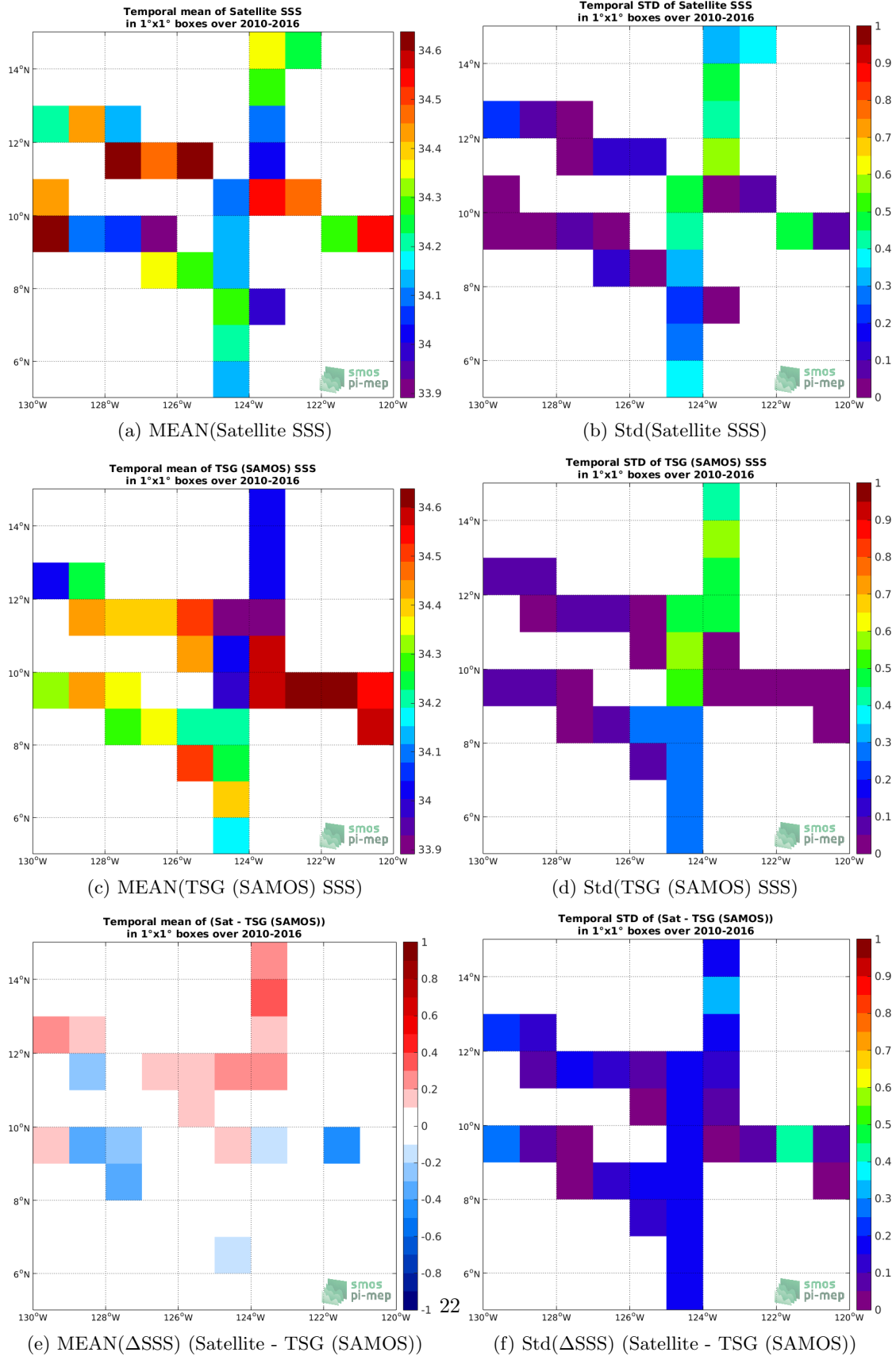
Figure 6: Temporal mean (left) and Std (right) of SSS from SMOS SSS L3 v3 Monthly (ICDC) (top), TSG (SAMOS) (middle), and of \Delta SSS (Satellite - TSG (SAMOS)). Only match-up pairs are used to generate these maps.
