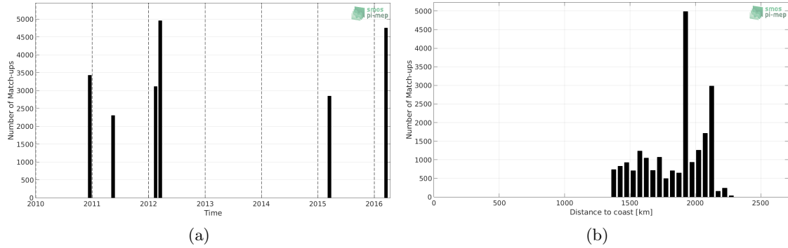
Figure 1: Number of match-ups between TSG (SAMOS) and SMOS SSS L3 v3 Monthly (ICDC) SSS as a function of time (a) and as function of the distance to coast (b) over the SPURS 2 Pi-MEP region and for the full satellite product period.
