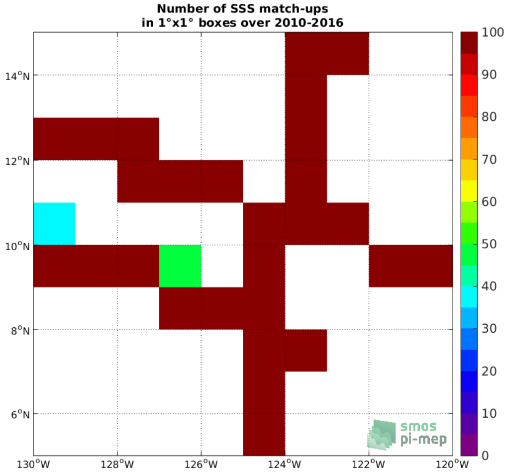
Figure 4: Number of SSS match-ups between TSG (SAMOS) SSS and the SMOS SSS L3 v3 Monthly (ICDC) SSS product for the SPURS 2 Pi-MEP region over 1°x1° boxes and for the full satellite product period.
