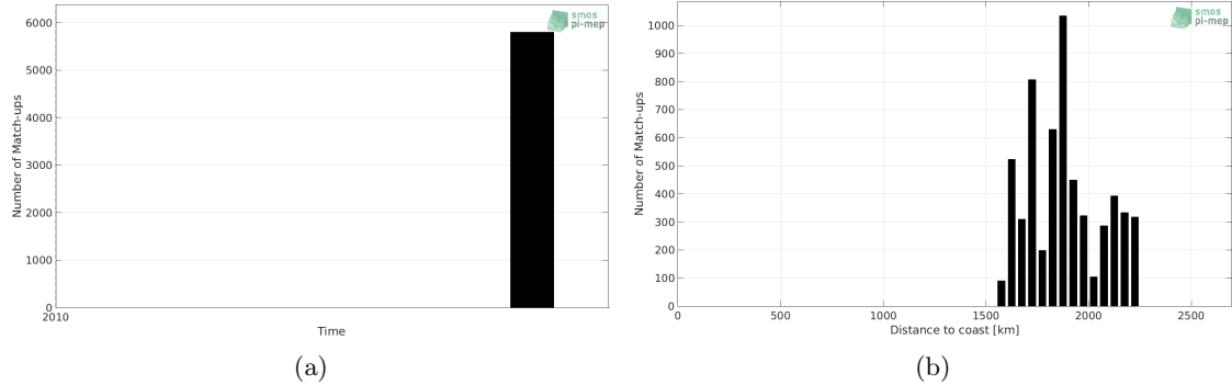
Figure 1: Number of match-ups between TSG (GOSUD-Sailing-ship) and SMOS SSS L3 v3 Monthly (ICDC) SSS as a function of time (a) and as function of the distance to coast (b) over the SPURS 2 Pi-MEP region and for the full satellite product period.
