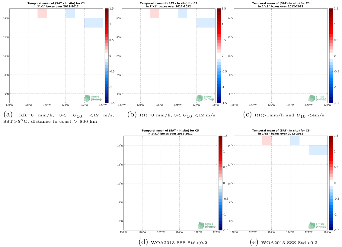
Figure 12: Temporal mean gridded over spatial boxes of size 1^\circ \times 1^\circ of \Delta SSS (SMOS SSS L3 v3 Monthly (ICDC) - TSG (GOSUD-Research-vessel)) for 5 different subdatasets corresponding to: RR=0 mm/h, 3 < U_{10} < 12 m/s, SST >5^\circ\text{C} , distance to coast > 800 km (a), RR=0 mm/h, 3 < U_{10} < 12 m/s (b), RR >1 mm/h and U_{10} < 4 m/s (c), WOA2013 SSS Std <0.2 (d), WOA2013 SSS Std >0.2 (e).
