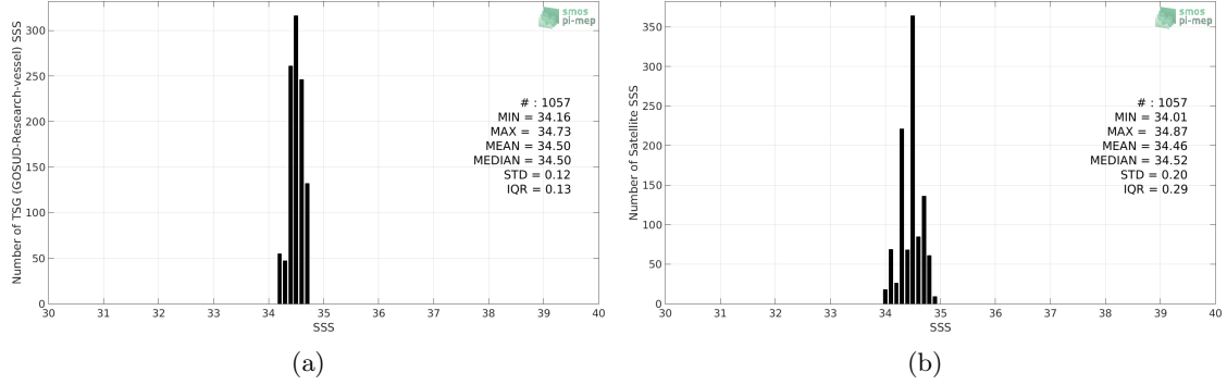
Figure 2: Histograms of SSS from TSG (GOSUD-Research-vessel) (a) and SMOS SSS L3 v3 Monthly (ICDC) (b) considering all match-up pairs per bins of 0.1 over the SPURS 2 Pi-MEP region and for the full satellite product period.
