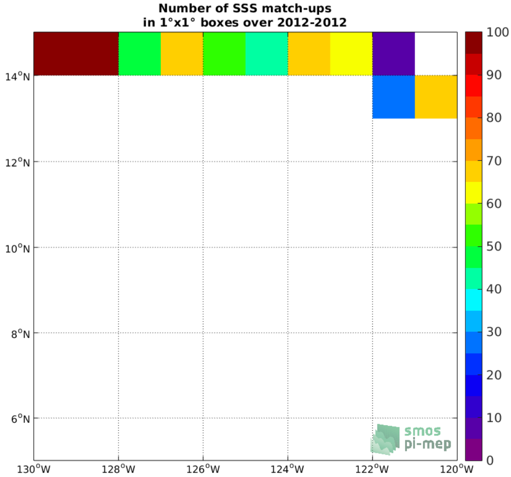
Figure 4: Number of SSS match-ups between TSG (GOSUD-Research-vessel) SSS and the SMOS SSS L3 v3 Monthly (ICDC) SSS product for the SPURS 2 Pi-MEP region over 1°x1° boxes and for the full satellite product period.
