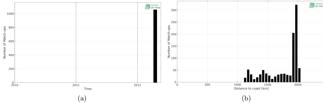
Figure 1: Number of match-ups between TSG (GOSUD-Research-vessel) and SMOS SSS L3 v3 Monthly (ICDC) SSS as a function of time (a) and as function of the distance to coast (b) over the SPURS 2 Pi-MEP region and for the full satellite product period.
