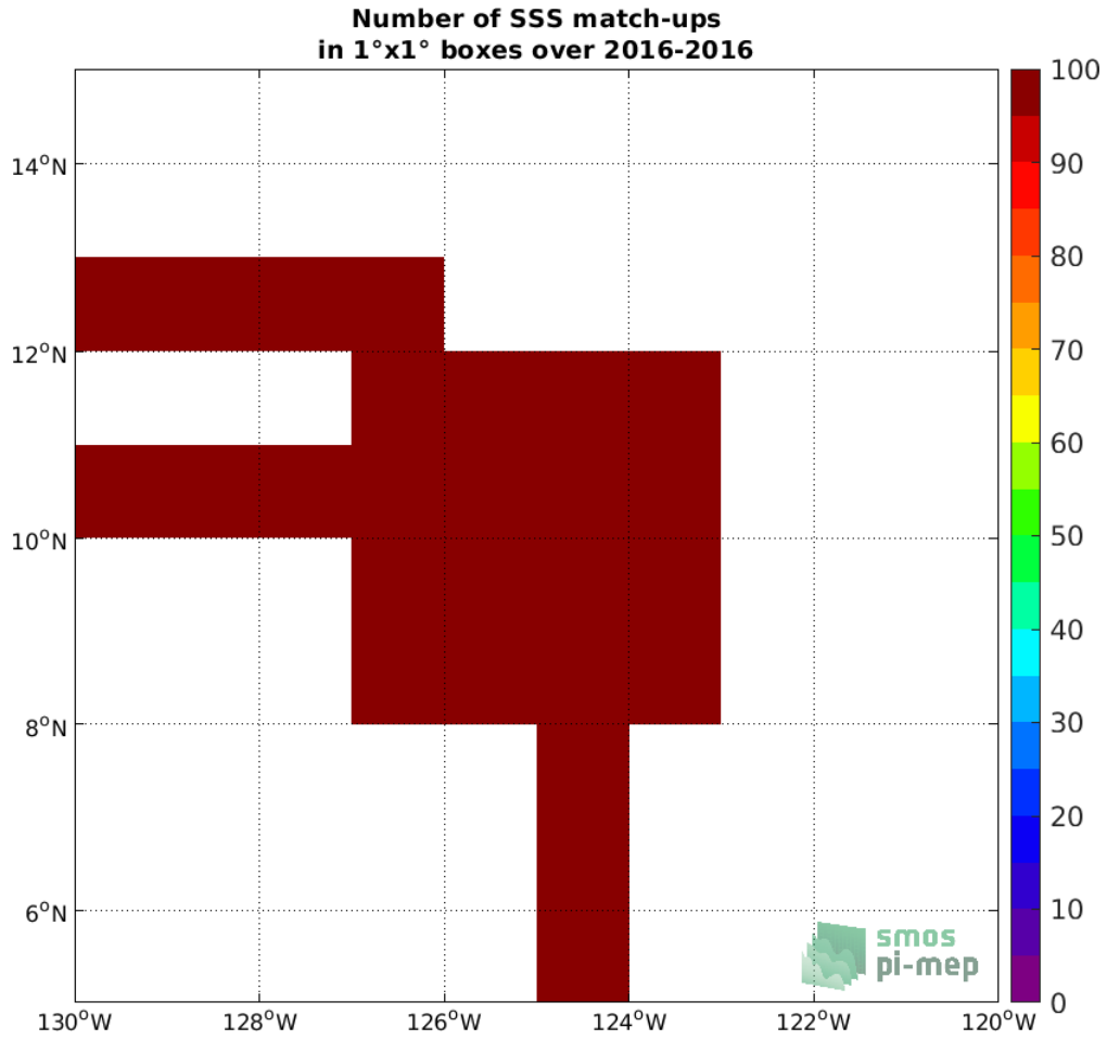
Figure 3: Number of SSS match-ups between Salinity Snake SSS and the SMOS SSS L3 v3 Monthly (ICDC) SSS product for the SPURS 2 Pi-MEP region over 1°x1° boxes and for the full satellite product period.
