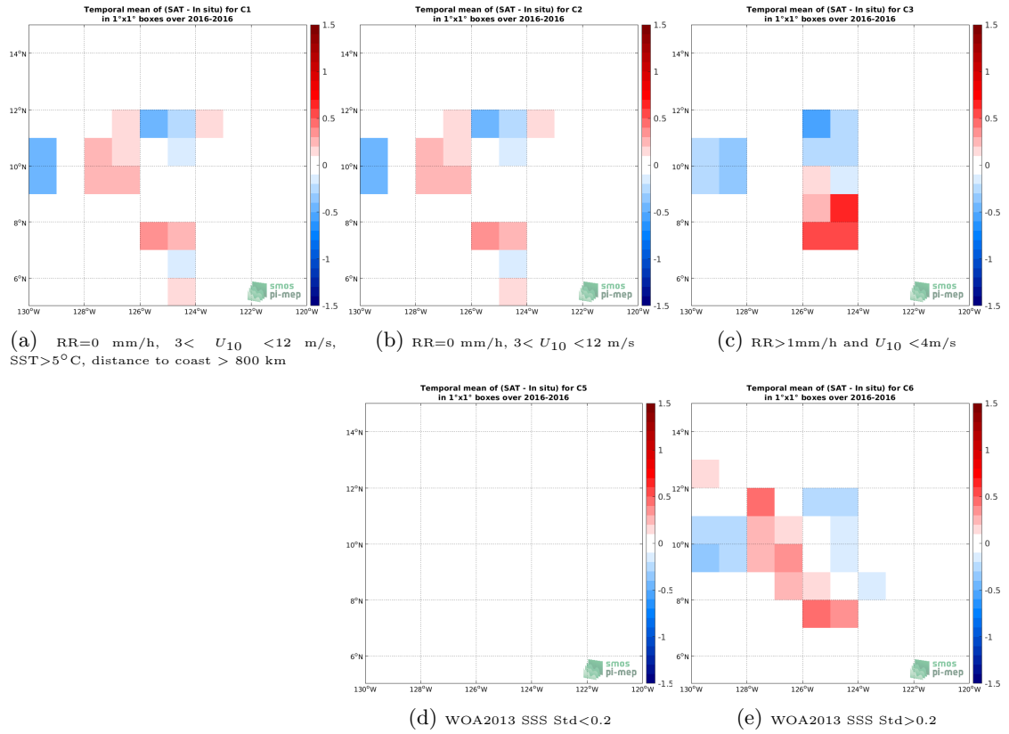
Figure 11: Temporal mean gridded over spatial boxes of size 1^\circ \times 1^\circ of \Delta SSS (SMOS SSS L3 v3 Monthly (ICDC) - Salinity Snake) for 5 different subdatasets corresponding to: RR=0 mm/h, 3 < U_{10} < 12 m/s, SST >5^\circ\text{C} , distance to coast > 800 km (a), RR=0 mm/h, 3 < U_{10} < 12 m/s (b), RR >1 mm/h and U_{10} < 4 m/s (c), WOA2013 SSS Std <0.2 (d), WOA2013 SSS Std >0.2 (e).
