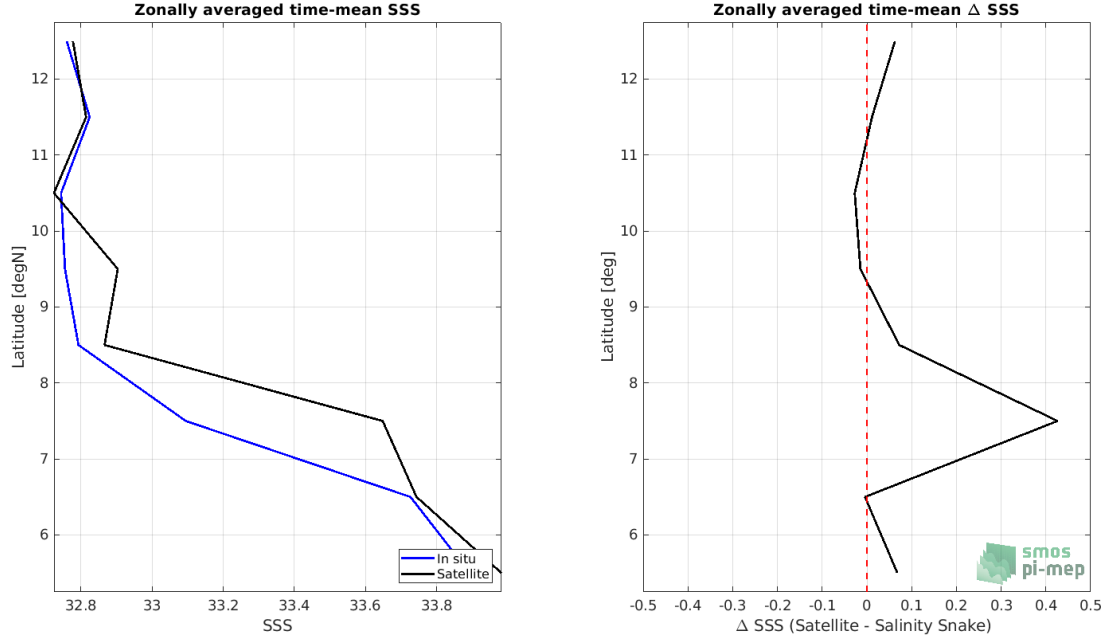
Figure 7: Left panel: Zonal mean SSS from SMOS SSS L3 v3 Monthly (ICDC) satellite product (black) and from Salinity Snake (blue). Right panel: Zonal mean of \Delta SSS (Satellite - Salinity Snake) for all the collected Pi-MEP match-up pairs estimated over the full satellite product period.
