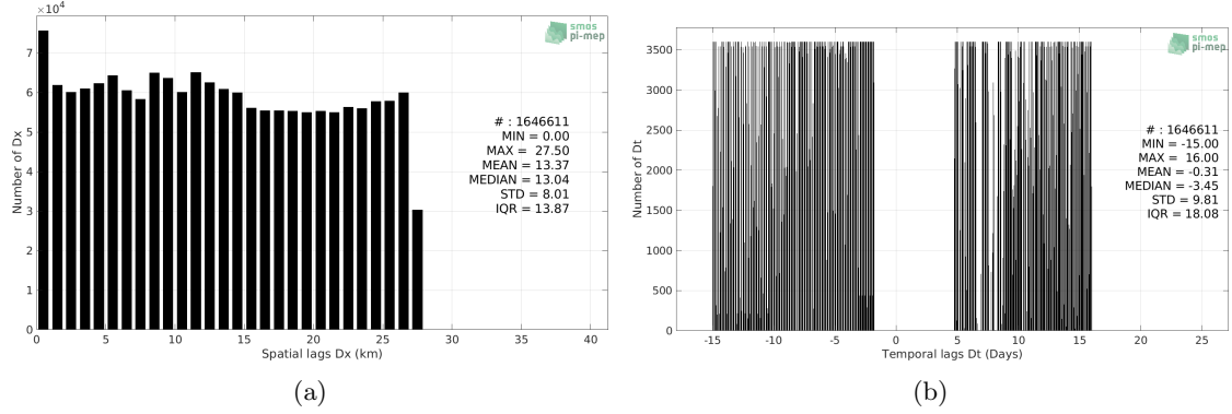
Figure 4: Histograms of the spatial (a) and temporal (b) lags between the location/time of the Salinity Snake measurement and the date of the corresponding SMOS SSS L3 v3 Monthly (ICDC) SSS pixel.
