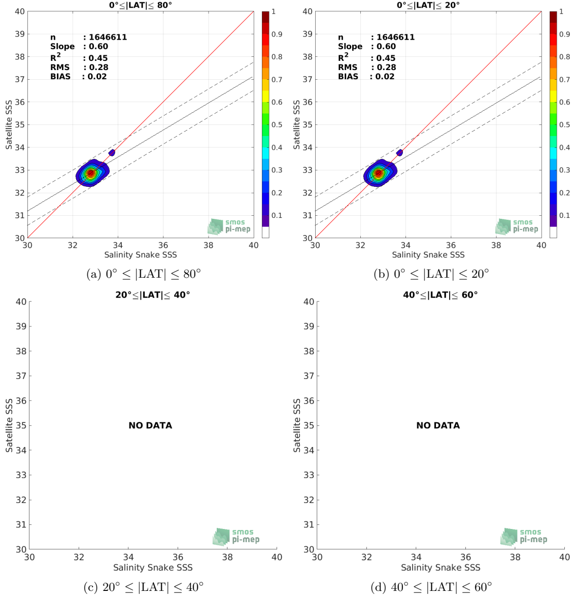
Figure 8: Contour maps of the concentration of SMOS SSS L3 v3 Monthly (ICDC) SSS (y-axis) versus Salinity Snake SSS (x-axis) at match-up pairs for different latitude bands. For each plot, the red line shows x=y . The black thin and dashed lines indicate a linear fit through the data cloud and the \pm 95\% confidence levels, respectively. The number match-up pairs n , the slope and R^2 coefficient of the linear fit, the root mean square (RMS) and the mean bias between satellite and in situ data are indicated for each latitude band in each plots.
