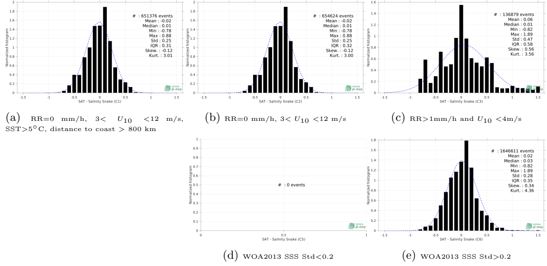
Figure 12: Normalized histogram of \Delta SSS (SMOS SSS L3 v3 Monthly (ICDC) - Salinity Snake) for 5 different subdatasets corresponding to: RR=0 mm/h, 3 < U_{10} < 12 m/s, SST>5°C, distance to coast > 800 km (a), RR=0 mm/h, 3 < U_{10} < 12 m/s (b), RR>1mm/h and U_{10} < 4 m/s (c), WOA2013 SSS Std<0.2 (d), WOA2013 SSS Std>0.2 (e).
