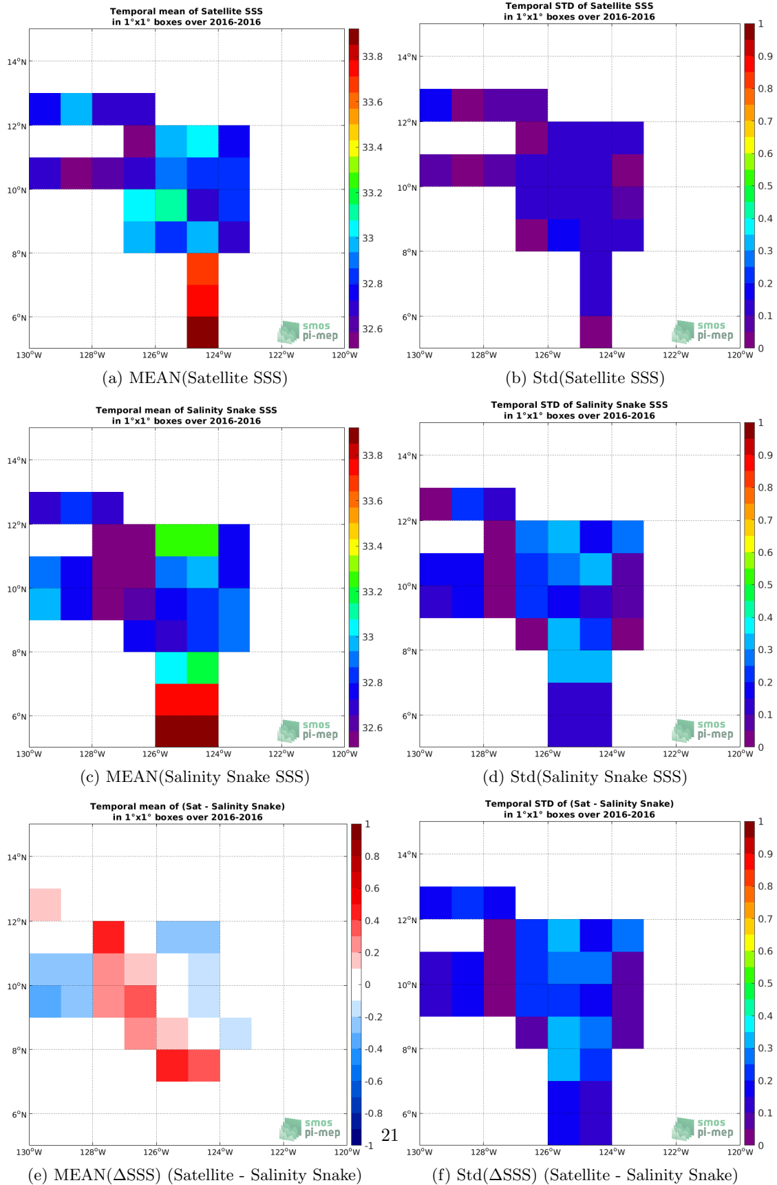
Figure 5: Temporal mean (left) and Std (right) of SSS from SMOS SSS L3 v3 Monthly (ICDC) (top), Salinity Snake (middle), and of \Delta SSS (Satellite - Salinity Snake). Only match-up pairs are used to generate these maps.
