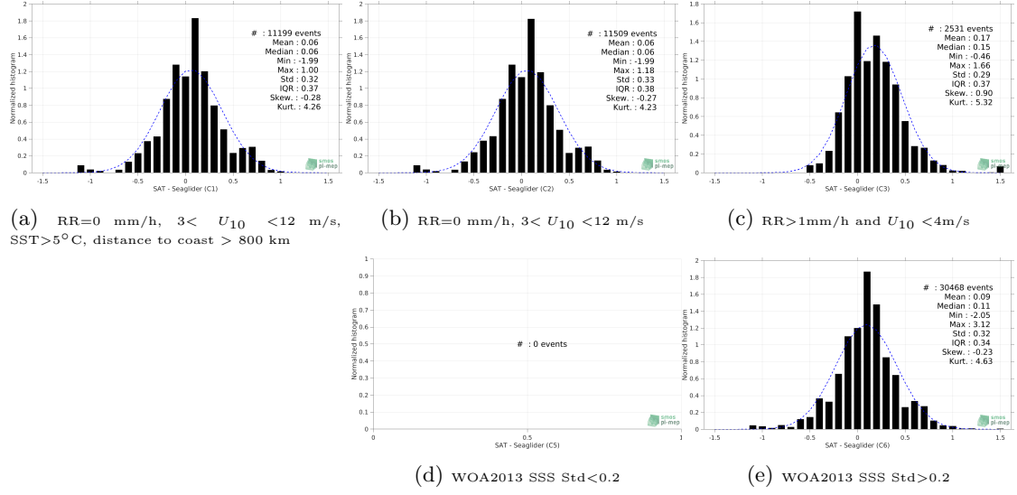
Figure 12: Normalized histogram of \Delta SSS (SMOS SSS L3 v3 Monthly (ICDC) - Seaglider) for 5 different subdatasets corresponding to: RR=0 mm/h, 3 < U_{10} < 12 m/s, SST>5°C, distance to coast > 800 km (a), RR=0 mm/h, 3 < U_{10} < 12 m/s (b), RR>1mm/h and U_{10} < 4 m/s (c), WOA2013 SSS Std<0.2 (d), WOA2013 SSS Std>0.2 (e).
