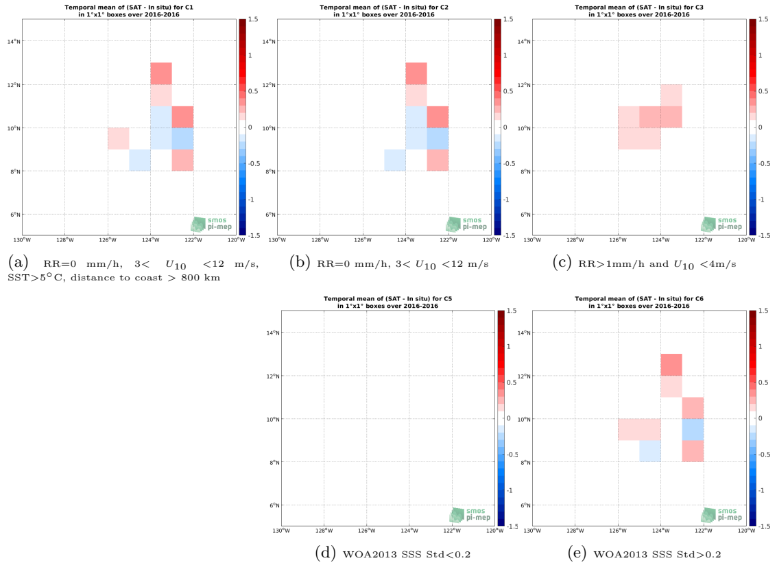
Figure 11: Temporal mean gridded over spatial boxes of size 1^\circ \times 1^\circ of \Delta SSS (SMOS SSS L3 v3 Monthly (ICDC) - Seaglider) for 5 different subdatasets corresponding to:RR=0 mm/h, 3 < U_{10} < 12 m/s, SST>5°C, distance to coast > 800 km (a), RR=0 mm/h, 3 < U_{10} < 12 m/s (b), RR>1mm/h and U_{10} < 4 m/s (c), WOA2013 SSS Std<0.2 (d), WOA2013 SSS Std>0.2 (e).
