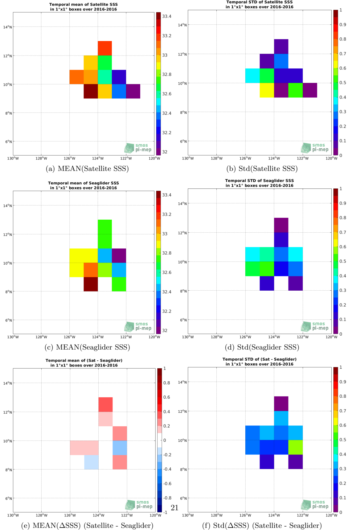
Figure 5: Temporal mean (left) and Std (right) of SSS from SMOS SSS L3 v3 Monthly (ICDC') (top), Seaglider (middle), and of \Delta SSS (Satellite - Seaglider). Only match-up pairs are used to generate these maps.
