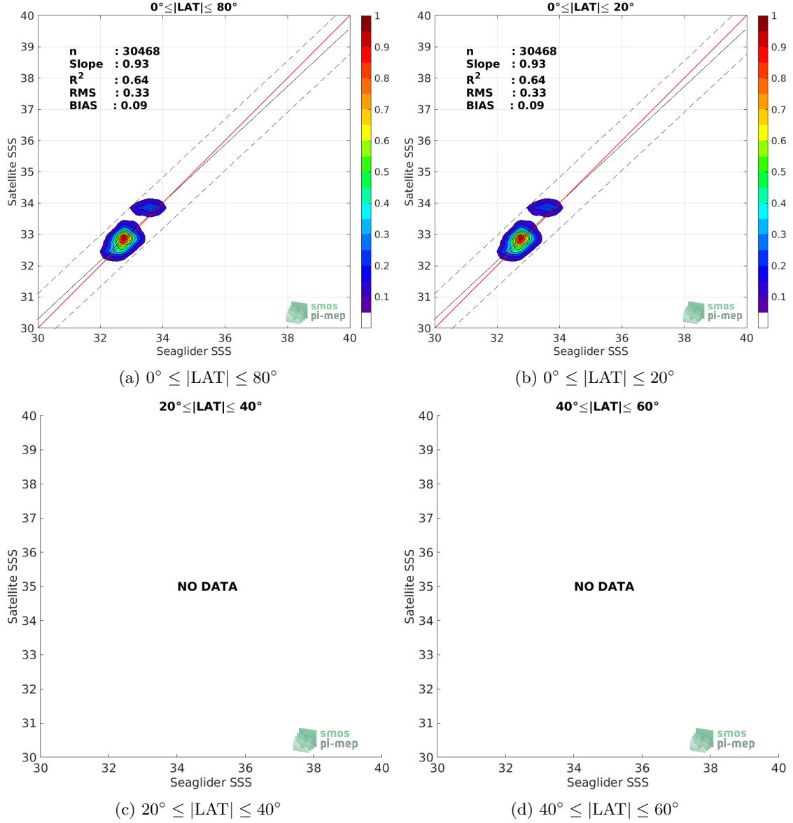
Figure 8: Contour maps of the concentration of SMOS SSS L3 v3 Monthly (ICDC) SSS (y-axis) versus Seaglider SSS (x-axis) at match-up pairs for different latitude bands. For each plot, the red line shows x=y . The black thin and dashed lines indicate a linear fit through the data cloud and the \pm 95\% confidence levels, respectively. The number match-up pairs n , the slope and R^2 coefficient of the linear fit, the root mean square (RMS) and the mean bias between satellite and in situ data are indicated for each latitude band in each plots.
