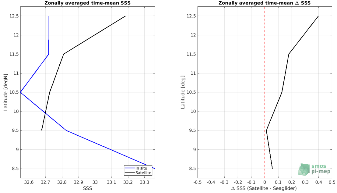
Figure 7: Left panel: Zonal mean SSS from SMOS SSS L3 v3 Monthly (ICDC) satellite product (black) and from Seaglider (blue). Right panel: Zonal mean of \Delta SSS (Satellite - Seaglider) for all the collected Pi-MEP match-up pairs estimated over the full satellite product period.
