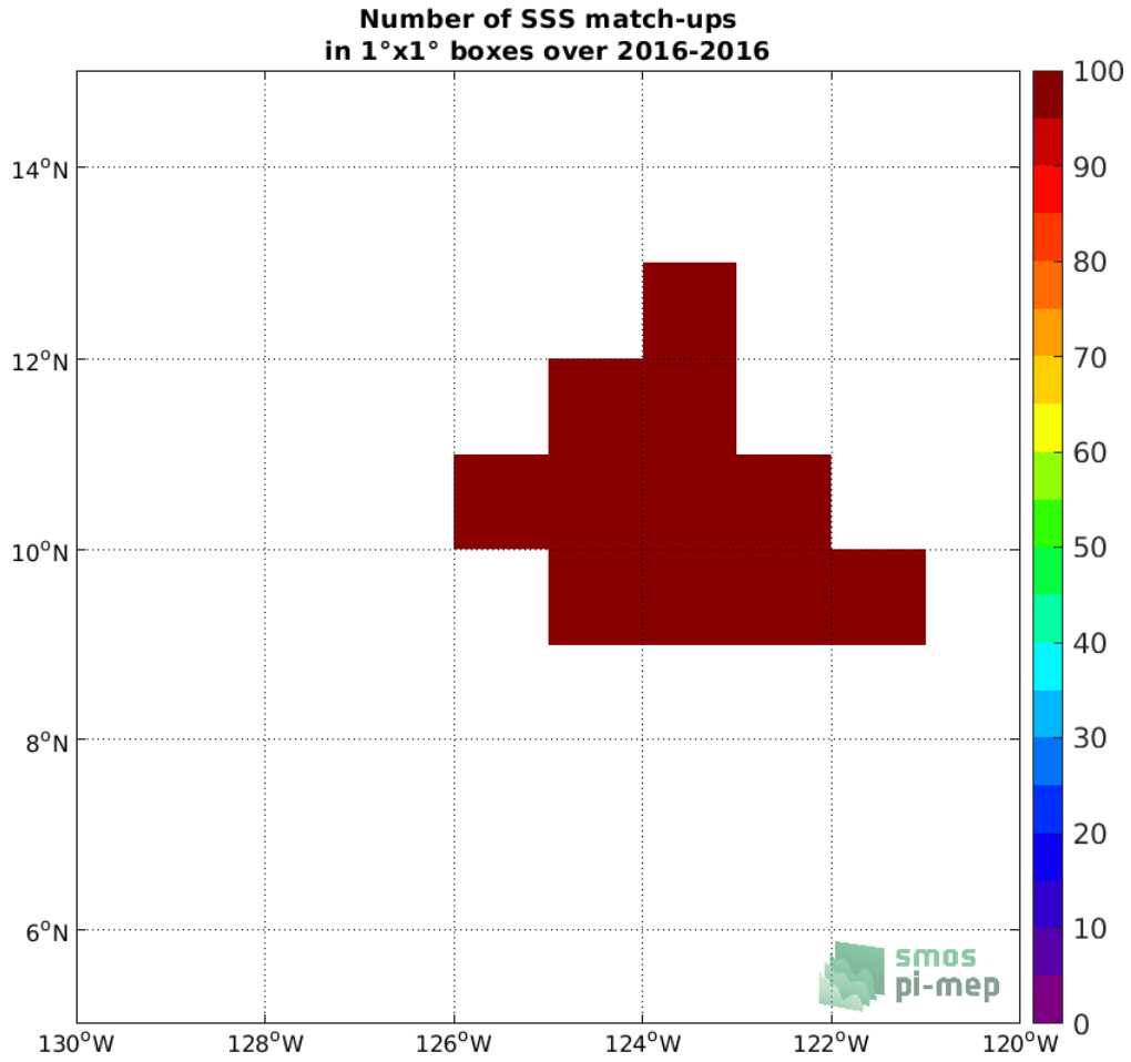
Figure 3: Number of SSS match-ups between Seagliders SSS and the SMOS SSS L3 v3 Monthly (ICDC) SSS product for the SPURS 2 Pi-MEP region over 1°x1° boxes and for the full satellite product period.
