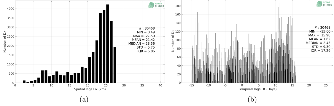
Figure 4: Histograms of the spatial (a) and temporal (b) lags between the location/time of the Seaglider measurement and the date of the corresponding SMOS SSS L3 v3 Monthly (ICDC) SSS pixel.
