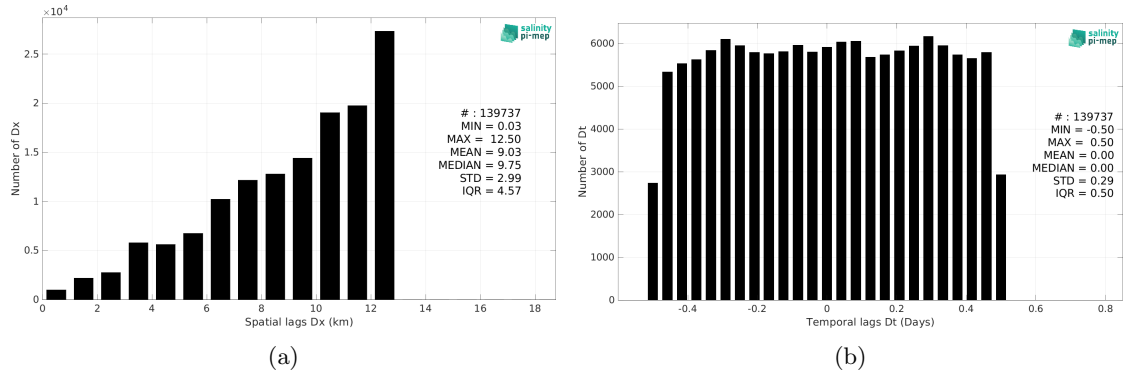
Figure 5: Histograms of the spatial (a) and temporal (b) lags between the location/time of the Waveglider (SPURS 2) measurement and the date of the corresponding SMOS SSS L2Q v331 - With FLAG (CMEMS-CATDS-CPDC) SSS pixel.
