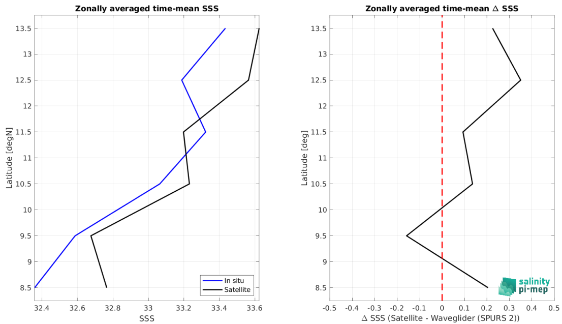
Figure 8: Left panel: Zonal mean SSS from SMOS SSS L2Q v331 - With FLAG (CMEMS-CATDS-CPDC) satellite product (black) and from Waveglider (SPURS 2) (blue). Right panel: Zonal mean of \Delta SSS (Satellite - Waveglider (SPURS 2)) for all the collected Pi-MEP match-up pairs estimated over the full satellite product period.
