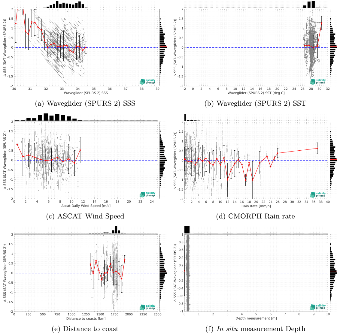
Figure 11: \Delta SSS (Satellite - Waveglider (SPURS 2)) sorted as function of Waveglider (SPURS 2) SSS values a), Waveglider (SPURS 2) SST b), ASCAT Wind speed c), CMORPH rain rate d), distance to coast (e) and in situ measurement depth (f). In all plots the median and Std of \Delta SSS for each bin is indicated by the red curves and black vertical thick bars ( \pm 1 Std)
