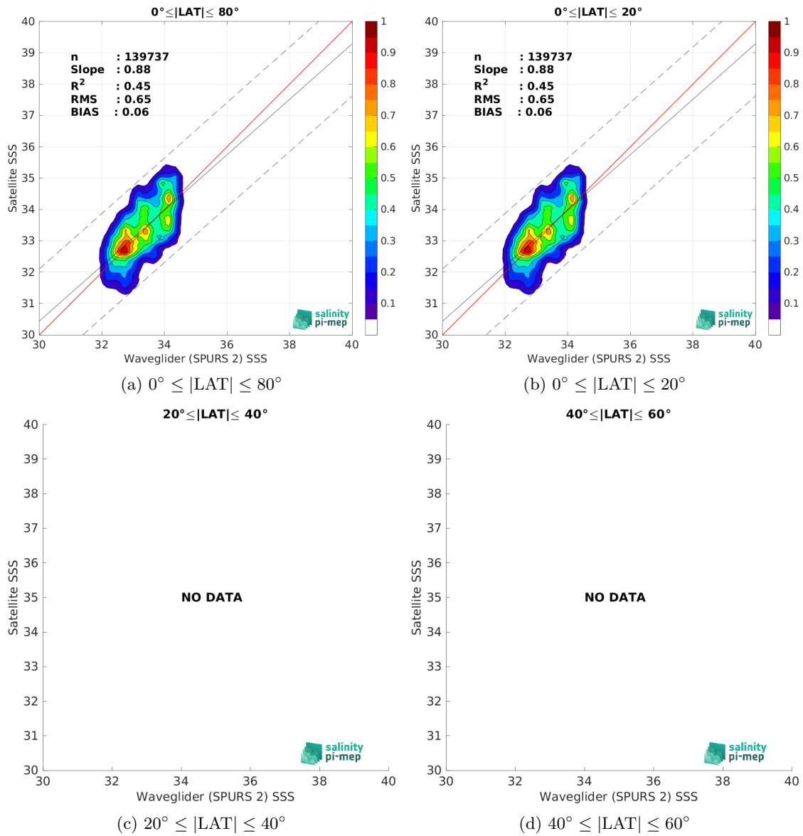
Figure 9: Contour maps of the concentration of SMOS SSS L2Q v331 - With FLAG (CMEMS-CATDS-CPDC) SSS (y-axis) versus Waveglider (SPURS 2) SSS (x-axis) at match-up pairs for different latitude bands. For each plot, the red line shows x=y . The black thin and dashed lines indicate a linear fit through the data cloud and the \pm 95\% confidence levels, respectively. The number match-up pairs n , the slope and R^2 coefficient of the linear fit, the root mean square (RMS) and the mean bias between satellite and in situ data are indicated for each latitude band in each plots.
