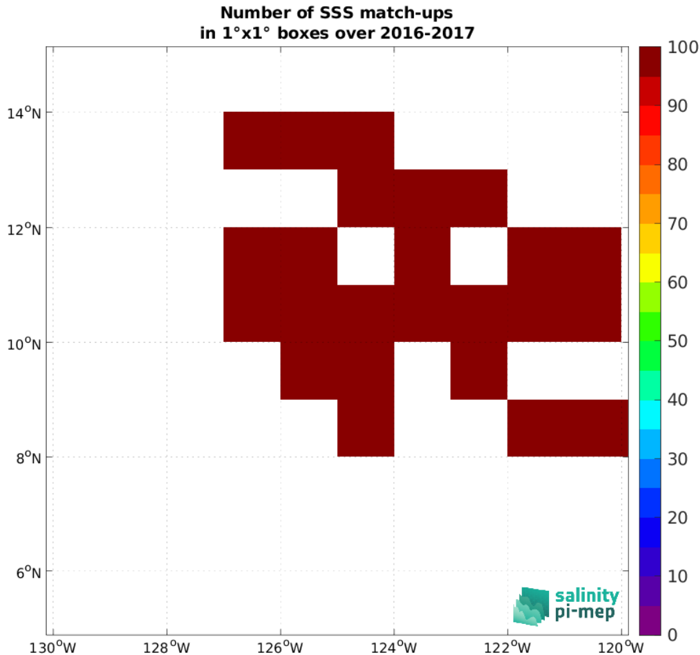
Figure 4: Number of SSS match-ups between Waveglider (SPURS 2) SSS and the SMOS SSS L2Q v331 - With FLAG (CMEMS-CATDS-CPDC) SSS product for the SPURS 2 Pi-MEP region over 1^\circ \times 1^\circ boxes and for the full satellite product period.
