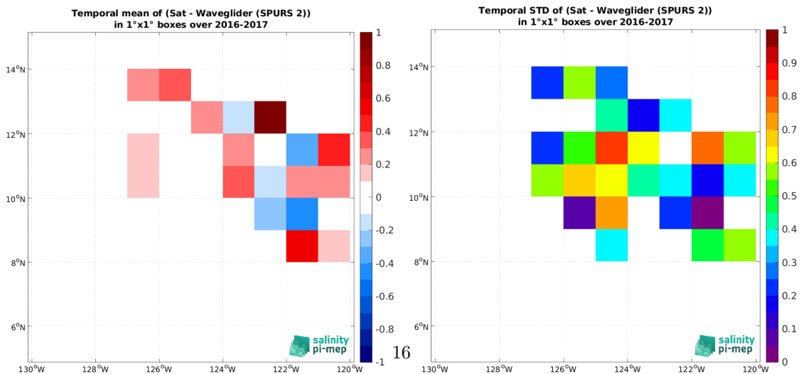
(e) MEAN( \Delta SSS) (Satellite - Waveglider (SPURS 2))
