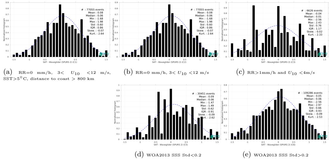
Figure 13: Normalized histogram of \Delta SSS (SMOS SSS L2Q v331 - With FLAG (CMEMS-CATDS-CPDC) - Waveglider (SPURS 2)) for 5 different subdatasets corresponding to: RR=0 mm/h, 3 < U_{10} < 12 m/s, SST>5°C, distance to coast > 800 km (a), RR=0 mm/h, 3 < U_{10} < 12 m/s (b), RR>1mm/h and U_{10} < 4 m/s (c), WOA2013 SSS Std<0.2 (d), WOA2013 SSS Std>0.2 (e).
