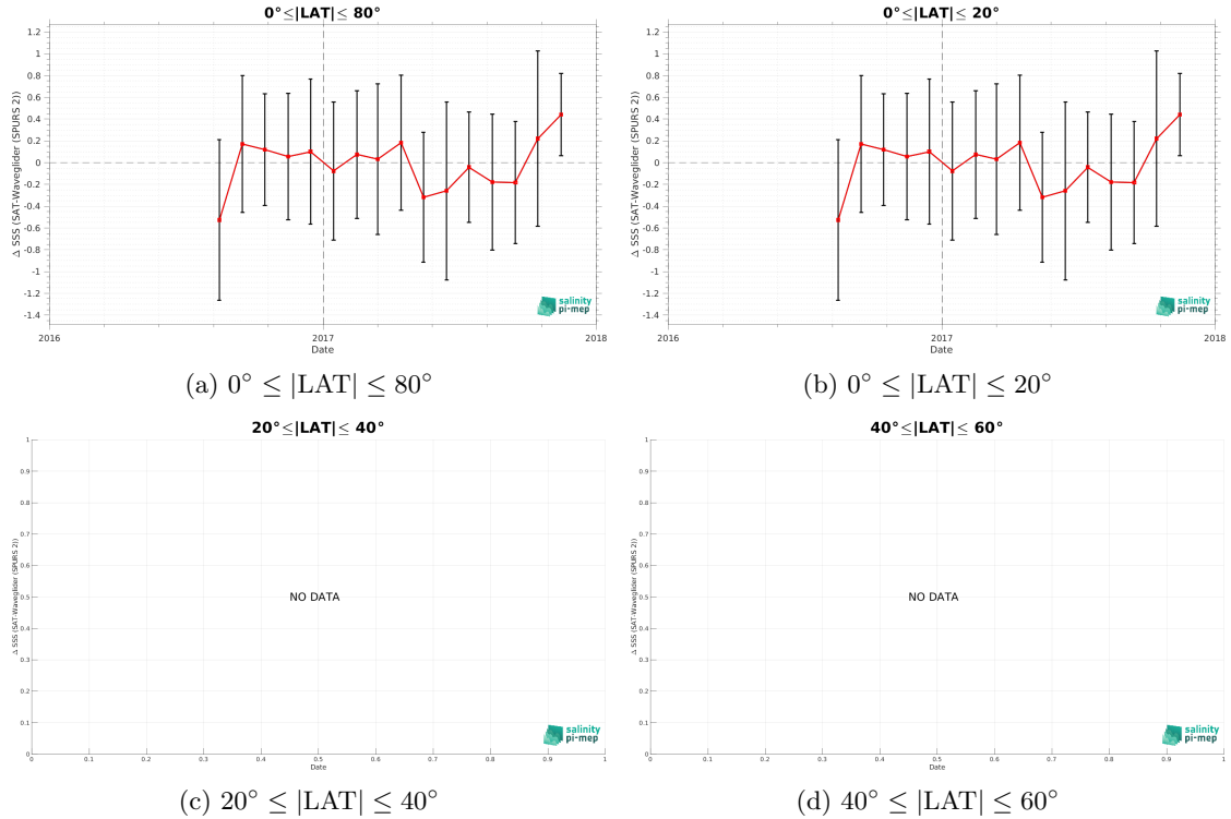
Figure 10: Monthly median (red curves) of \Delta SSS (Satellite - Waveglider (SPURS 2)) and \pm 1 Std (black vertical thick bars) as function of time for all the collected Pi-MEP match-up pairs estimated over the SPURS 2 Pi-MEP region and for the full satellite product period are shown for different latitude bands: (a) 80^\circ\text{S}-80^\circ\text{N} , (b) 20^\circ\text{S}-20^\circ\text{N} , (c) 40^\circ\text{S}-20^\circ\text{S} and 20^\circ\text{N}-40^\circ\text{N} and (d) 60^\circ\text{S}-40^\circ\text{S} and 40^\circ\text{N}-60^\circ\text{N} .
