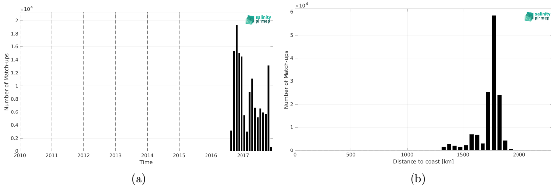
Figure 1: Number of match-ups between Waveglider (SPURS 2) and SMOS SSS L2Q v331 - With FLAG (CMEMS-CATDS-CPDC) SSS as a function of time (a) and as function of the distance to coast (b) over the SPURS 2 Pi-MEP region and for the full satellite product period.
