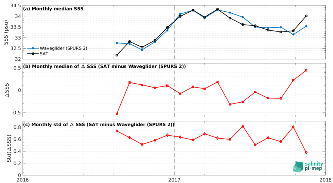
Figure 7: Time series of the monthly median SSS (top), median of \Delta SSS (Satellite - Waveglider (SPURS 2)) and Std of \Delta SSS (Satellite - Waveglider (SPURS 2)) over the SPURS 2 Pi-MEP region considering all match-ups collected by the Pi-MEP.
