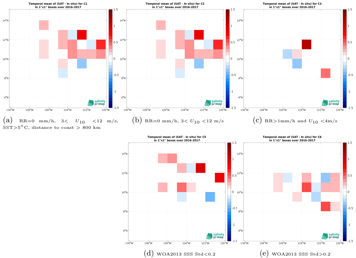
Figure 12: Temporal mean gridded over spatial boxes of size 1^{\circ}\times 1^{\circ} of \Delta\text{SSS} (SMOS SSS L2Q v331 - With FLAG (CMEMS-CATDS-CPDC) - Waveglider (SPURS 2)) for 5 different sub-datasets corresponding to:RR=0 mm/h, 3 < U_{10} < 12 m/s, SST >5^{\circ}\text{C} , distance to coast > 800 km (a), RR=0 mm/h, 3 < U_{10} < 12 m/s (b), RR >1 mm/h and U_{10} < 4 m/s (c), WOA2013 SSS Std <0.2 (d), WOA2013 SSS Std >0.2 (e).
