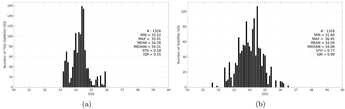
Figure 3: Histograms of SSS from TSG (SAMOS) (a) and SMOS SSS L2Q v331 - With FLAG (CMEMS-CATDS-CPDC) (b) considering all match-up pairs per bins of 0.1 over the SPURS 2 Pi-MEP region and for the full satellite product period.
