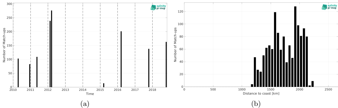
Figure 2: Number of match-ups between TSG (SAMOS) and SMOS SSS L2Q v331 - With FLAG (CMEMS-CATDS-CPDC) SSS as a function of time (a) and as function of the distance to coast (b) over the SPURS 2 Pi-MEP region and for the full satellite product period.
