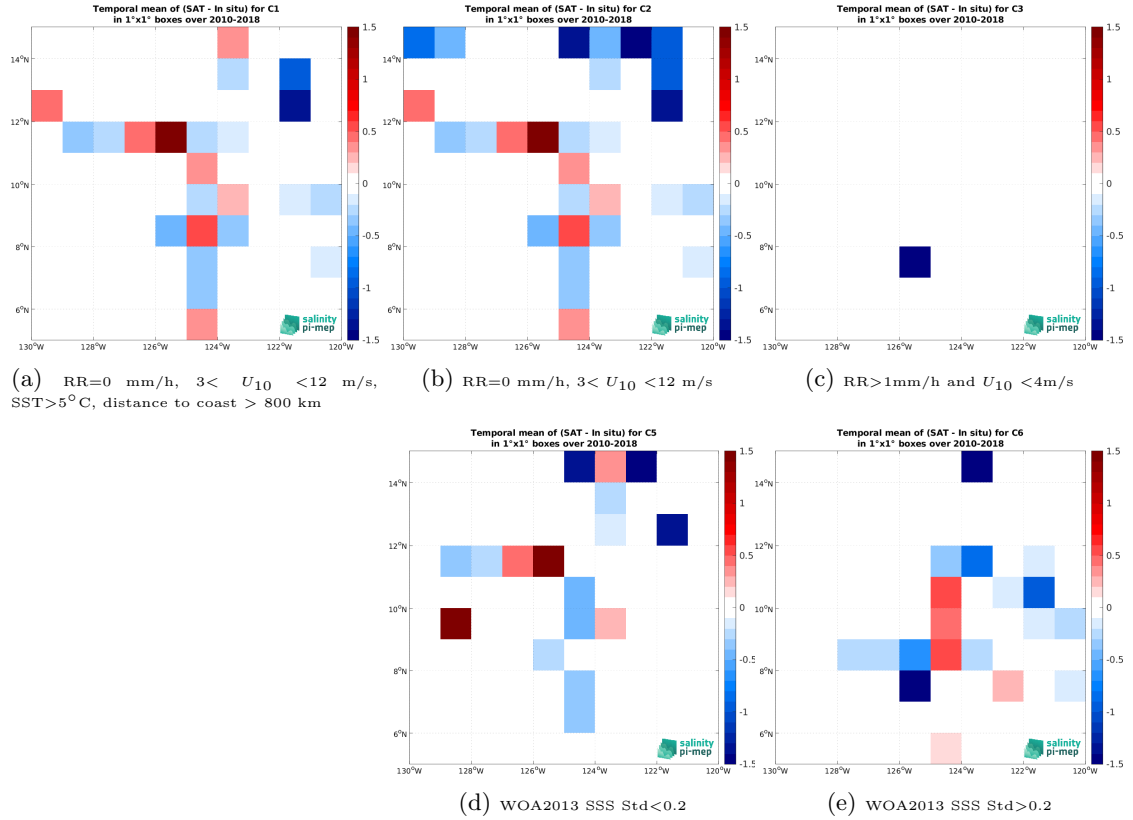
Figure 12: Temporal mean gridded over spatial boxes of size 1^{\circ}\times 1^{\circ} of \Delta\text{SSS} (SMOS SSS L2Q v331 - With FLAG (CMEMS-CATDS-CPDC) - TSG (SAMOS)) for 5 different subdatasets corresponding to:RR=0 mm/h, 3 < U_{10} < 12 m/s, SST >5^{\circ}\text{C} , distance to coast > 800 km (a), RR=0 mm/h, 3 < U_{10} < 12 m/s (b), RR >1 mm/h and U_{10} < 4 m/s (c), WOA2013 SSS Std <0.2 (d), WOA2013 SSS Std >0.2 (e).
