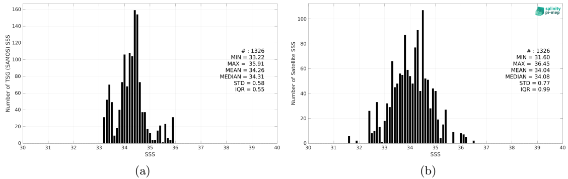
Figure 2: Histograms of SSS from TSG (SAMOS) (a) and SMOS SSS L2Q v331 - With FLAG (CMEMS-CATDS-CPDC) (b) considering all match-up pairs per bins of 0.1 over the SPURS 2 Pi-MEP region and for the full satellite product period.
