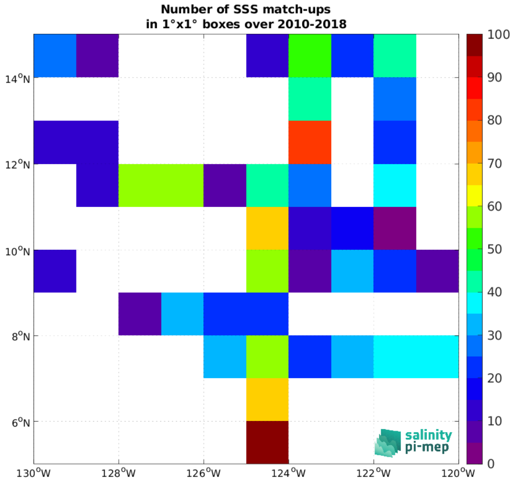
Figure 4: Number of SSS match-ups between TSG (SAMOS) SSS and the SMOS SSS L2Q v331 - With FLAG (CMEMS-CATDS-CPDC) SSS product for the SPURS 2 Pi-MEP region over 1^\circ \times 1^\circ boxes and for the full satellite product period.
