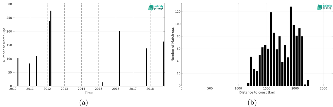
Figure 1: Number of match-ups between TSG (SAMOS) and SMOS SSS L2Q v331 - With FLAG (CMEMS-CATDS-CPDC) SSS as a function of time (a) and as function of the distance to coast (b) over the SPURS 2 Pi-MEP region and for the full satellite product period.
