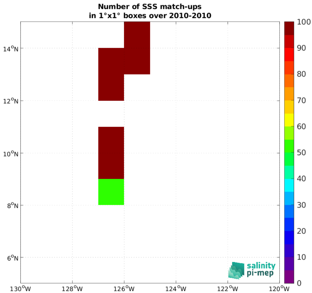
Figure 5: Number of SSS match-ups between TSG (GOSUD-Sailing-ship) SSS and the SMOS SSS L2Q v331 - With FLAG (CMEMS-CATDS-CPDC) SSS product for the SPURS 2 Pi-MEP region over 1^\circ \times 1^\circ boxes and for the full satellite product period.
