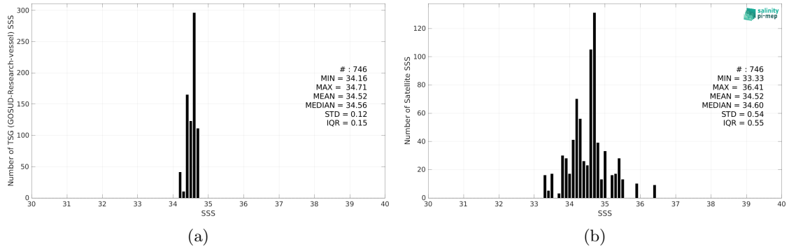
Figure 2: Histograms of SSS from TSG (GOSUD-Research-vessel) (a) and SMOS SSS L2Q v331 - With FLAG (CMEMS-CATDS-CPDC) (b) considering all match-up pairs per bins of 0.1 over the SPURS 2 Pi-MEP region and for the full satellite product period.
