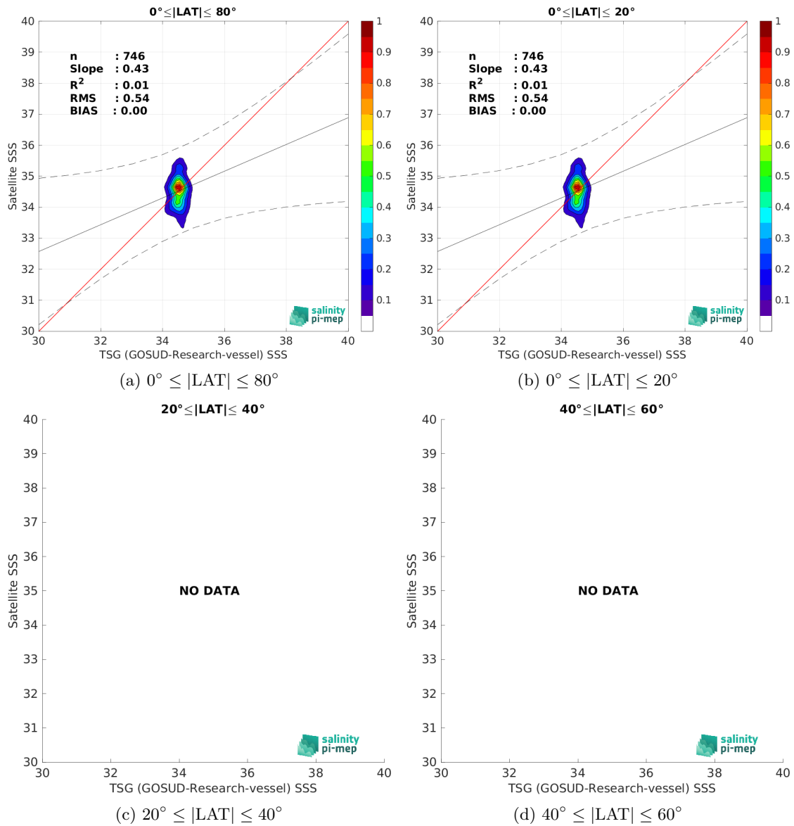
Figure 9: Contour maps of the concentration of SMOS SSS L2Q v331 - With FLAG (CMEMS-CATDS-CPDC) SSS (y-axis) versus TSG (GOSUD-Research-vessel) SSS (x-axis) at match-up pairs for different latitude bands. For each plot, the red line shows x=y . The black thin and dashed lines indicate a linear fit through the data cloud and the \pm 95\% confidence levels, respectively. The number match-up pairs n , the slope and R^2 coefficient of the linear fit, the root mean square (RMS) and the mean bias between satellite and in situ data are indicated for each latitude band in each plots.
