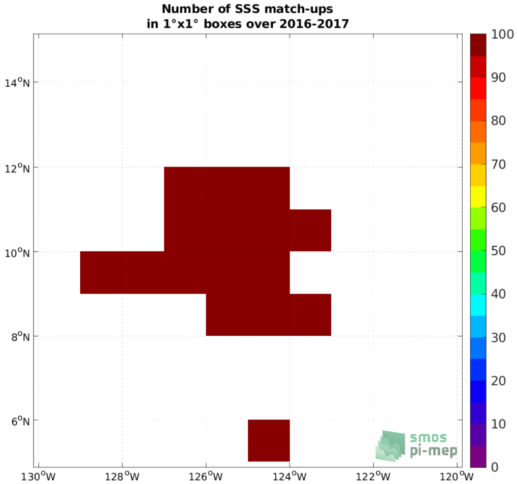
Figure 4: Number of SSS match-ups between Salinity Snake (SPURS 2) SSS and the SMOS SSS L2Q v331 - With FLAG (CMEMS-CATDS-CPDC) SSS product for the SPURS 2 Pi-MEP region over 1^\circ \times 1^\circ boxes and for the full satellite product period.
