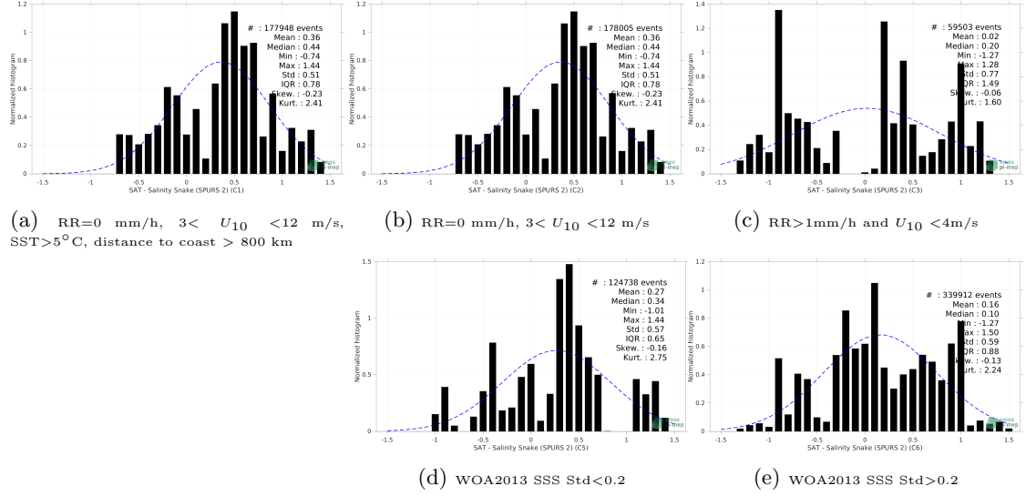
Figure 13: Normalized histogram of \Delta SSS (SMOS SSS L2Q v331 - With FLAG (CMEMS-CATDS-CPDC) - Salinity Snake (SPURS 2)) for 5 different subdatasets corresponding to: RR=0 mm/h, 3 < U_{10} < 12 m/s, SST > 5°C, distance to coast > 800 km (a), RR=0 mm/h, 3 < U_{10} < 12 m/s (b), RR > 1mm/h and U_{10} < 4 m/s (c), WOA2013 SSS Std < 0.2 (d), WOA2013 SSS Std > 0.2 (e).
