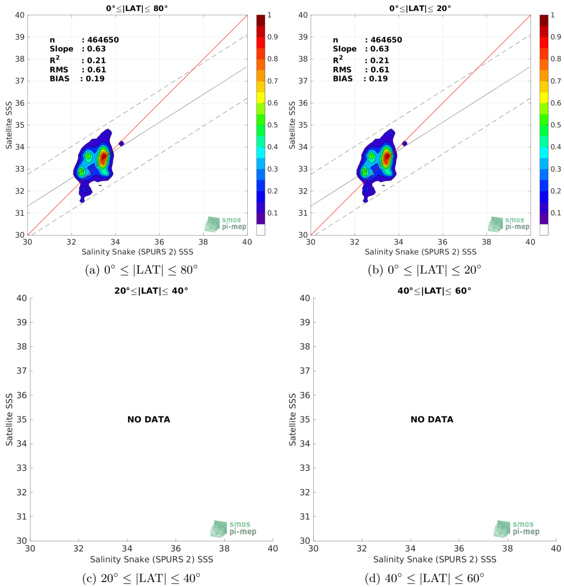
Figure 9: Contour maps of the concentration of SMOS SSS L2Q v331 - With FLAG (CMEMS-CATDS-CPDC) SSS (y-axis) versus Salinity Snake (SPURS 2) SSS (x-axis) at match-up pairs for different latitude bands. For each plot, the red line shows x=y . The black thin and dashed lines indicate a linear fit through the data cloud and the \pm 95\% confidence levels, respectively. The number match-up pairs n , the slope and R^2 coefficient of the linear fit, the root mean square (RMS) and the mean bias between satellite and in situ data are indicated for each latitude band in each plots.
