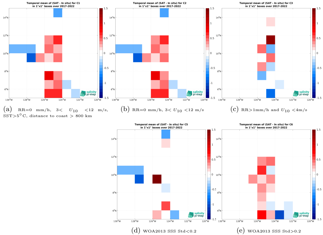
Figure 12: Temporal mean gridded over spatial boxes of size 1^\circ \times 1^\circ of \Delta\text{SSS} (SMOS SSS L2Q v331 - With FLAG (CMEMS-CATDS-CPDC) - Saildrone) for 5 different subdatasets corresponding to:RR=0 mm/h, 3 < U_{10} < 12 m/s, SST >5^\circ\text{C} , distance to coast > 800 km (a), RR=0 mm/h, 3 < U_{10} < 12 m/s (b), RR >1 mm/h and U_{10} < 4 m/s (c), WOA2013 SSS Std <0.2 (d), WOA2013 SSS Std >0.2 (e).
