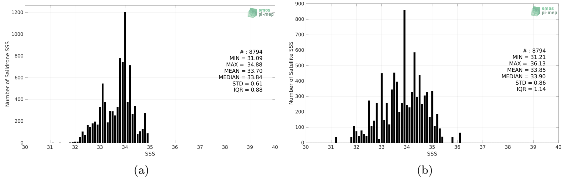
Figure 2: Histograms of SSS from Saildrone (a) and SMOS SSS L2Q v331 - With FLAG (CMEMS-CATDS-CPDC) (b) considering all match-up pairs per bins of 0.1 over the SPURS 2 Pi-MEP region and for the full satellite product period.
