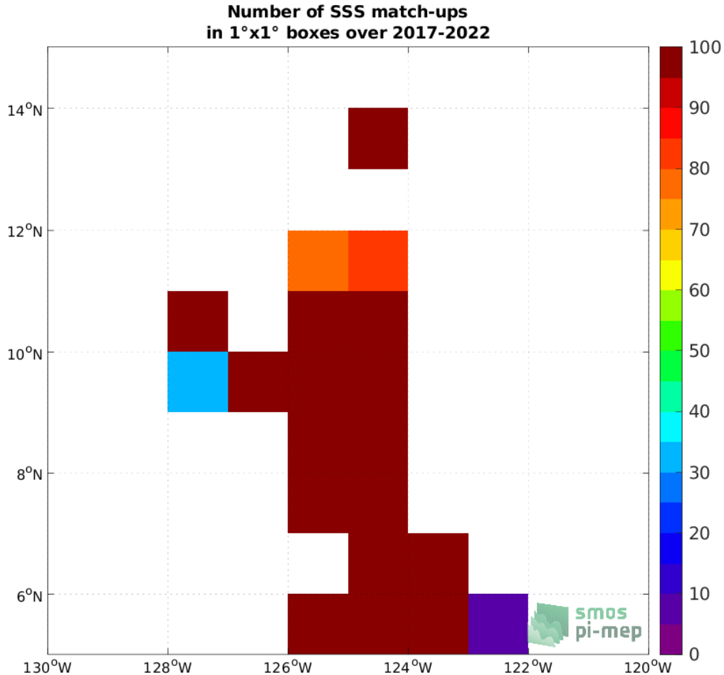
Figure 4: Number of SSS match-ups between Saildrone SSS and the SMOS SSS L2Q v331 - With FLAG (CMEMS-CATDS-CPDC) SSS product for the SPURS 2 Pi-MEP region over 1^\circ \times 1^\circ boxes and for the full satellite product period.
