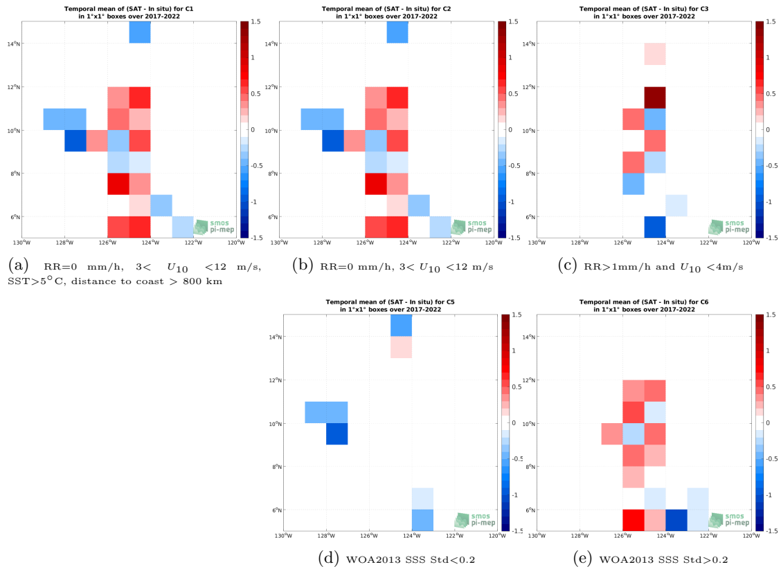
Figure 12: Temporal mean gridded over spatial boxes of size 1^\circ \times 1^\circ of \Delta SSS (SMOS SSS L2Q v331 - With FLAG (CMEMS-CATDS-CPDC) - Saildrone) for 5 different subdatasets corresponding to:RR=0 mm/h, 3 < U_{10} < 12 m/s, SST >5^\circ C, distance to coast > 800 km (a), RR=0 mm/h, 3 < U_{10} < 12 m/s (b), RR >1 mm/h and U_{10} < 4 m/s (c), WOA2013 SSS Std <0.2 (d), WOA2013 SSS Std >0.2 (e).
