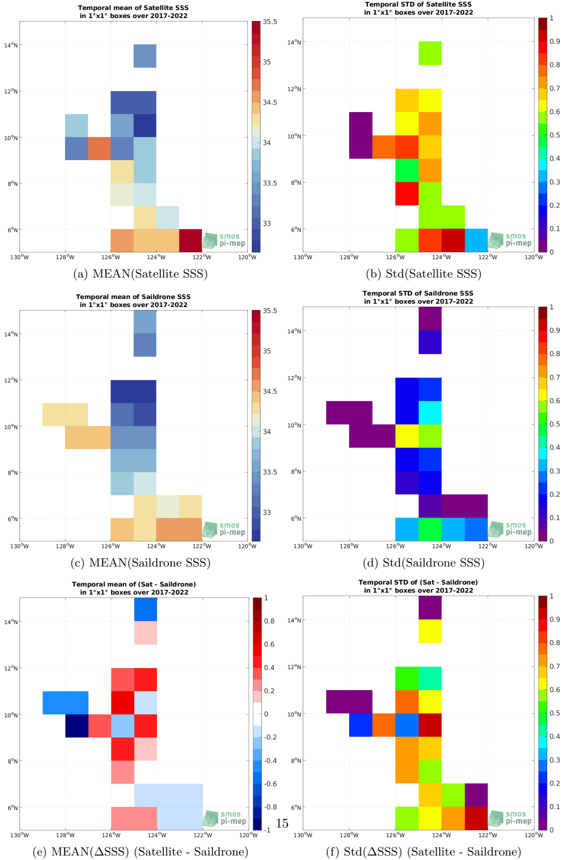
Figure 6: Temporal mean (left) and Std (right) of SSS from SMOS SSS L2Q v331 - With FLAG (CMEMS-CATDS-CPDC) (top), Saildrone (middle), and of \Delta SSS (Satellite - Saildrone). Only match-up pairs are used to generate these maps.
