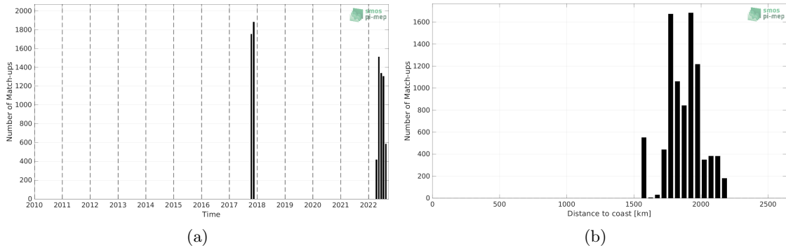
Figure 1: Number of match-ups between Saildrone and SMOS SSS L2Q v331 - With FLAG (CMEMS-CATDS-CPDC) SSS as a function of time (a) and as function of the distance to coast (b) over the SPURS 2 Pi-MEP region and for the full satellite product period.
