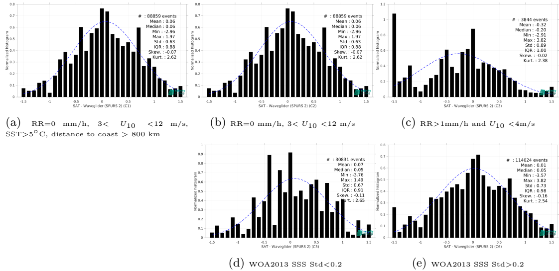
Figure 15: Normalized histogram of \Delta SSS (SMOS SSS L2Q v331 - No FLAG (CMEMS-CATDS-CPDC) - Waveglider (SPURS 2)) for 5 different subdatasets corresponding to: RR=0 mm/h, 3 < U_{10} < 12 m/s, SST > 5°C, distance to coast > 800 km (a), RR=0 mm/h, 3 < U_{10} < 12 m/s (b), RR > 1mm/h and U_{10} < 4 m/s (c), WOA2013 SSS Std < 0.2 (d), WOA2013 SSS Std > 0.2 (e).
