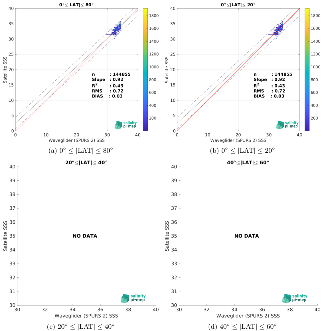
Figure 10: Contour maps of the concentration of SMOS SSS L2Q v331 - No FLAG (CMEMS-CATDS-CPDC) SSS (y-axis) versus Waveglider (SPURS 2) SSS (x-axis) at match-up pairs for different latitude bands. For each plot, the red line shows x=y . The black thin and dashed lines indicate a linear fit through the data cloud and the \pm 95\% confidence levels, respectively. The number match-up pairs n , the slope and R^2 coefficient of the linear fit, the root mean square (RMS) and the mean bias between satellite and in situ data are indicated for each latitude band in each plots.
