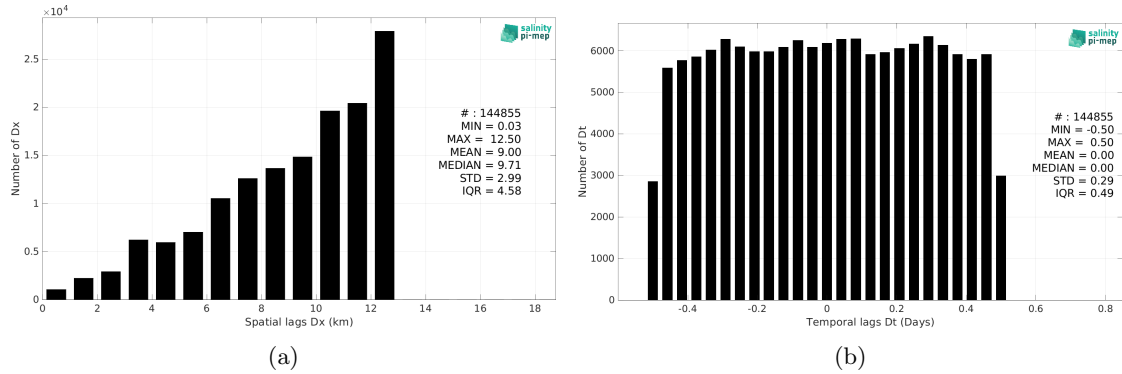
Figure 6: Histograms of the spatial (a) and temporal (b) lags between the location/time of the Waveglider (SPURS 2) measurement and the date of the corresponding SMOS SSS L2Q v331 - No FLAG (CMEMS-CATDS-CPDC) SSS pixel.
