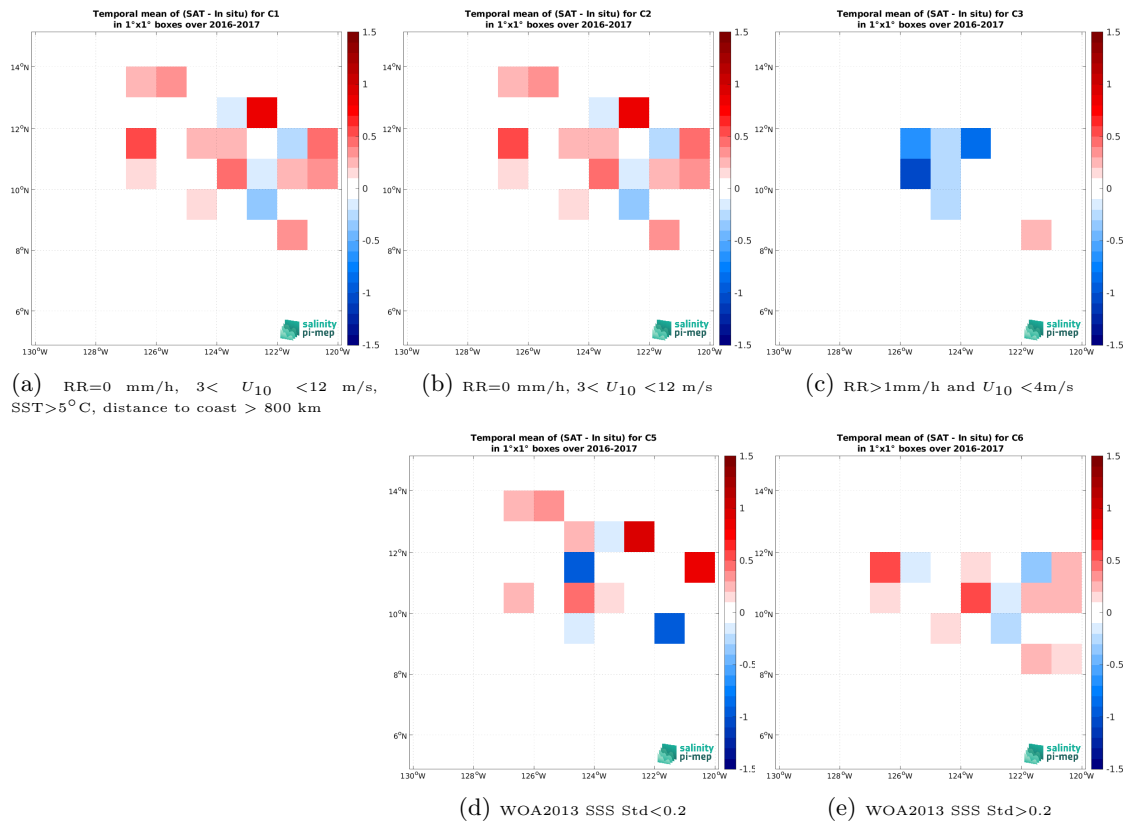
Figure 14: Temporal mean gridded over spatial boxes of size 1^\circ \times 1^\circ of \Delta SSS (SMOS SSS L2Q v331 - No FLAG (CMEMS-CATDS-CPDC) - Waveglider (SPURS 2)) for 5 different subdatasets corresponding to:RR=0 mm/h, 3 < U_{10} < 12 m/s, SST >5^\circ C, distance to coast > 800 km (a), RR=0 mm/h, 3 < U_{10} < 12 m/s (b), RR >1 mm/h and U_{10} < 4 m/s (c), WOA2013 SSS Std <0.2 (d), WOA2013 SSS Std >0.2 (e).
