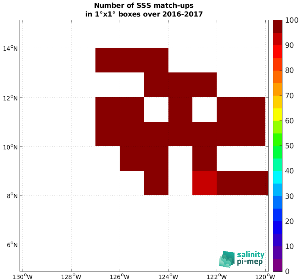
Figure 5: Number of SSS match-ups between Waveglider (SPURS 2) SSS and the SMOS SSS L2Q v331 - No FLAG (CMEMS-CATDS-CPDC) SSS product for the SPURS 2 Pi-MEP region over 1^\circ \times 1^\circ boxes and for the full satellite product period.
