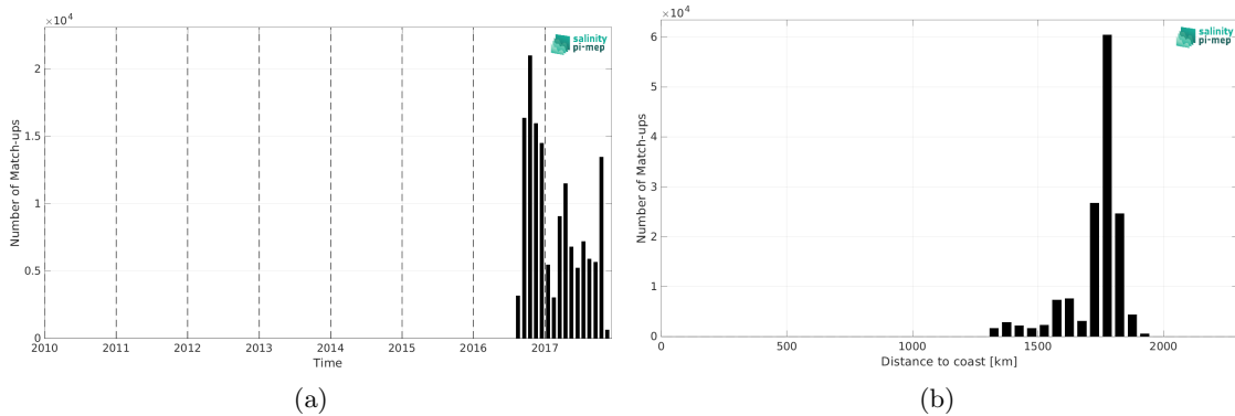
Figure 2: Number of match-ups between Waveglider (SPURS 2) and SMOS SSS L2Q v331 - No FLAG (CMEMS-CATDS-CPDC) SSS as a function of time (a) and as function of the distance to coast (b) over the SPURS 2 Pi-MEP region and for the full satellite product period.
