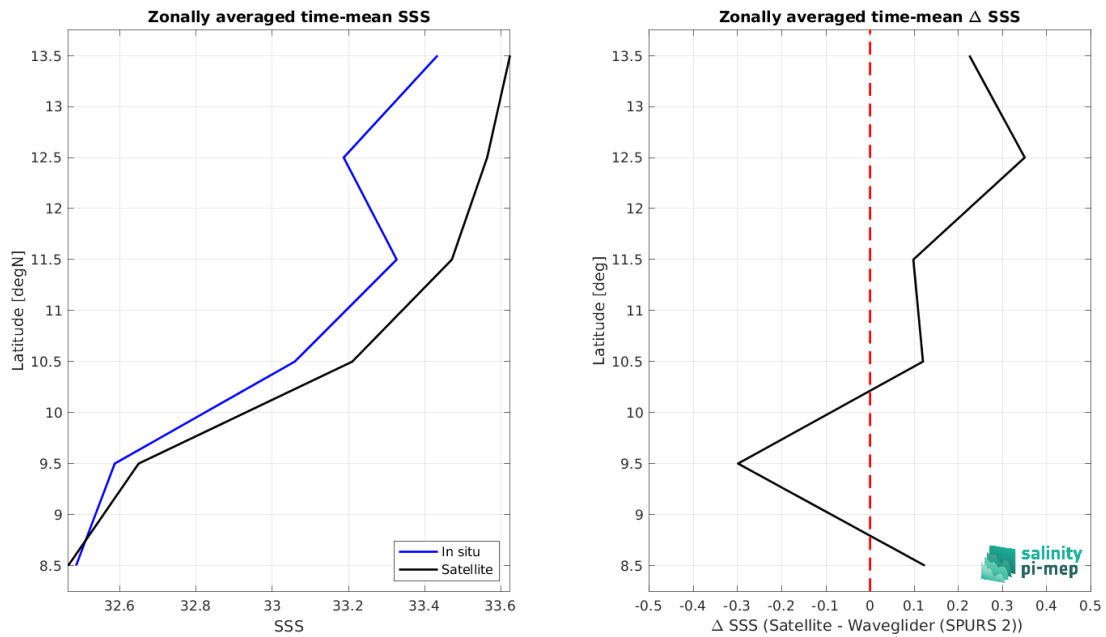
Figure 9: Left panel: Zonal mean SSS from SMOS SSS L2Q v331 - No FLAG (CMEMS-CATDS-CPDC) satellite product (black) and from Waveglider (SPURS 2) (blue). Right panel: Zonal mean of \Delta SSS (Satellite - Waveglider (SPURS 2)) for all the collected Pi-MEP match-up pairs estimated over the full satellite product period.
