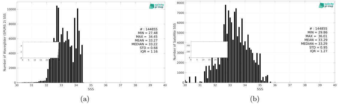
Figure 3: Histograms of SSS from Waveglider (SPURS 2) (a) and SMOS SSS L2Q v331 - No FLAG (CMEMS-CATDS-CPDC) (b) considering all match-up pairs per bins of 0.1 over the SPURS 2 Pi-MEP region and for the full satellite product period.
