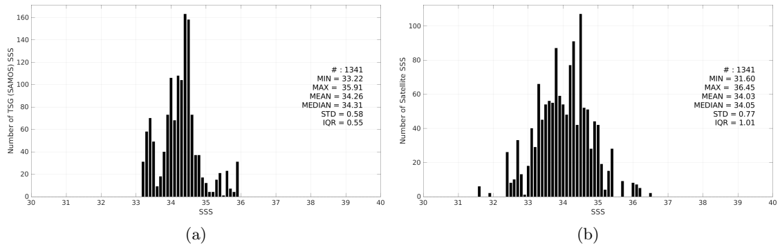
Figure 3: Histograms of SSS from TSG (SAMOS) (a) and SMOS SSS L2Q v331 - No FLAG (CMEMS-CATDS-CPDC) (b) considering all match-up pairs per bins of 0.1 over the SPURS 2 Pi-MEP region and for the full satellite product period.
