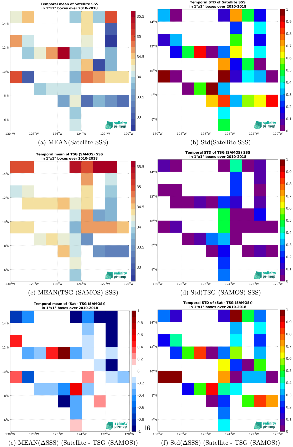
Figure 7: Temporal mean (left) and Std (right) of SSS from SMOS SSS L2Q v331 - No FLAG (CMEMS-CATDS-CPDC) (top), TSG (SAMOS) (middle), and of \Delta SSS (Satellite - TSG (SAMOS)). Only match-up pairs are used to generate these maps.
