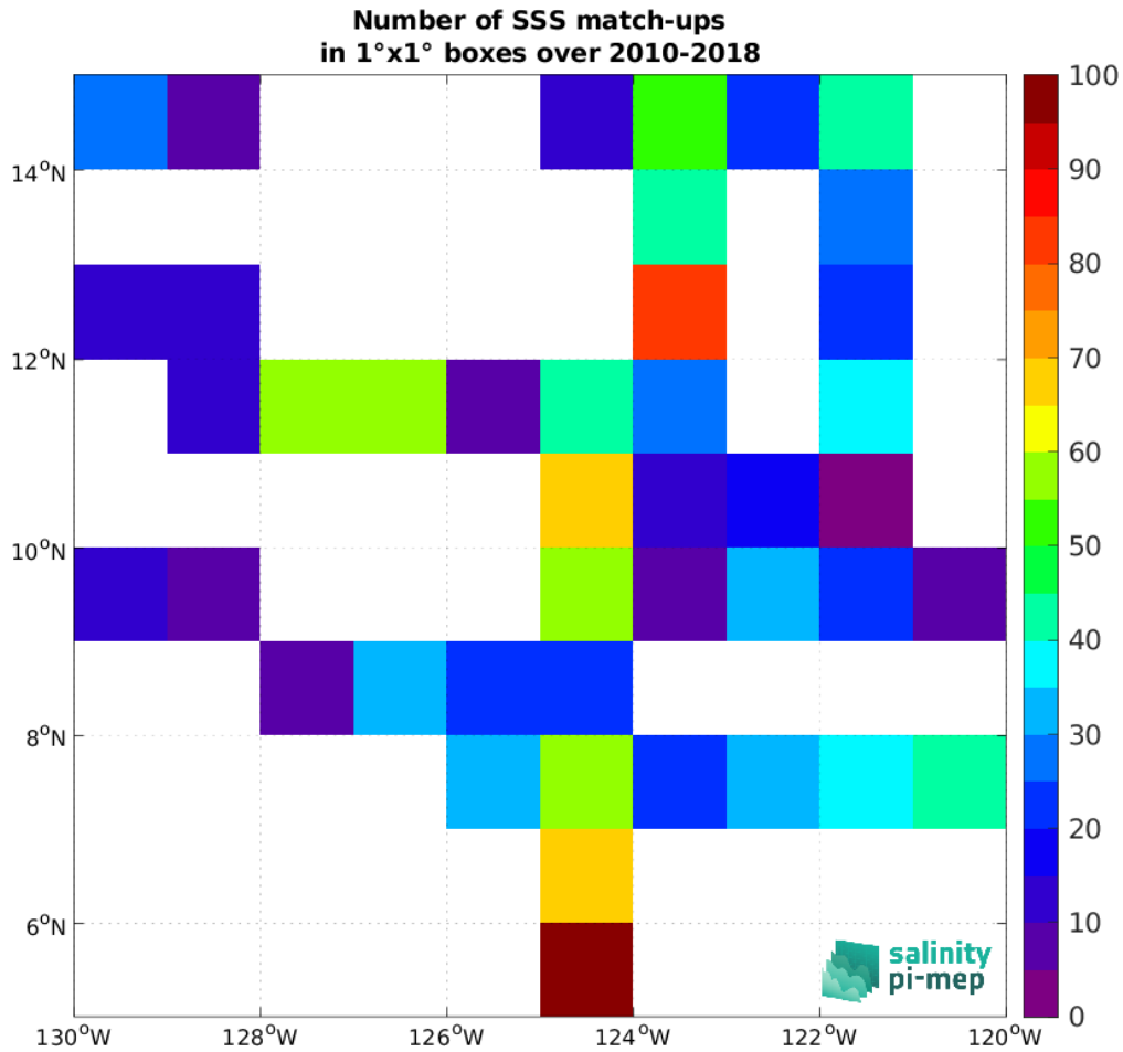
Figure 5: Number of SSS match-ups between TSG (SAMOS) SSS and the SMOS SSS L2Q v331 - No FLAG (CMEMS-CATDS-CPDC) SSS product for the SPURS 2 Pi-MEP region over 1°x1° boxes and for the full satellite product period.
