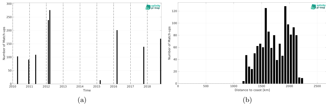
Figure 2: Number of match-ups between TSG (SAMOS) and SMOS SSS L2Q v331 - No FLAG (CMEMS-CATDS-CPDC) SSS as a function of time (a) and as function of the distance to coast (b) over the SPURS 2 Pi-MEP region and for the full satellite product period.
