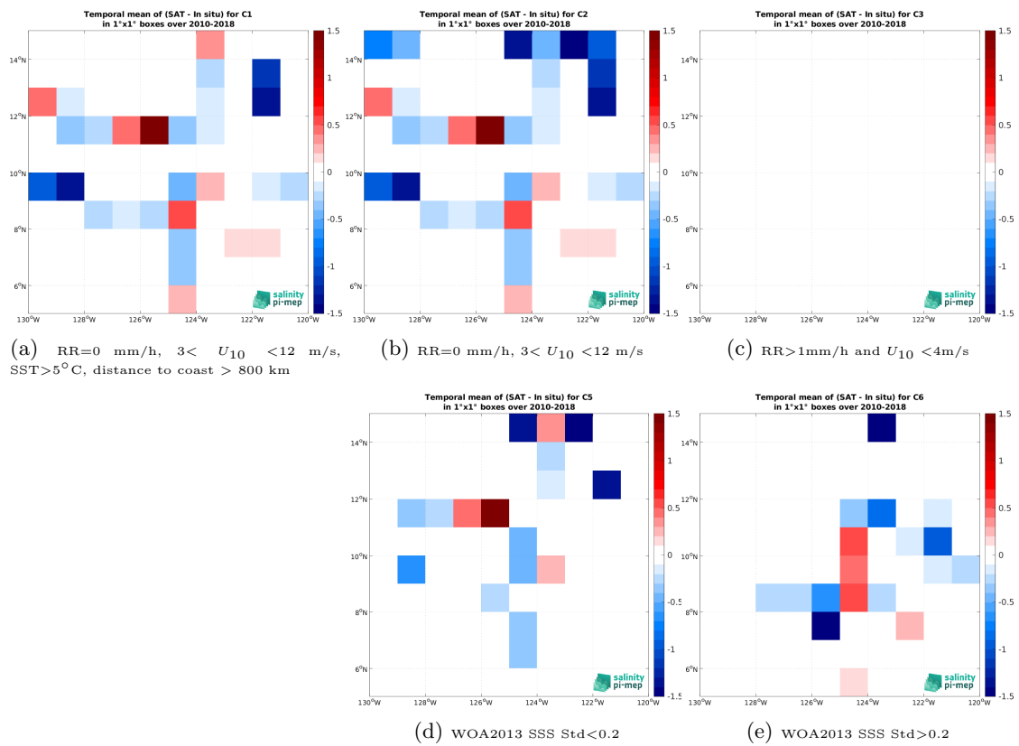
Figure 14: Temporal mean gridded over spatial boxes of size 1^\circ \times 1^\circ of \Delta\text{SSS} (SMOS SSS L2Q v331 - No FLAG (CMEMS-CATDS-CPDC) - TSG (SAMOS)) for 5 different subdatasets corresponding to:RR=0 mm/h, 3 < U_{10} < 12 m/s, SST >5^\circ\text{C} , distance to coast > 800 km (a), RR=0 mm/h, 3 < U_{10} < 12 m/s (b), RR >1 mm/h and U_{10} < 4 m/s (c), WOA2013 SSS Std <0.2 (d), WOA2013 SSS Std >0.2 (e).
