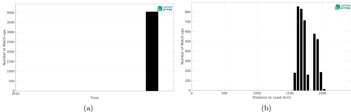
Figure 2: Number of match-ups between TSG (GOSUD-Sailing-ship) and SMOS SSS L2Q v331 - No FLAG (CMEMS-CATDS-CPDC) SSS as a function of time (a) and as function of the distance to coast (b) over the SPURS 2 Pi-MEP region and for the full satellite product period.
