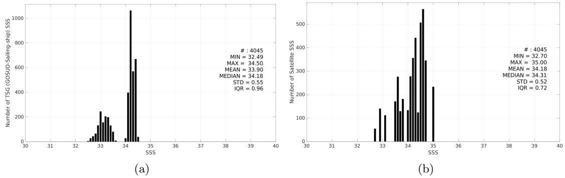
Figure 3: Histograms of SSS from TSG (GOSUD-Sailing-ship) (a) and SMOS SSS L2Q v331 - No FLAG (CMEMS-CATDS-CPDC) (b) considering all match-up pairs per bins of 0.1 over the SPURS 2 Pi-MEP region and for the full satellite product period.
