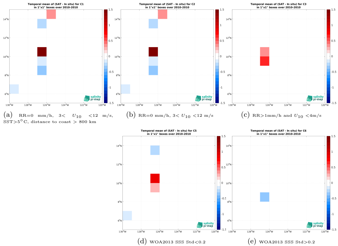
Figure 14: Temporal mean gridded over spatial boxes of size 1^\circ \times 1^\circ of \Delta SSS (SMOS SSS L2Q v331 - No FLAG (CMEMS-CATDS-CPDC) - TSG (GOSUD-Sailing-ship)) for 5 different sub-datasets corresponding to:RR=0 mm/h, 3 < U_{10} < 12 m/s, SST >5^\circ C, distance to coast > 800 km (a), RR=0 mm/h, 3 < U_{10} < 12 m/s (b), RR >1 mm/h and U_{10} < 4 m/s (c), WOA2013 SSS Std <0.2 (d), WOA2013 SSS Std >0.2 (e).
