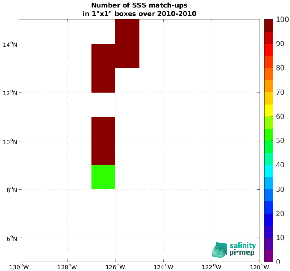
Figure 5: Number of SSS match-ups between TSG (GOSUD-Sailing-ship) SSS and the SMOS SSS L2Q v331 - No FLAG (CMEMS-CATDS-CPDC) SSS product for the SPURS 2 Pi-MEP region over 1^\circ \times 1^\circ boxes and for the full satellite product period.
