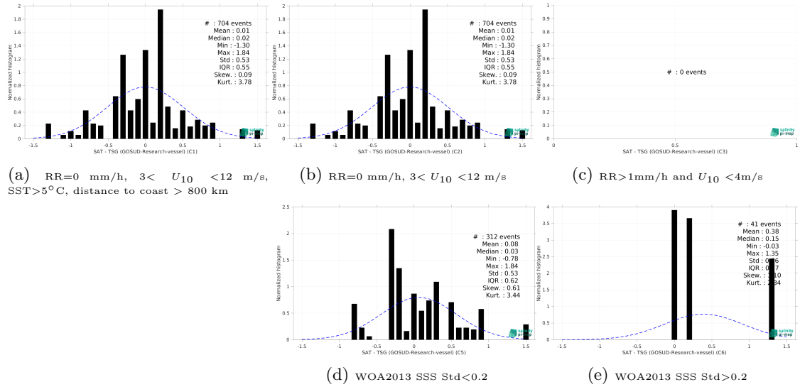
Figure 15: Normalized histogram of \Delta SSS (SMOS SSS L2Q v331 - No FLAG (CMEMS-CATDS-CPDC) - TSG (GOSUD-Research-vessel)) for 5 different subdatasets corresponding to: RR=0 mm/h, 3 < U_{10} < 12 m/s, SST>5°C, distance to coast > 800 km (a), RR=0 mm/h, 3 < U_{10} < 12 m/s (b), RR>1mm/h and U_{10} < 4 m/s (c), WOA2013 SSS Std<0.2 (d), WOA2013 SSS Std>0.2 (e).
