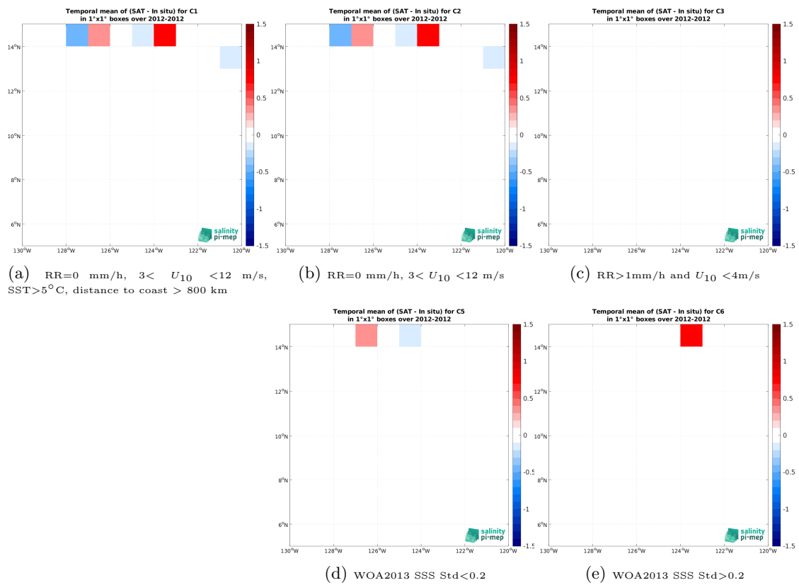
Figure 14: Temporal mean gridded over spatial boxes of size 1^\circ \times 1^\circ of \Delta SSS (SMOS SSS L2Q v331 - No FLAG (CMEMS-CATDS-CPDC) - TSG (GOSUD-Research-vessel)) for 5 different subdatasets corresponding to:RR=0 mm/h, 3 < U_{10} < 12 m/s, SST >5^\circ C, distance to coast > 800 km (a), RR=0 mm/h, 3 < U_{10} < 12 m/s (b), RR >1 mm/h and U_{10} < 4 m/s (c), WOA2013 SSS Std <0.2 (d), WOA2013 SSS Std >0.2 (e).
