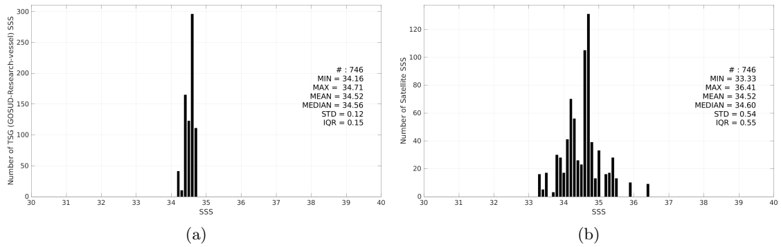
Figure 3: Histograms of SSS from TSG (GOSUD-Research-vessel) (a) and SMOS SSS L2Q v331 - No FLAG (CMEMS-CATDS-CPDC) (b) considering all match-up pairs per bins of 0.1 over the SPURS 2 Pi-MEP region and for the full satellite product period.
