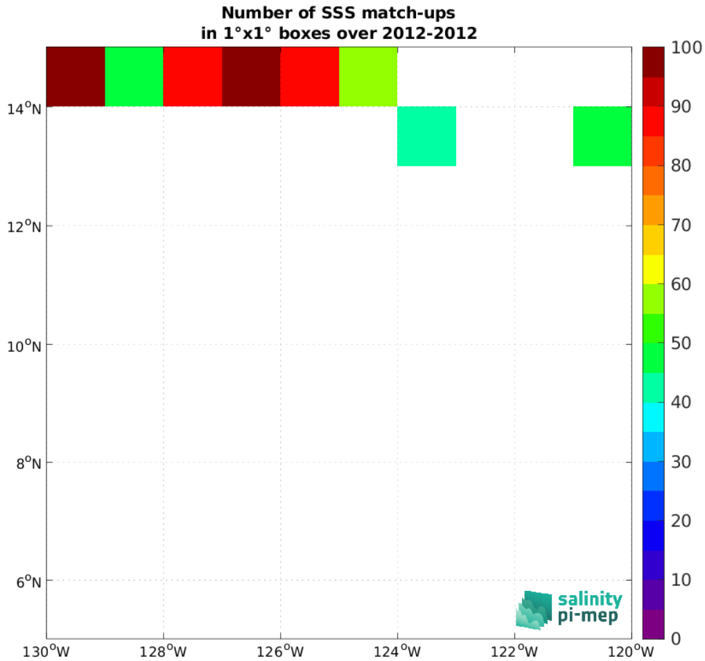
Figure 5: Number of SSS match-ups between TSG (GOSUD-Research-vessel) SSS and the SMOS SSS L2Q v331 - No FLAG (CMEMS-CATDS-CPDC) SSS product for the SPURS 2 Pi-MEP region over 1^\circ \times 1^\circ boxes and for the full satellite product period.
