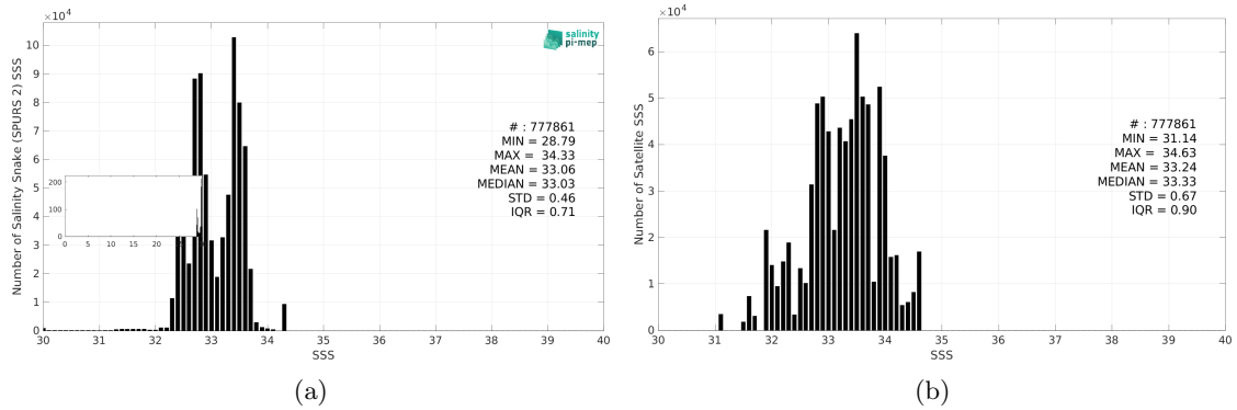
Figure 3: Histograms of SSS from Salinity Snake (SPURS 2) (a) and SMOS SSS L2Q v331 - No FLAG (CMEMS-CATDS-CPDC) (b) considering all match-up pairs per bins of 0.1 over the SPURS 2 Pi-MEP region and for the full satellite product period.
