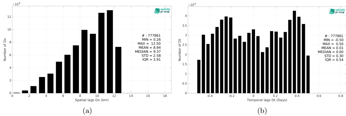
Figure 6: Histograms of the spatial (a) and temporal (b) lags between the location/time of the Salinity Snake (SPURS 2) measurement and the date of the corresponding SMOS SSS L2Q v331 - No FLAG (CMEMS-CATDS-CPDC) SSS pixel.
