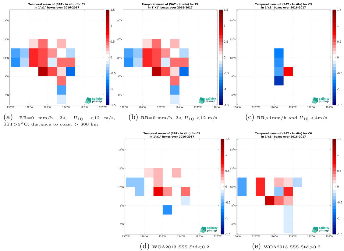
Figure 14: Temporal mean gridded over spatial boxes of size 1^\circ \times 1^\circ of \Delta\text{SSS} (SMOS SSS L2Q v331 - No FLAG (CMEMS-CATDS-CPDC) - Salinity Snake (SPURS 2)) for 5 different sub-datasets corresponding to:RR=0 mm/h, 3 < U_{10} < 12 m/s, SST>5°C, distance to coast > 800 km (a), RR=0 mm/h, 3 < U_{10} < 12 m/s (b), RR>1mm/h and U_{10} < 4 m/s (c), WOA2013 SSS Std<0.2 (d), WOA2013 SSS Std>0.2 (e).
