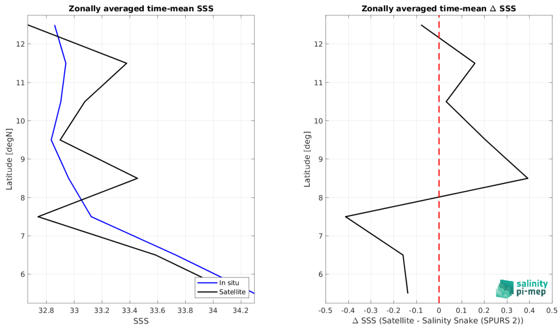
Figure 9: Left panel: Zonal mean SSS from SMOS SSS L2Q v331 - No FLAG (CMEMS-CATDS-CPDC) satellite product (black) and from Salinity Snake (SPURS 2) (blue). Right panel: Zonal mean of \Delta SSS (Satellite - Salinity Snake (SPURS 2)) for all the collected Pi-MEP match-up pairs estimated over the full satellite product period.
