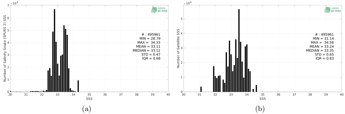
Figure 2: Histograms of SSS from Salinity Snake (SPURS 2) (a) and SMOS SSS L2Q v331 - No FLAG (CMEMS-CATDS-CPDC) (b) considering all match-up pairs per bins of 0.1 over the SPURS 2 Pi-MEP region and for the full satellite product period.
