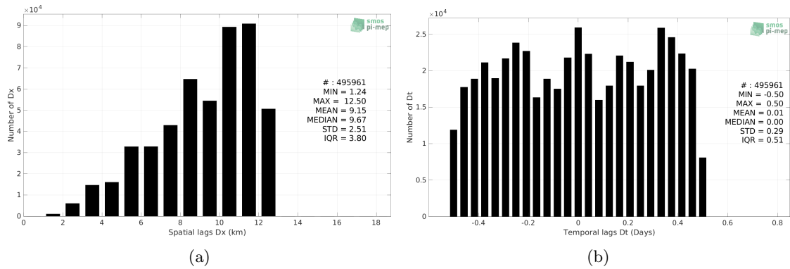
Figure 5: Histograms of the spatial (a) and temporal (b) lags between the location/time of the Salinity Snake (SPURS 2) measurement and the date of the corresponding SMOS SSS L2Q v331 - No FLAG (CMEMS-CATDS-CPDC) SSS pixel.
