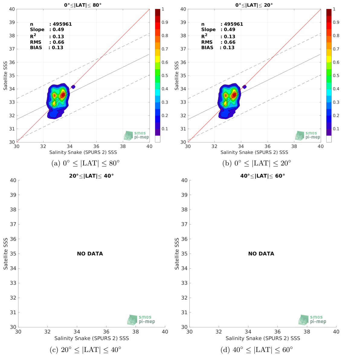
Figure 9: Contour maps of the concentration of SMOS SSS L2Q v331 - No FLAG (CMEMS-CATDS-CPDC) SSS (y-axis) versus Salinity Snake (SPURS 2) SSS (x-axis) at match-up pairs for different latitude bands. For each plot, the red line shows x=y . The black thin and dashed lines indicate a linear fit through the data cloud and the \pm 95\% confidence levels, respectively. The number match-up pairs n , the slope and R^2 coefficient of the linear fit, the root mean square (RMS) and the mean bias between satellite and in situ data are indicated for each latitude band in each plots.
