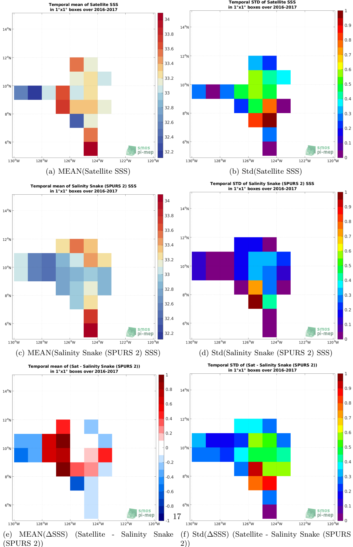
Figure 6: Temporal mean (left) and Std (right) of SSS from SMOS SSS L2Q v331 - No FLAG (CMEMS-CATDS-CPDC) (top), Salinity Snake (SPURS 2) (middle), and of \Delta SSS (Satellite - Salinity Snake (SPURS 2)). Only match-up pairs are used to generate these maps.
