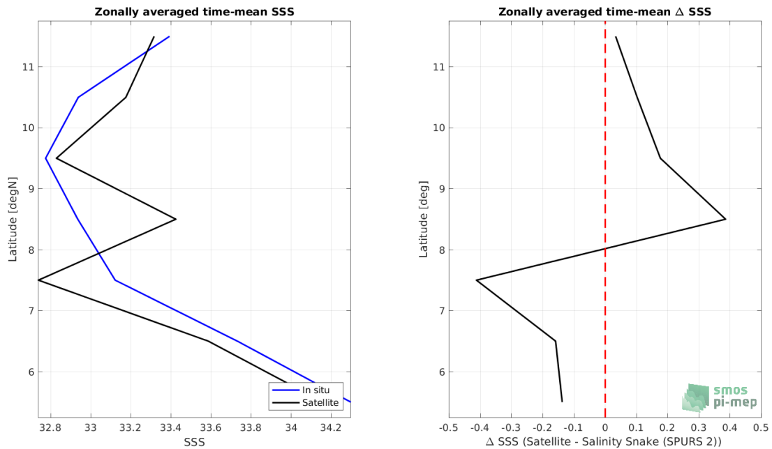
Figure 8: Left panel: Zonal mean SSS from SMOS SSS L2Q v331 - No FLAG (CMEMS-CATDS-CPDC) satellite product (black) and from Salinity Snake (SPURS 2) (blue). Right panel: Zonal mean of \Delta SSS (Satellite - Salinity Snake (SPURS 2)) for all the collected Pi-MEP match-up pairs estimated over the full satellite product period.
