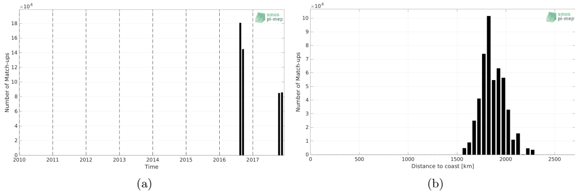
Figure 1: Number of match-ups between Salinity Snake (SPURS 2) and SMOS SSS L2Q v331 - No FLAG (CMEMS-CATDS-CPDC) SSS as a function of time (a) and as function of the distance to coast (b) over the SPURS 2 Pi-MEP region and for the full satellite product period.
