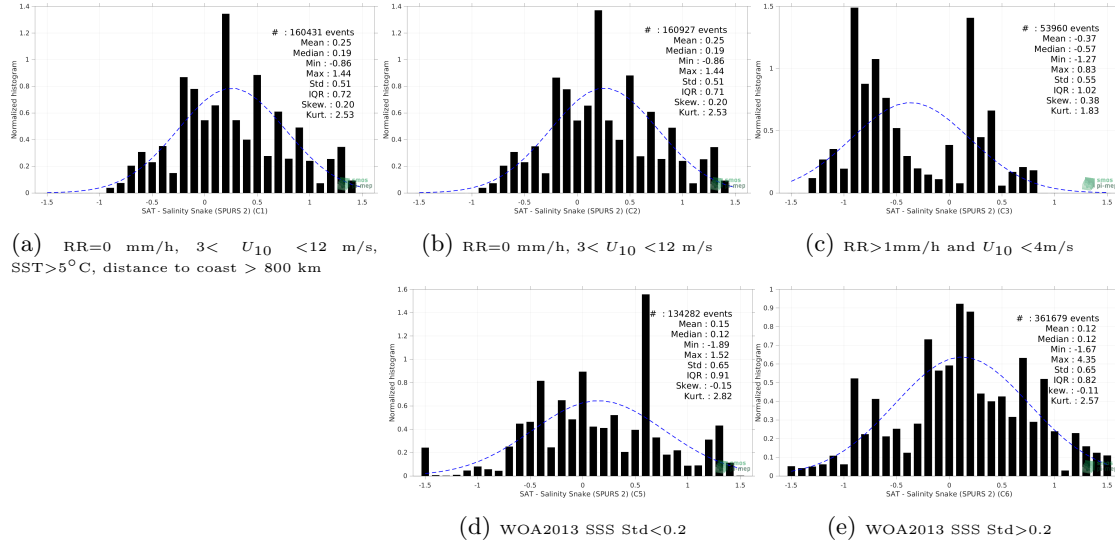
Figure 13: Normalized histogram of \Delta SSS (SMOS SSS L2Q v331 - No FLAG (CMEMS-CATDS-CPDC) - Salinity Snake (SPURS 2)) for 5 different subdatasets corresponding to: RR=0 mm/h, 3 < U_{10} < 12 m/s, SST > 5°C, distance to coast > 800 km (a), RR=0 mm/h, 3 < U_{10} < 12 m/s (b), RR > 1mm/h and U_{10} < 4 m/s (c), WOA2013 SSS Std < 0.2 (d), WOA2013 SSS Std > 0.2 (e).
