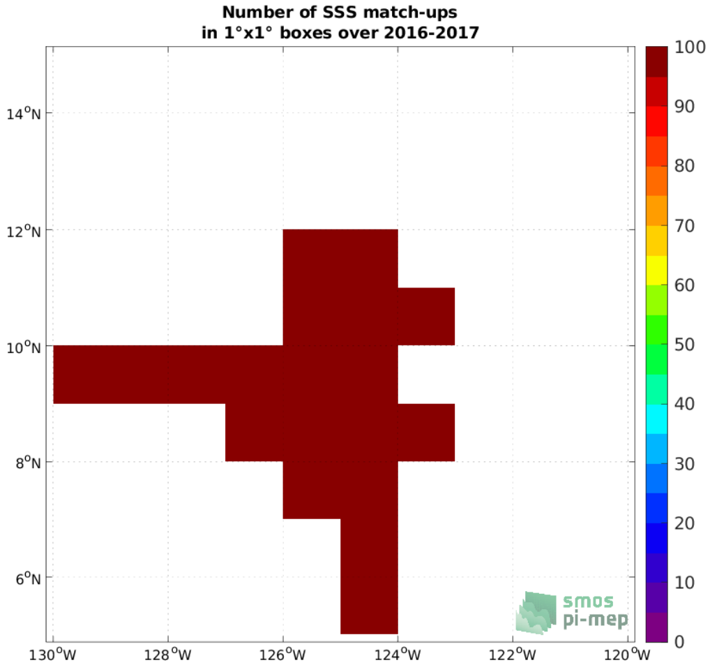
Figure 4: Number of SSS match-ups between Salinity Snake (SPURS 2) SSS and the SMOS SSS L2Q v331 - No FLAG (CMEMS-CATDS-CPDC) SSS product for the SPURS 2 Pi-MEP region over 1^\circ \times 1^\circ boxes and for the full satellite product period.
