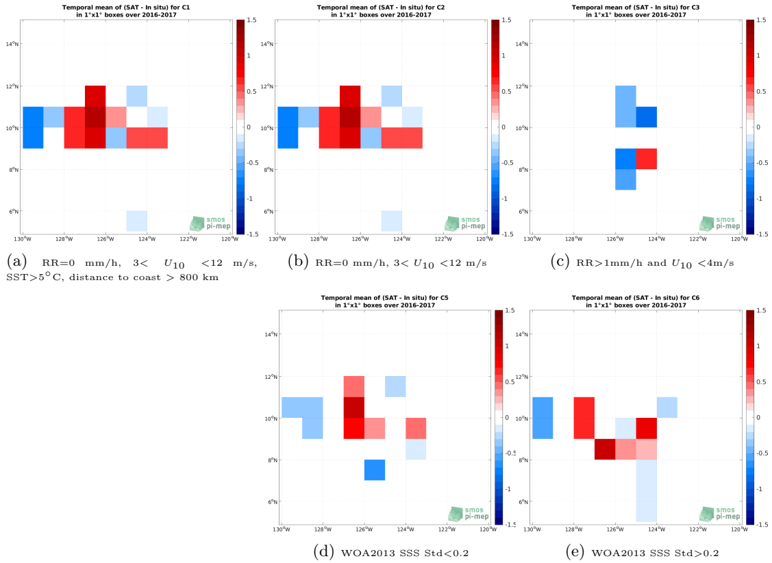
Figure 12: Temporal mean gridded over spatial boxes of size 1^\circ \times 1^\circ of \Delta SSS (SMOS SSS L2Q v331 - No FLAG (CMEMS-CATDS-CPDC) - Salinity Snake (SPURS 2)) for 5 different sub-datasets corresponding to: RR=0 mm/h, 3 < U_{10} < 12 m/s, SST > 5°C, distance to coast > 800 km (a), RR=0 mm/h, 3 < U_{10} < 12 m/s (b), RR > 1mm/h and U_{10} < 4 m/s (c), WOA2013 SSS Std < 0.2 (d), WOA2013 SSS Std > 0.2 (e).
