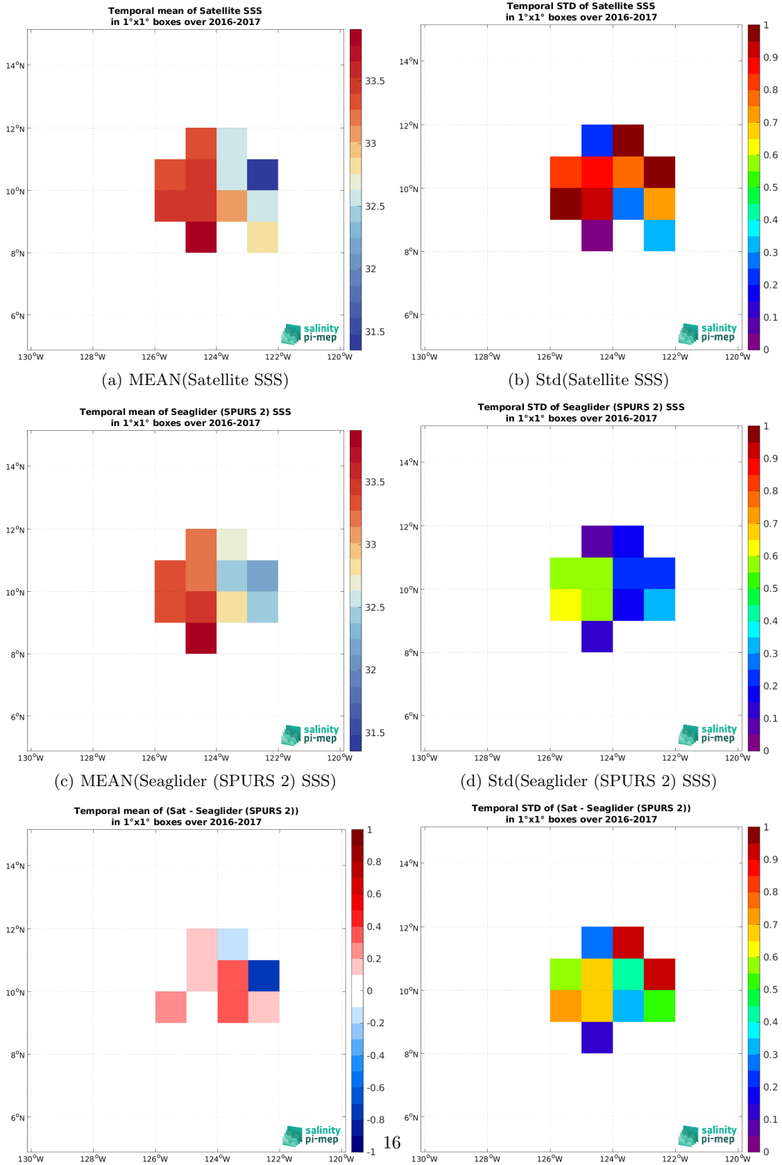
(e) MEAN( \Delta SSS) (Satellite - Seaglider (SPURS 2)) (f) Std( \Delta SSS) (Satellite - Seaglider (SPURS 2)) Figure 7: Temporal mean (left) and Std (right) of SSS from SMOS SSS L2Q v331 - No FLAG (CMEMS-CATDS-CPDC) (top), Seaglider (SPURS 2) (middle), and of \Delta SSS (Satellite - Seaglider (SPURS 2)). Only match-up pairs are used to generate these maps.
