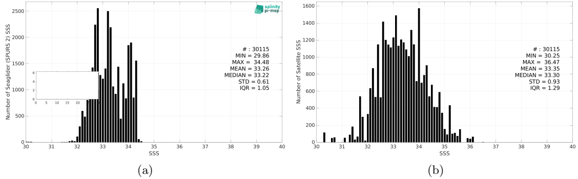
Figure 3: Histograms of SSS from Seaglider (SPURS 2) (a) and SMOS SSS L2Q v331 - No FLAG (CMEMS-CATDS-CPDC) (b) considering all match-up pairs per bins of 0.1 over the SPURS 2 Pi-MEP region and for the full satellite product period.
