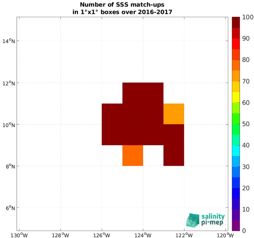
Figure 5: Number of SSS match-ups between Seaglider (SPURS 2) SSS and the SMOS SSS L2Q v331 - No FLAG (CMEMS-CATDS-CPDC) SSS product for the SPURS 2 Pi-MEP region over 1^\circ \times 1^\circ boxes and for the full satellite product period.
