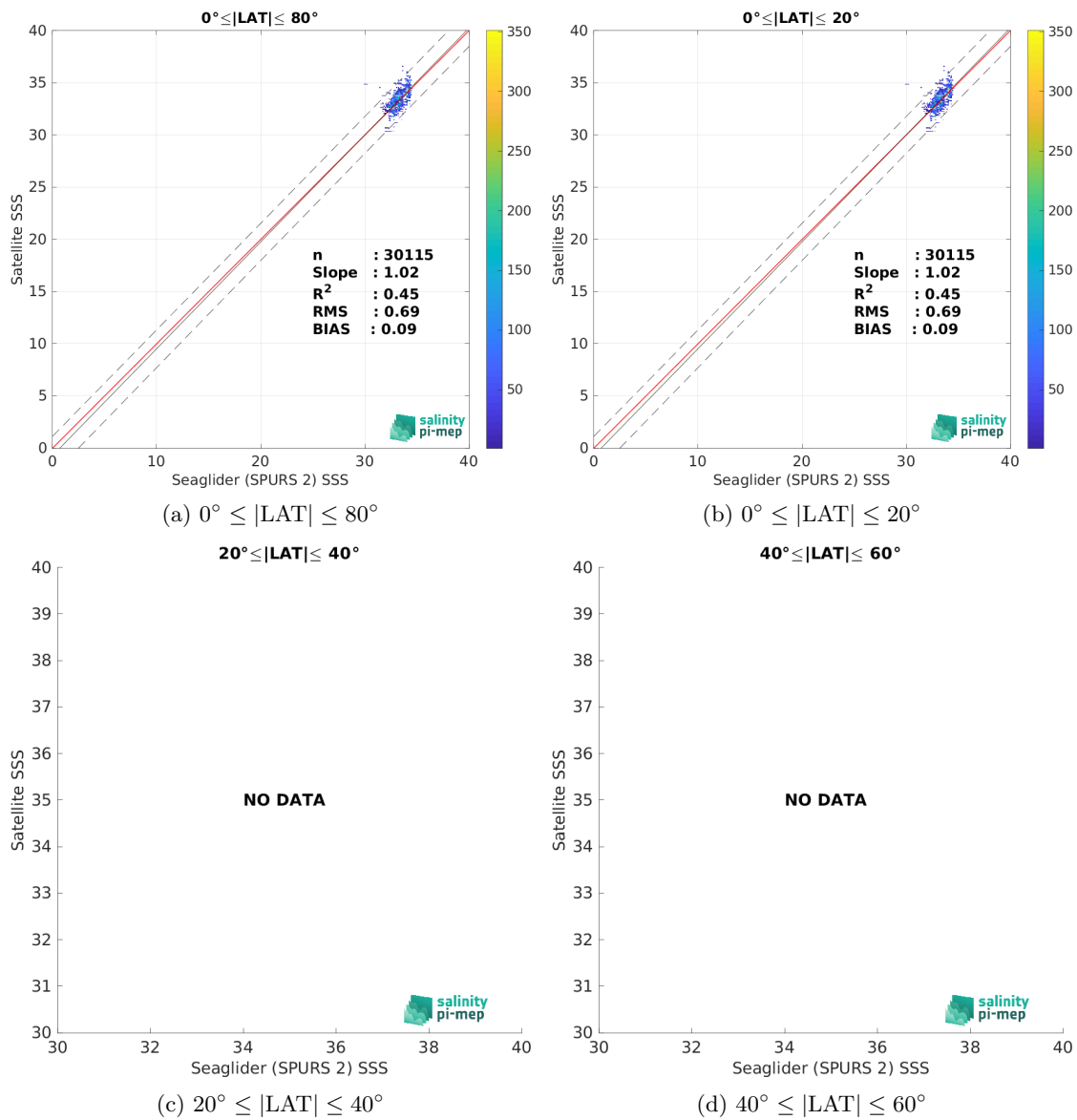
Figure 10: Contour maps of the concentration of SMOS SSS L2Q v331 - No FLAG (CMEMS-CATDS-CPDC) SSS (y-axis) versus Seaglider (SPURS 2) SSS (x-axis) at match-up pairs for different latitude bands. For each plot, the red line shows x=y . The black thin and dashed lines indicate a linear fit through the data cloud and the \pm 95\% confidence levels, respectively. The number match-up pairs n , the slope and R^2 coefficient of the linear fit, the root mean square (RMS) and the mean bias between satellite and in situ data are indicated for each latitude band in each plots.
