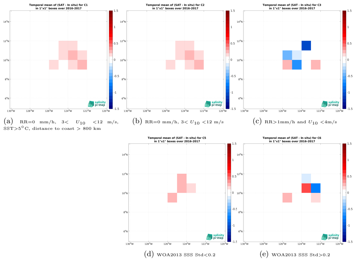
Figure 14: Temporal mean gridded over spatial boxes of size 1^\circ \times 1^\circ of \Delta\text{SSS} (SMOS SSS L2Q v331 - No FLAG (CMEMS-CATDS-CPDC) - Seaglider (SPURS 2)) for 5 different subdatasets corresponding to:RR=0 mm/h, 3 < U_{10} < 12 m/s, SST>5°C, distance to coast > 800 km (a), RR=0 mm/h, 3 < U_{10} < 12 m/s (b), RR>1mm/h and U_{10} < 4 m/s (c), WOA2013 SSS Std<0.2 (d), WOA2013 SSS Std>0.2 (e).
