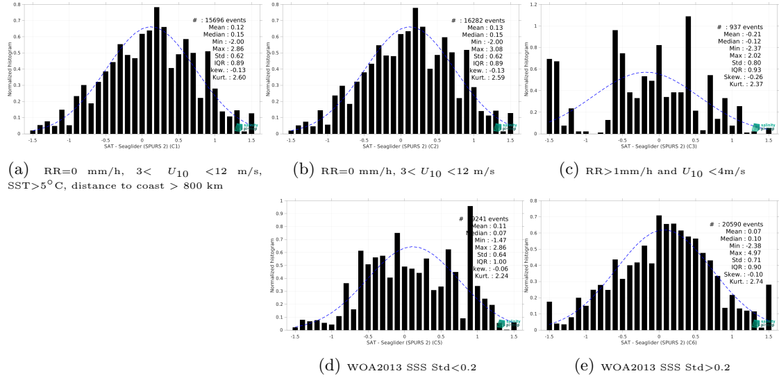
Figure 15: Normalized histogram of \Delta SSS (SMOS SSS L2Q v331 - No FLAG (CMEMS-CATDS-CPDC) - Seaglider (SPURS 2)) for 5 different subdatasets corresponding to: RR=0 mm/h, 3 < U_{10} < 12 m/s, SST > 5°C, distance to coast > 800 km (a), RR=0 mm/h, 3 < U_{10} < 12 m/s (b), RR > 1mm/h and U_{10} < 4 m/s (c), WOA2013 SSS Std < 0.2 (d), WOA2013 SSS Std > 0.2 (e).
