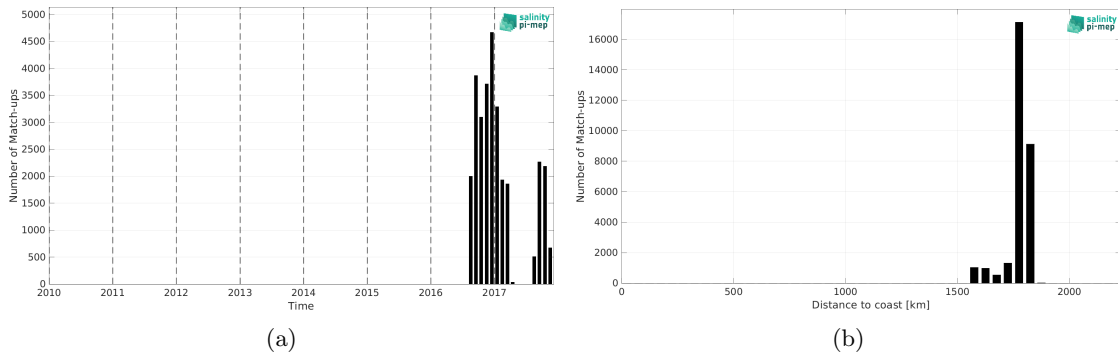
Figure 2: Number of match-ups between Seaglider (SPURS 2) and SMOS SSS L2Q v331 - No FLAG (CMEMS-CATDS-CPDC) SSS as a function of time (a) and as function of the distance to coast (b) over the SPURS 2 Pi-MEP region and for the full satellite product period.
