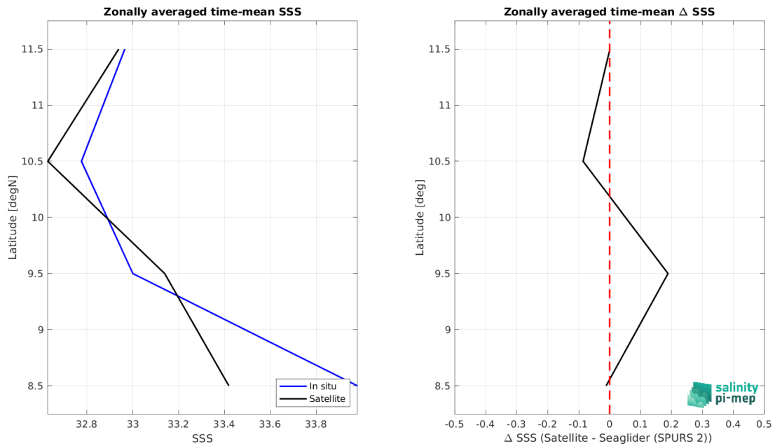
Figure 9: Left panel: Zonal mean SSS from SMOS SSS L2Q v331 - No FLAG (CMEMS-CATDS-CPDC) satellite product (black) and from Seaglider (SPURS 2) (blue). Right panel: Zonal mean of \Delta SSS (Satellite - Seaglider (SPURS 2)) for all the collected Pi-MEP match-up pairs estimated over the full satellite product period.
