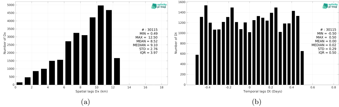
Figure 6: Histograms of the spatial (a) and temporal (b) lags between the location/time of the Seaglider (SPURS 2) measurement and the date of the corresponding SMOS SSS L2Q v331 - No FLAG (CMEMS-CATDS-CPDC) SSS pixel.
