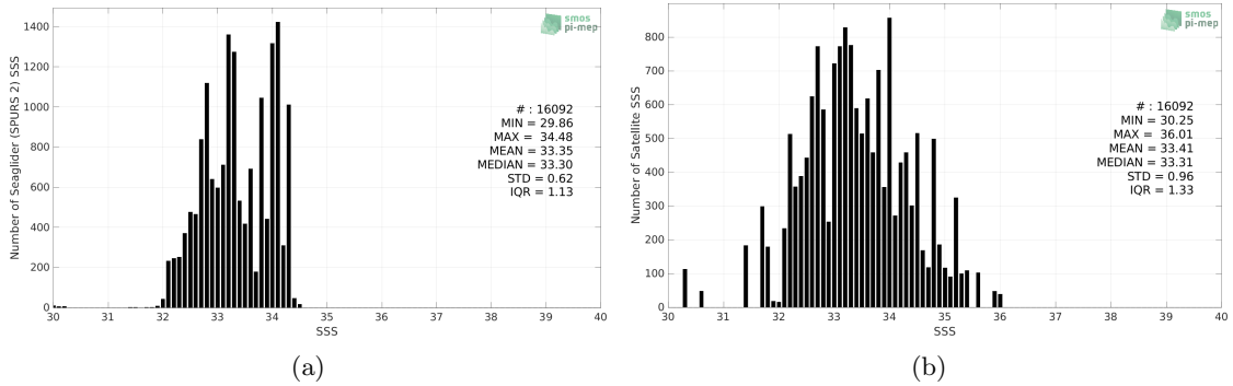
Figure 2: Histograms of SSS from Seaglider (SPURS 2) (a) and SMOS SSS L2Q v331 - No FLAG (CMEMS-CATDS-CPDC) (b) considering all match-up pairs per bins of 0.1 over the SPURS 2 Pi-MEP region and for the full satellite product period.
