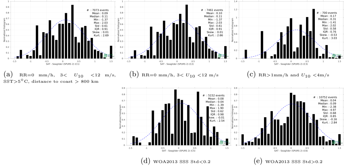
Figure 13: Normalized histogram of \Delta SSS (SMOS SSS L2Q v331 - No FLAG (CMEMS-CATDS-CPDC) - Seaglider (SPURS 2)) for 5 different subdatasets corresponding to: RR=0 mm/h, 3 < U_{10} < 12 m/s, SST > 5°C, distance to coast > 800 km (a), RR=0 mm/h, 3 < U_{10} < 12 m/s (b), RR > 1mm/h and U_{10} < 4 m/s (c), WOA2013 SSS Std < 0.2 (d), WOA2013 SSS Std > 0.2 (e).
