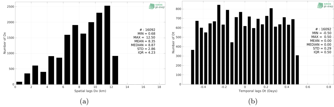
Figure 5: Histograms of the spatial (a) and temporal (b) lags between the location/time of the Seaglider (SPURS 2) measurement and the date of the corresponding SMOS SSS L2Q v331 - No FLAG (CMEMS-CATDS-CPDC) SSS pixel.
