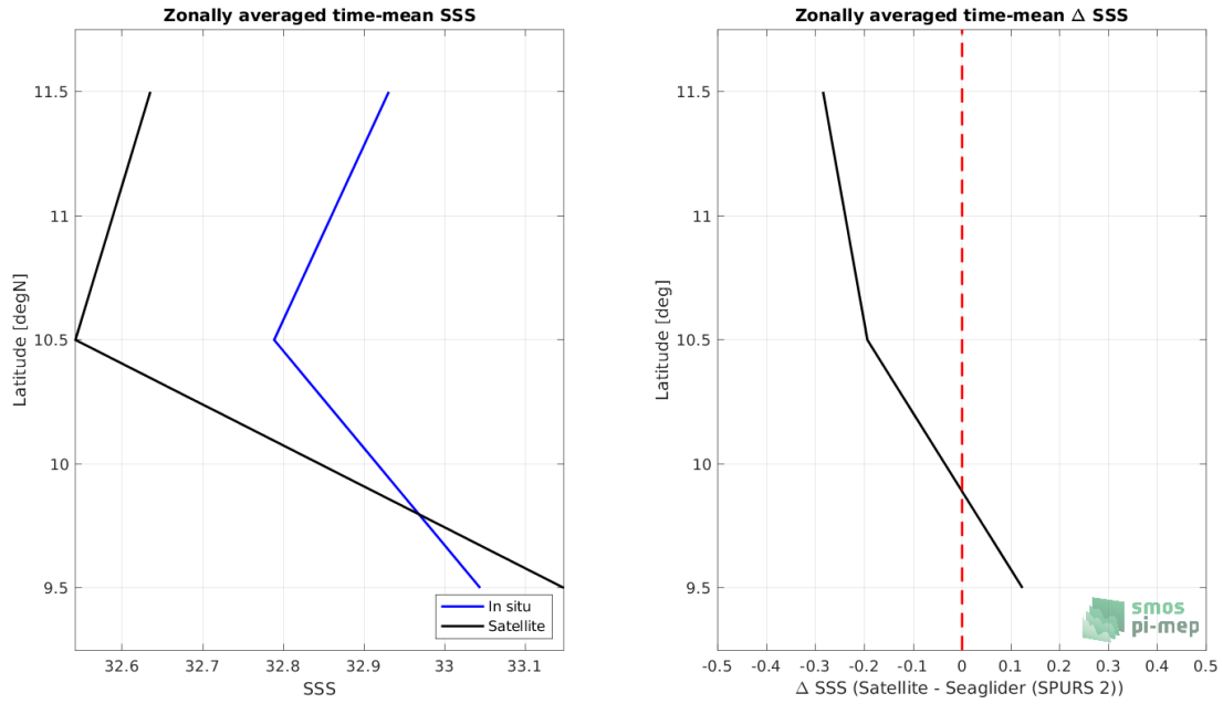
Figure 8: Left panel: Zonal mean SSS from SMOS SSS L2Q v331 - No FLAG (CMEMS-CATDS-CPDC) satellite product (black) and from Seaglider (SPURS 2) (blue). Right panel: Zonal mean of \Delta SSS (Satellite - Seaglider (SPURS 2)) for all the collected Pi-MEP match-up pairs estimated over the full satellite product period.
