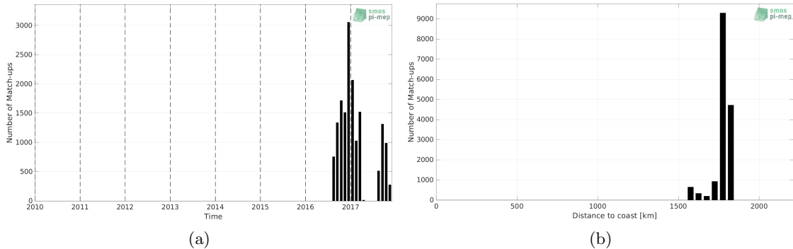
Figure 1: Number of match-ups between Seaglider (SPURS 2) and SMOS SSS L2Q v331 - No FLAG (CMEMS-CATDS-CPDC) SSS as a function of time (a) and as function of the distance to coast (b) over the SPURS 2 Pi-MEP region and for the full satellite product period.
