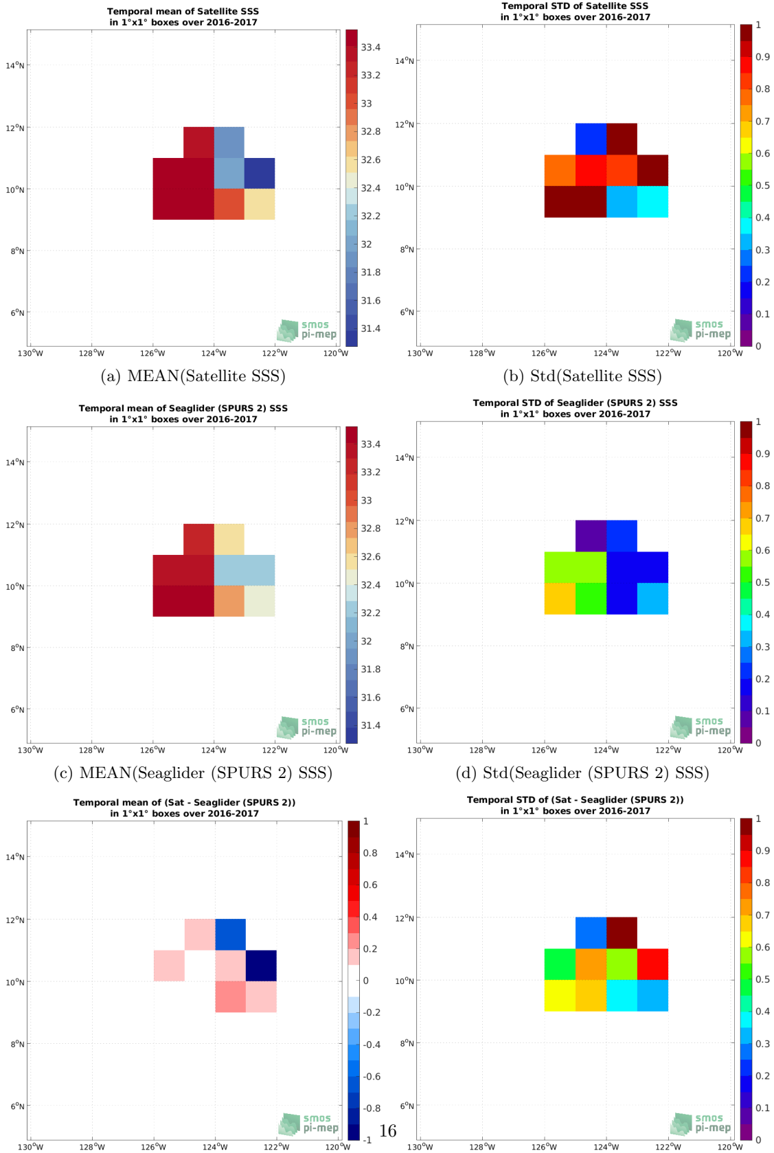
Figure 6: Temporal mean (left) and Std (right) of SSS from SMOS SSS L2Q v331 - No FLAG (CMEMS-CATDS-CPDC) (top), Seaglider (SPURS 2) (middle), and of \Delta SSS (Satellite - Seaglider (SPURS 2)). Only match-up pairs are used to generate these maps.
