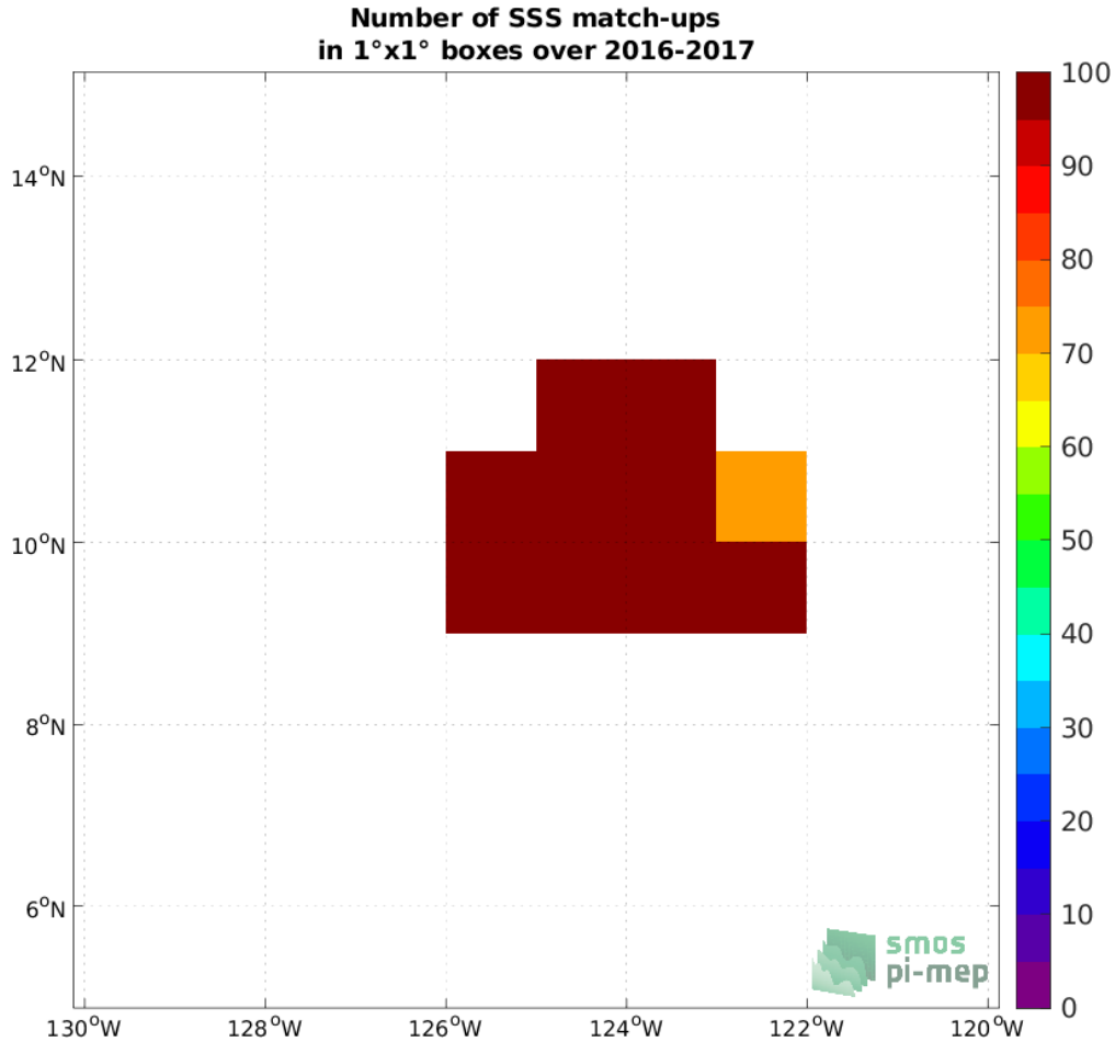
Figure 4: Number of SSS match-ups between Seaglider (SPURS 2) SSS and the SMOS SSS L2Q v331 - No FLAG (CMEMS-CATDS-CPDC) SSS product for the SPURS 2 Pi-MEP region over 1^\circ \times 1^\circ boxes and for the full satellite product period.
