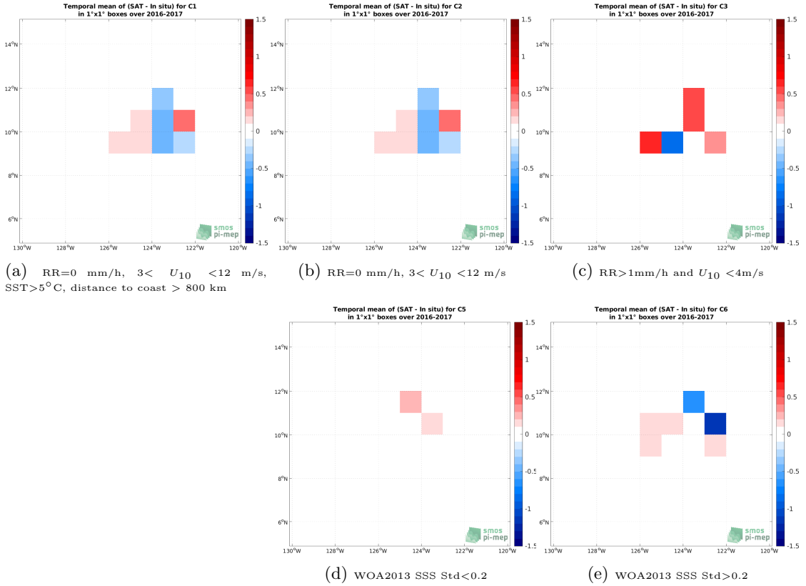
Figure 12: Temporal mean gridded over spatial boxes of size 1^{\circ}\times 1^{\circ} of \Delta\text{SSS} (SMOS SSS L2Q v331 - No FLAG (CMEMS-CATDS-CPDC) - Seaglider (SPURS 2)) for 5 different subdatasets corresponding to:RR=0 mm/h, 3 < U_{10} < 12 m/s, SST >5^{\circ}\text{C} , distance to coast > 800 km (a), RR=0 mm/h, 3 < U_{10} < 12 m/s (b), RR >1 mm/h and U_{10} < 4 m/s (c), WOA2013 SSS Std <0.2 (d), WOA2013 SSS Std >0.2 (e).
