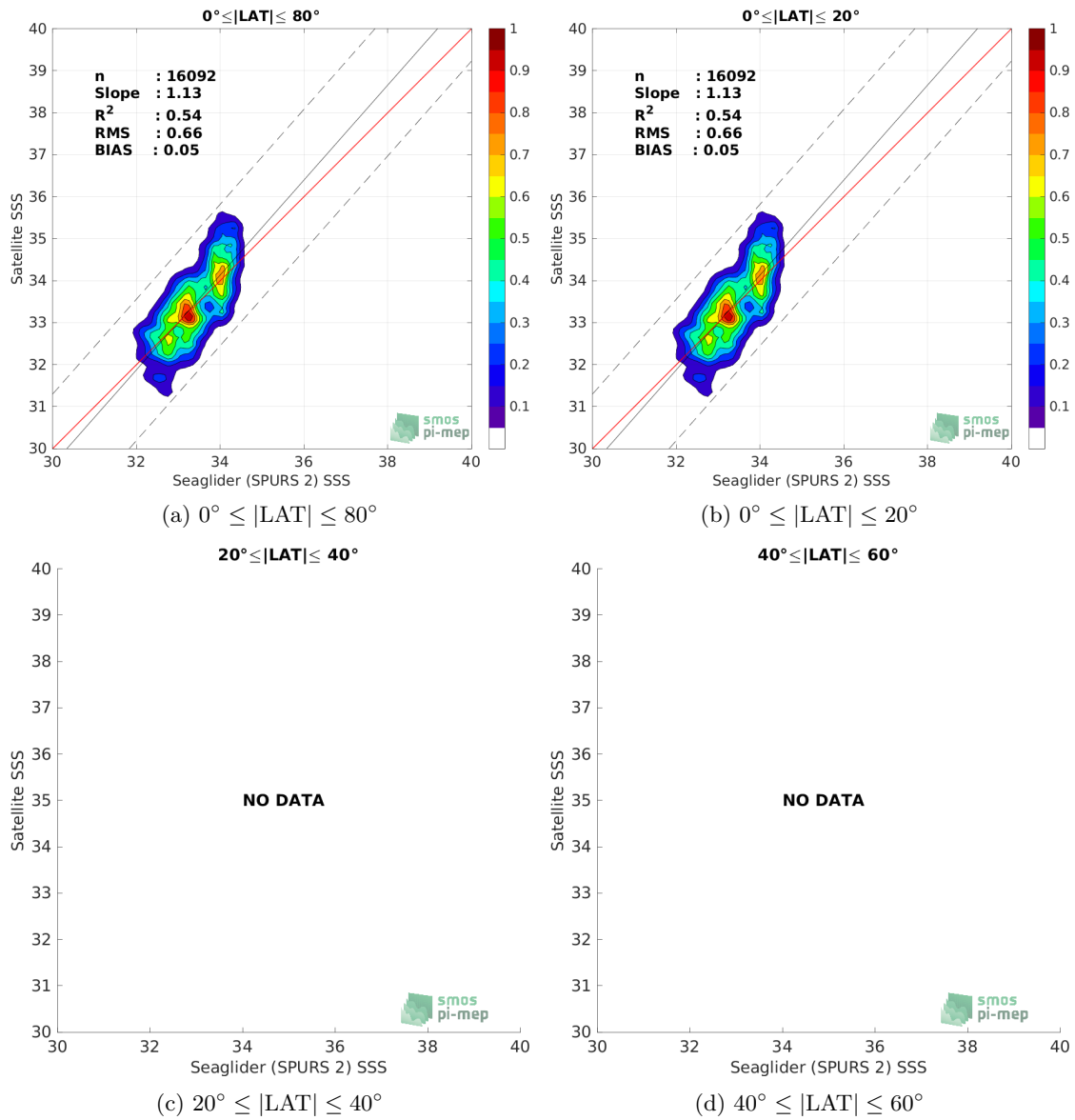
Figure 9: Contour maps of the concentration of SMOS SSS L2Q v331 - No FLAG (CMEMS-CATDS-CPDC) SSS (y-axis) versus Seaglider (SPURS 2) SSS (x-axis) at match-up pairs for different latitude bands. For each plot, the red line shows x=y . The black thin and dashed lines indicate a linear fit through the data cloud and the \pm 95\% confidence levels, respectively. The number match-up pairs n , the slope and R^2 coefficient of the linear fit, the root mean square (RMS) and the mean bias between satellite and in situ data are indicated for each latitude band in each plots.
