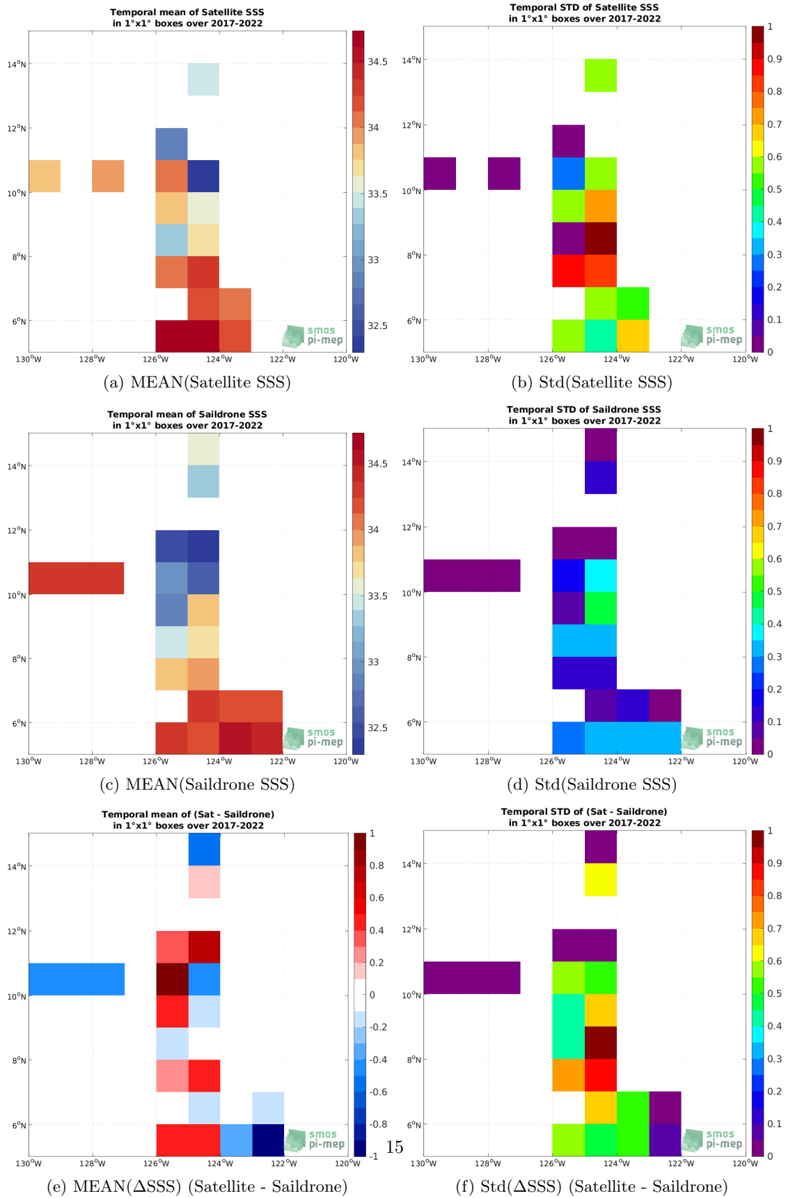
Figure 6: Temporal mean (left) and Std (right) of SSS from SMOS SSS L2Q v331 - No FLAG (CMEMS-CATDS-CPDC) (top), Saildrone (middle), and of \Delta SSS (Satellite - Saildrone). Only match-up pairs are used to generate these maps.
