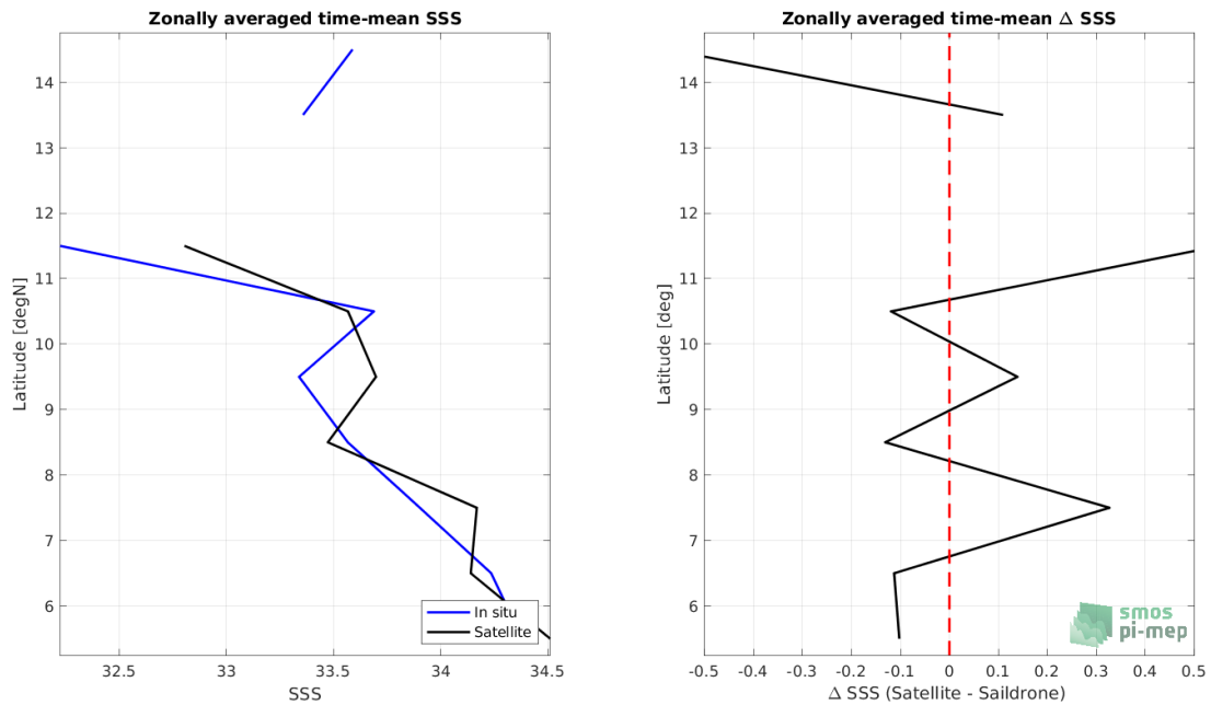
Figure 8: Left panel: Zonal mean SSS from SMOS SSS L2Q v331 - No FLAG (CMEMS-CATDS-CPDC) satellite product (black) and from Sairdron (blue). Right panel: Zonal mean of \Delta SSS (Satellite - Sairdron) for all the collected Pi-MEP match-up pairs estimated over the full satellite product period.
