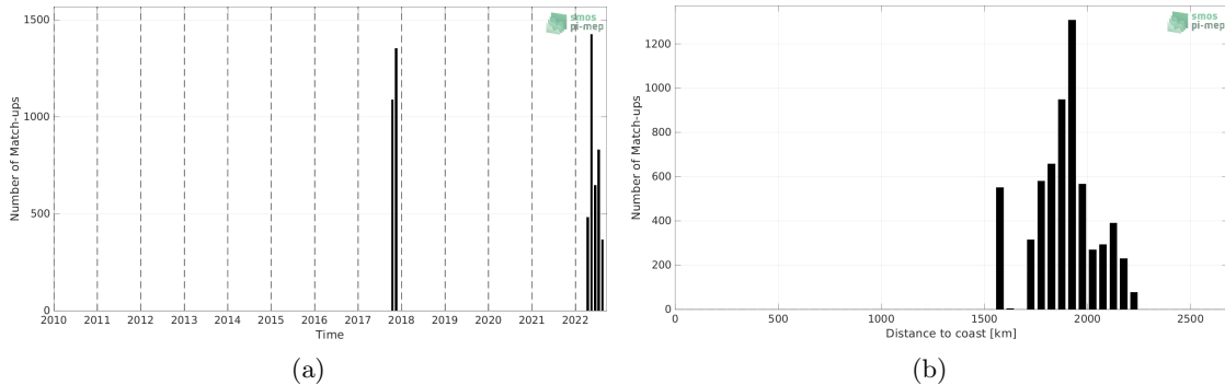
Figure 1: Number of match-ups between Saildrone and SMOS SSS L2Q v331 - No FLAG (CMEMS-CATDS-CPDC) SSS as a function of time (a) and as function of the distance to coast (b) over the SPURS 2 Pi-MEP region and for the full satellite product period.
