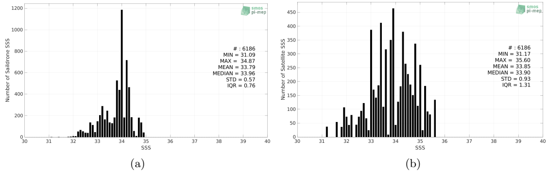
Figure 2: Histograms of SSS from Saildrone (a) and SMOS SSS L2Q v331 - No FLAG (CMEMS-CATDS-CPDC) (b) considering all match-up pairs per bins of 0.1 over the SPURS 2 Pi-MEP region and for the full satellite product period.
