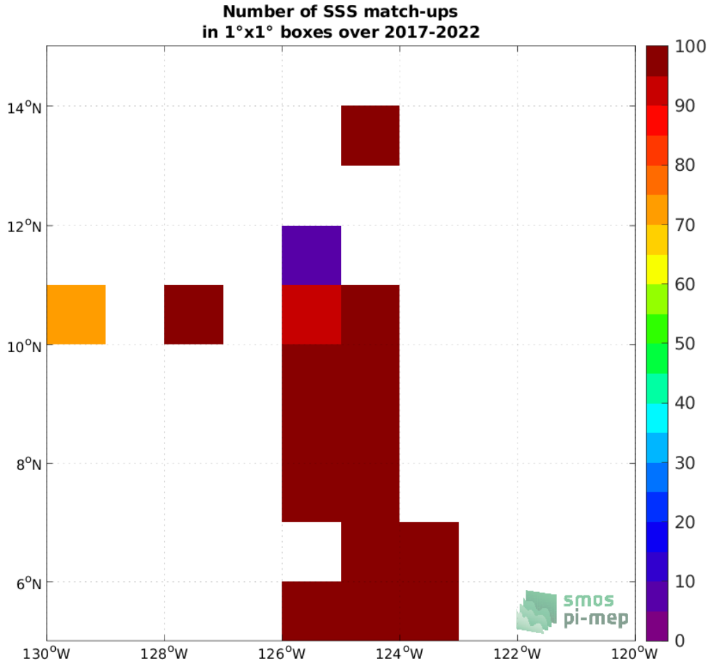
Figure 4: Number of SSS match-ups between Saildrone SSS and the SMOS SSS L2Q v331 - No FLAG (CMEMS-CATDS-CPDC) SSS product for the SPURS 2 Pi-MEP region over 1^\circ \times 1^\circ boxes and for the full satellite product period.
