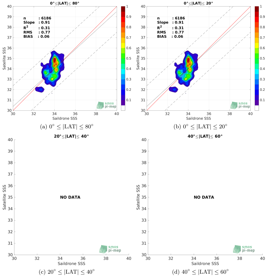
Figure 9: Contour maps of the concentration of SMOS SSS L2Q v331 - No FLAG (CMEMS-CATDS-CPDC) SSS (y-axis) versus Sailability SSS (x-axis) at match-up pairs for different latitude bands. For each plot, the red line shows x=y . The black thin and dashed lines indicate a linear fit through the data cloud and the \pm 95\% confidence levels, respectively. The number match-up pairs n , the slope and R^2 coefficient of the linear fit, the root mean square (RMS) and the mean bias between satellite and in situ data are indicated for each latitude band in each plots.
