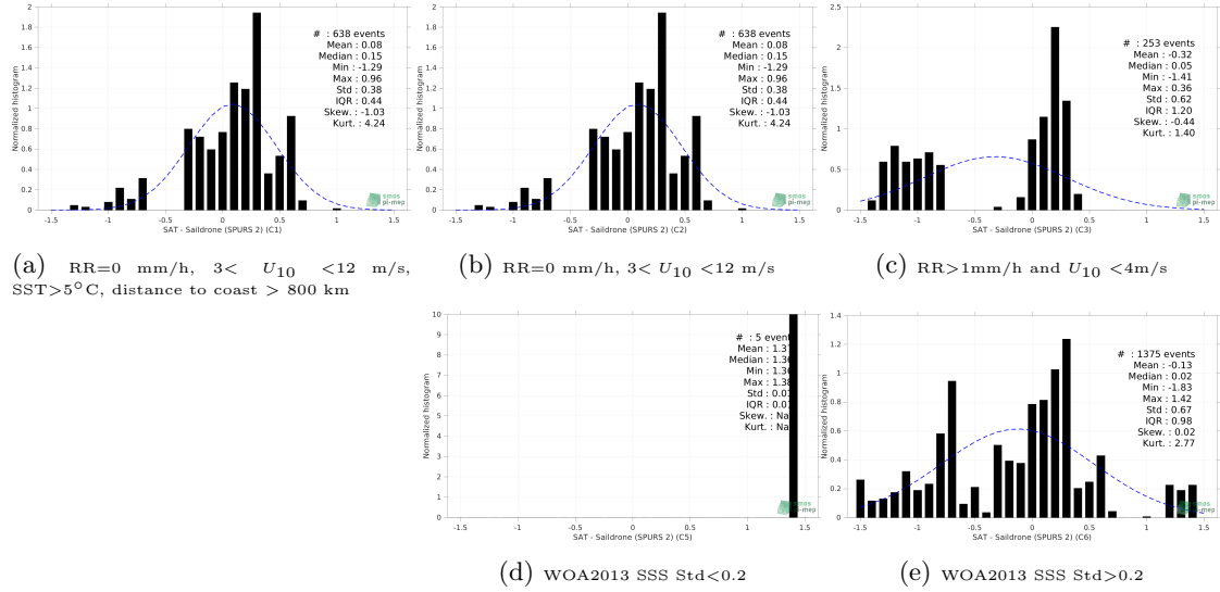
Figure 13: Normalized histogram of \Delta SSS (SMOS SSS L2Q v331 - No FLAG (CMEMS-CATDS-CPDC) - Saildrone (SPURS 2)) for 5 different subdatasets corresponding to: RR=0 mm/h, 3 < U_{10} < 12 m/s, SST>5°C, distance to coast > 800 km (a), RR=0 mm/h, 3 < U_{10} < 12 m/s (b), RR>1mm/h and U_{10} < 4 m/s (c), WOA2013 SSS Std<0.2 (d), WOA2013 SSS Std>0.2 (e).
