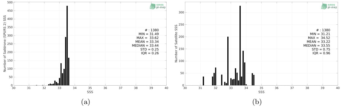
Figure 2: Histograms of SSS from Sairdrone (SPURS 2) (a) and SMOS SSS L2Q v331 - No FLAG (CMEMS-CATDS-CPDC) (b) considering all match-up pairs per bins of 0.1 over the SPURS 2 Pi-MEP region and for the full satellite product period.
