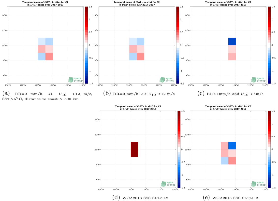
Figure 12: Temporal mean gridded over spatial boxes of size 1^{\circ}\times 1^{\circ} of \Delta\text{SSS} (SMOS SSS L2Q v331 - No FLAG (CMEMS-CATDS-CPDC) - Saldrone (SPURS 2)) for 5 different subdatasets corresponding to:RR=0 mm/h, 3 < U_{10} < 12 m/s, SST >5^{\circ}\text{C} , distance to coast > 800 km (a), RR=0 mm/h, 3 < U_{10} < 12 m/s (b), RR >1 mm/h and U_{10} < 4 m/s (c), WOA2013 SSS Std <0.2 (d), WOA2013 SSS Std >0.2 (e).
