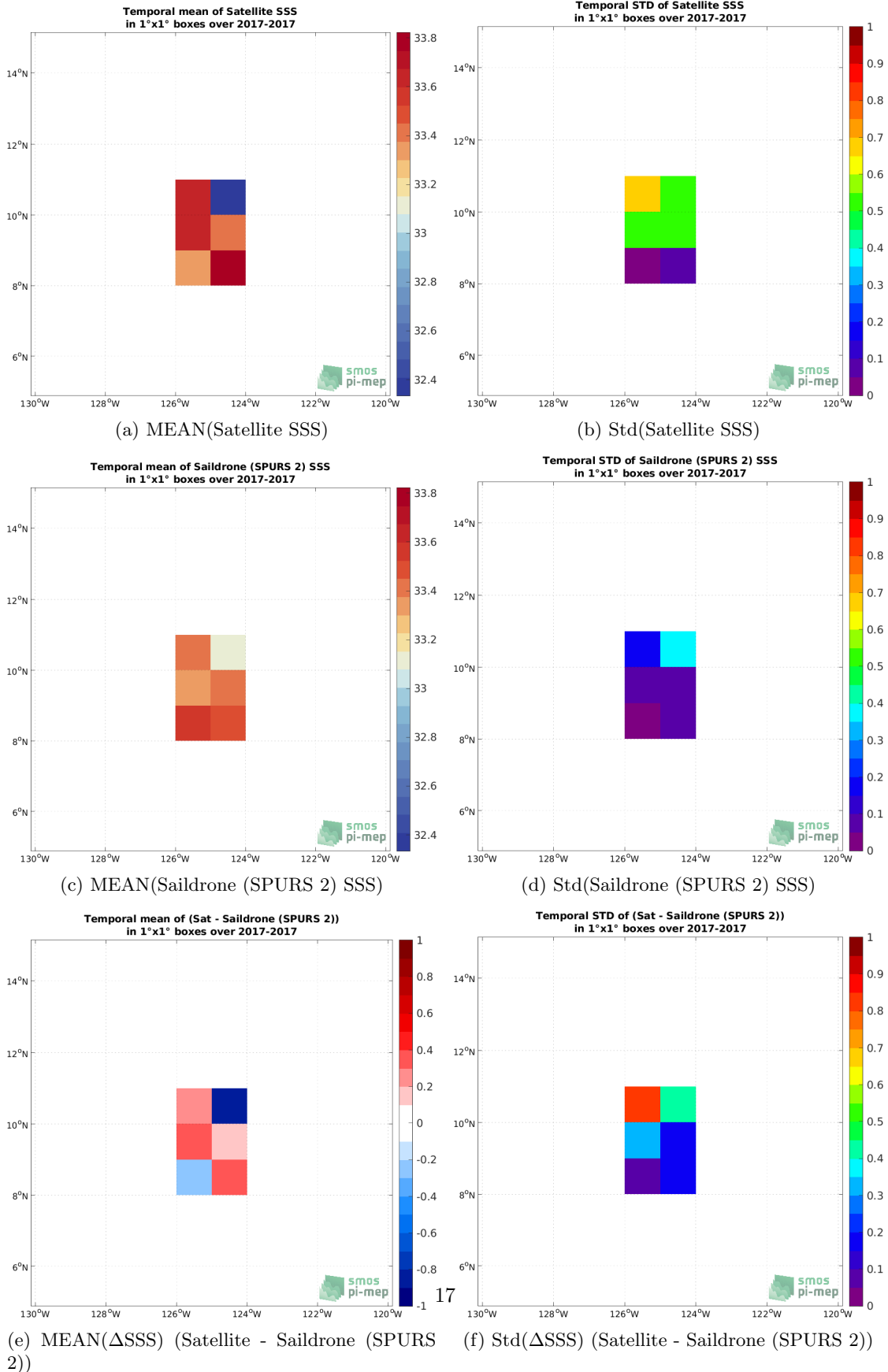
Figure 6: Temporal mean (left) and Std (right) of SSS from SMOS SSS L2Q v331 - No FLAG (CMEMS-CATDS-CPDC) (top), Saildrone (SPURS 2) (middle), and of \Delta SSS (Satellite - Saildrone (SPURS 2)). Only match-up pairs are used to generate these maps.
