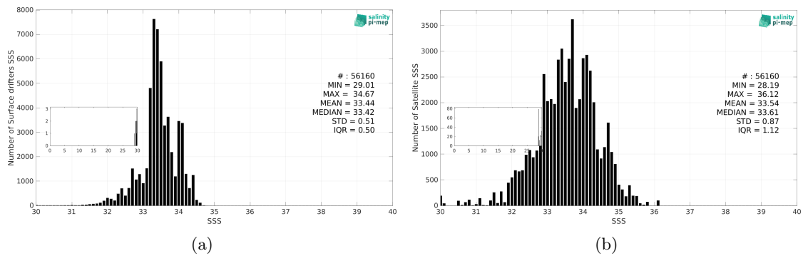
Figure 3: Histograms of SSS from Surface drifters (a) and SMOS SSS L2Q v331 - No FLAG (CMEMS-CATDS-CPDC) (b) considering all match-up pairs per bins of 0.1 over the SPURS 2 Pi-MEP region and for the full satellite product period.
