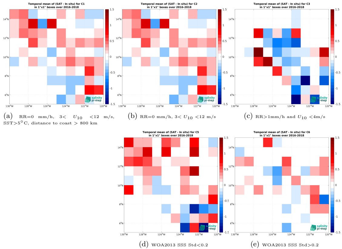
Figure 13: Temporal mean gridded over spatial boxes of size 1^\circ \times 1^\circ of \Delta\text{SSS} (SMOS SSS L2Q v331 - No FLAG (CMEMS-CATDS-CPDC) - Surface drifters) for 5 different subdatasets corresponding to:RR=0 mm/h, 3 < U_{10} < 12 m/s, SST >5^\circ\text{C} , distance to coast > 800 km (a), RR=0 mm/h, 3 < U_{10} < 12 m/s (b), RR >1 mm/h and U_{10} < 4 m/s (c), WOA2013 SSS Std <0.2 (d), WOA2013 SSS Std >0.2 (e).
