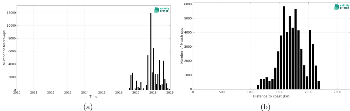
Figure 2: Number of match-ups between Surface drifters and SMOS SSS L2Q v331 - No FLAG (CMEMS-CATDS-CPDC) SSS as a function of time (a) and as function of the distance to coast (b) over the SPURS 2 Pi-MEP region and for the full satellite product period.
