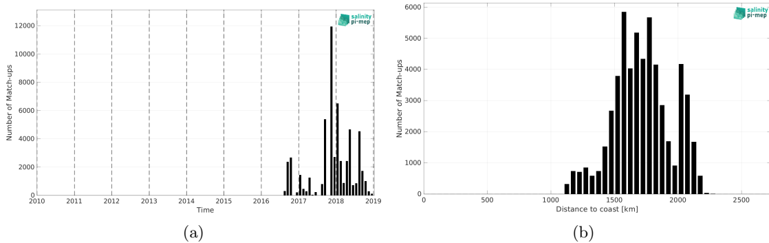
Figure 1: Number of match-ups between Surface drifters and SMOS SSS L2Q v331 - No FLAG (CMEMS-CATDS-CPDC) SSS as a function of time (a) and as function of the distance to coast (b) over the SPURS 2 Pi-MEP region and for the full satellite product period.
