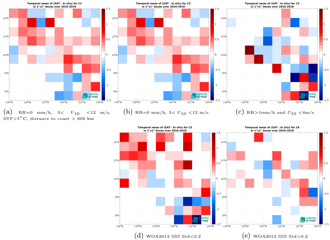
Figure 11: Temporal mean gridded over spatial boxes of size 1^{\circ}\times 1^{\circ} of \Delta\text{SSS} (SMOS SSS L2Q v331 - No FLAG (CMEMS-CATDS-CPDC) - Surface drifters) for 5 different subdatasets corresponding to:RR=0 mm/h, 3 < U_{10} < 12 m/s, SST >5^{\circ}\text{C} , distance to coast > 800 km (a), RR=0 mm/h, 3 < U_{10} < 12 m/s (b), RR >1 mm/h and U_{10} < 4 m/s (c), WOA2013 SSS Std <0.2 (d), WOA2013 SSS Std >0.2 (e).
