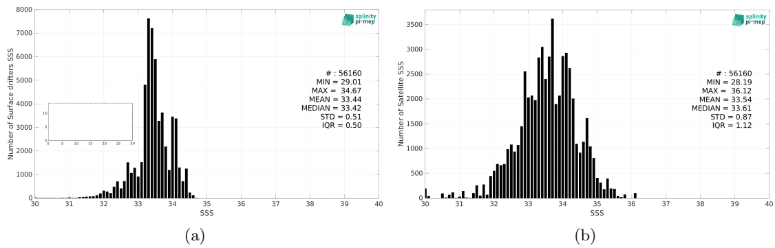
Figure 2: Histograms of SSS from Surface drifters (a) and SMOS SSS L2Q v331 - No FLAG (CMEMS-CATDS-CPDC) (b) considering all match-up pairs per bins of 0.1 over the SPURS 2 Pi-MEP region and for the full satellite product period.
