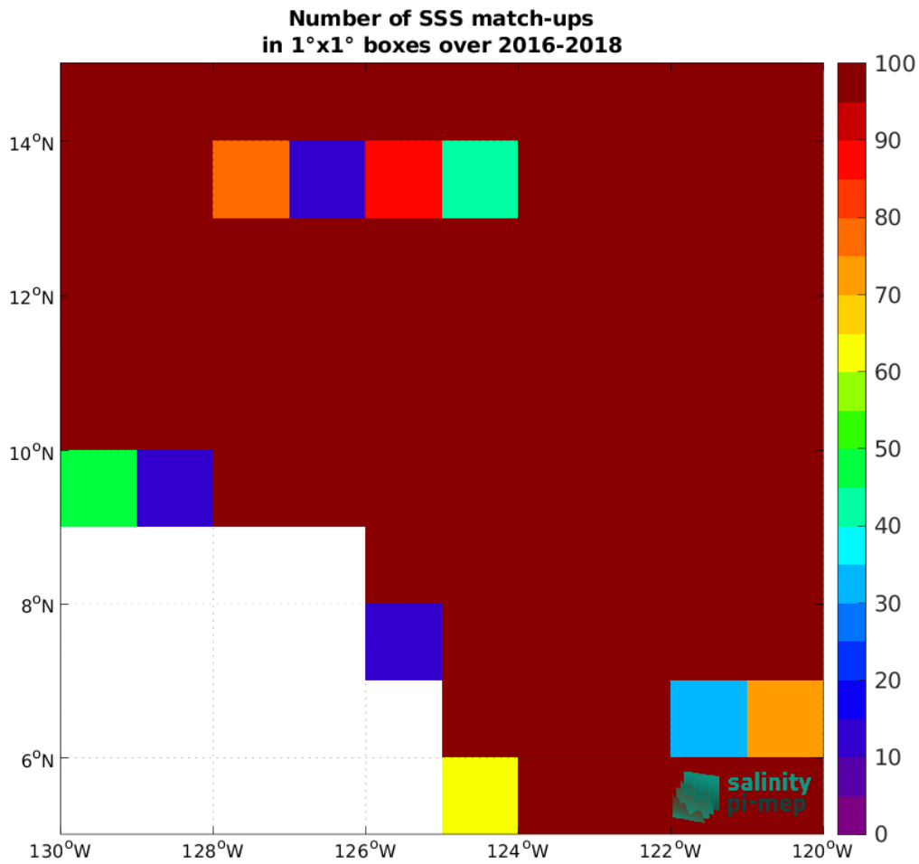
Figure 3: Number of SSS match-ups between Surface drifters SSS and the SMOS SSS L2Q v331 - No FLAG (CMEMS-CATDS-CPDC) SSS product for the SPURS 2 Pi-MEP region over 1°x1° boxes and for the full satellite product period.
