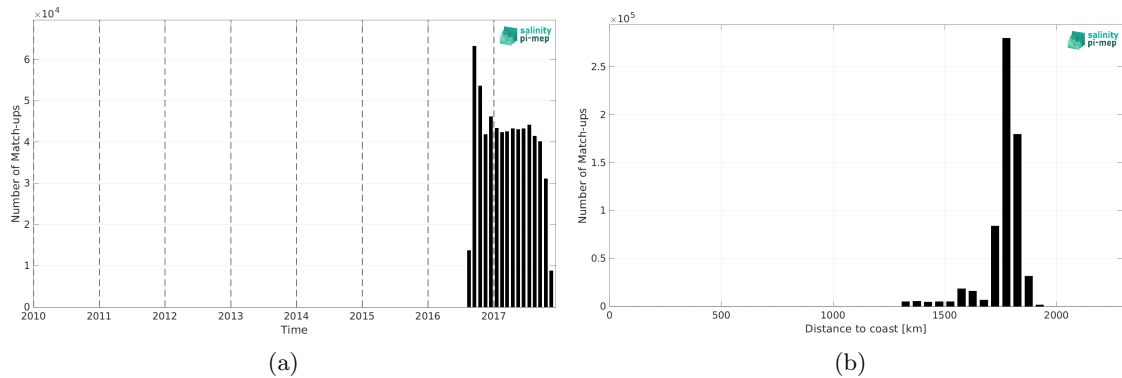
Figure 2: Number of match-ups between Waveglider (SPURS 2) and SMOS SSS L3 v9 - 9 Days (CATDS-CEC-LOCEAN) SSS as a function of time (a) and as function of the distance to coast (b) over the SPURS 2 Pi-MEP region and for the full satellite product period.
