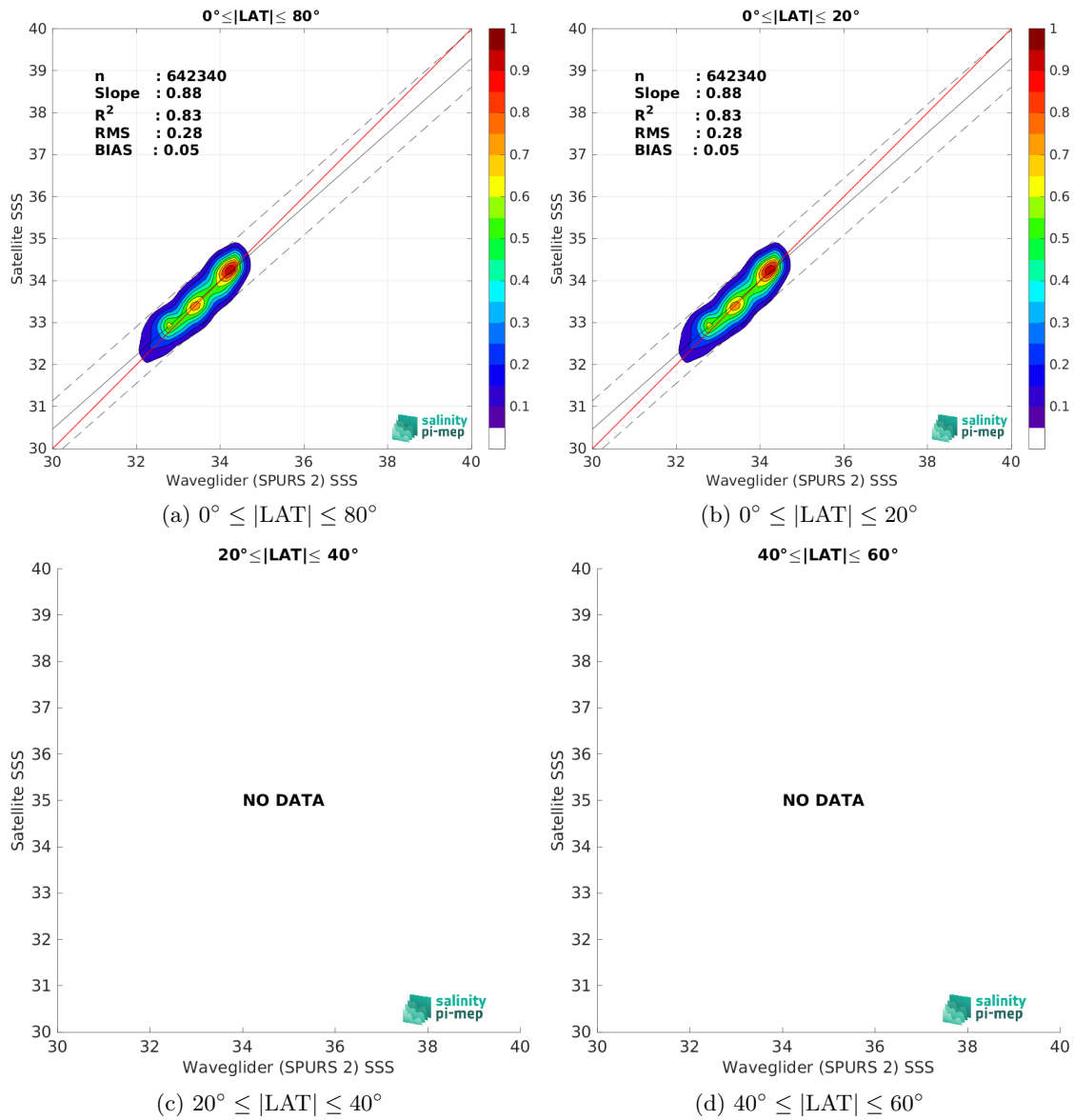
Figure 10: Contour maps of the concentration of SMOS SSS L3 v9 - 9 Days (CATDS-CEC-LOCEAN) SSS (y-axis) versus Waveglider (SPURS 2) SSS (x-axis) at match-up pairs for different latitude bands. For each plot, the red line shows x=y . The black thin and dashed lines indicate a linear fit through the data cloud and the \pm 95\% confidence levels, respectively. The number match-up pairs n , the slope and R^2 coefficient of the linear fit, the root mean square (RMS) and the mean bias between satellite and in situ data are indicated for each latitude band in each plots.
