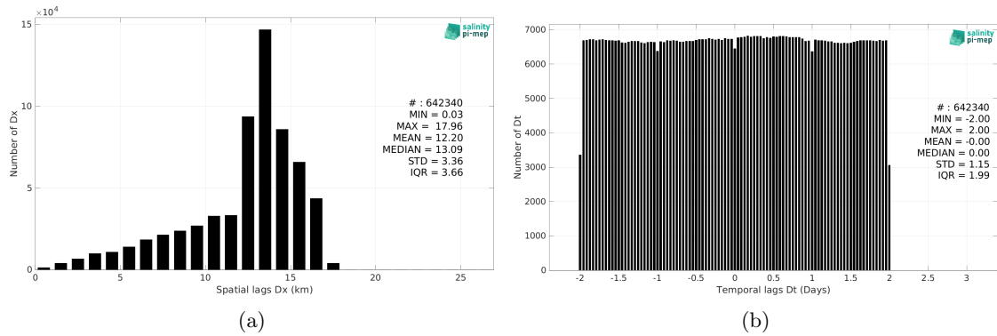
Figure 6: Histograms of the spatial (a) and temporal (b) lags between the location/time of the Waveglider (SPURS 2) measurement and the date of the corresponding SMOS SSS L3 v9 - 9 Days (CATDS-CEC-LOCEAN) SSS pixel.
