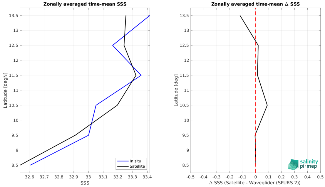
Figure 9: Left panel: Zonal mean SSS from SMOS SSS L3 v9 - 9 Days (CATDS-CEC-LOCEAN) satellite product (black) and from Waveglider (SPURS 2) (blue). Right panel: Zonal mean of \Delta SSS (Satellite - Waveglider (SPURS 2)) for all the collected Pi-MEP match-up pairs estimated over the full satellite product period.
