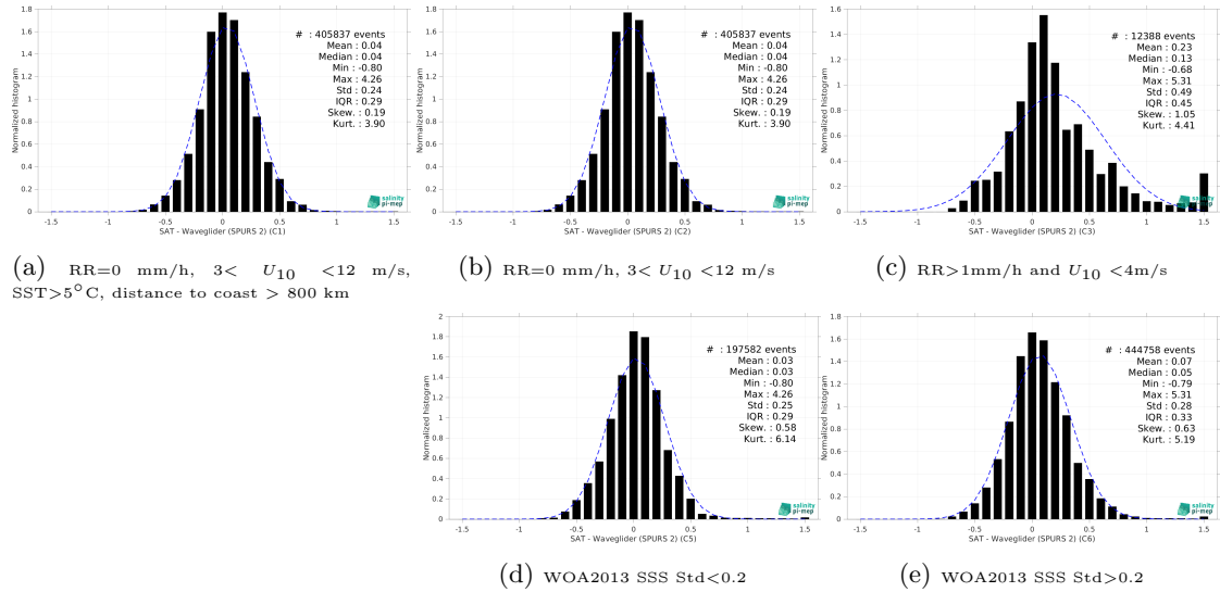
Figure 15: Normalized histogram of \Delta SSS (SMOS SSS L3 v9 - 9 Days (CATDS-CEC-LOCEAN) - Waveglider (SPURS 2)) for 5 different subdatasets corresponding to: RR=0 mm/h, 3 < U_{10} < 12 m/s, SST > 5°C, distance to coast > 800 km (a), RR=0 mm/h, 3 < U_{10} < 12 m/s (b), RR > 1mm/h and U_{10} < 4 m/s (c), WOA2013 SSS Std < 0.2 (d), WOA2013 SSS Std > 0.2 (e).
