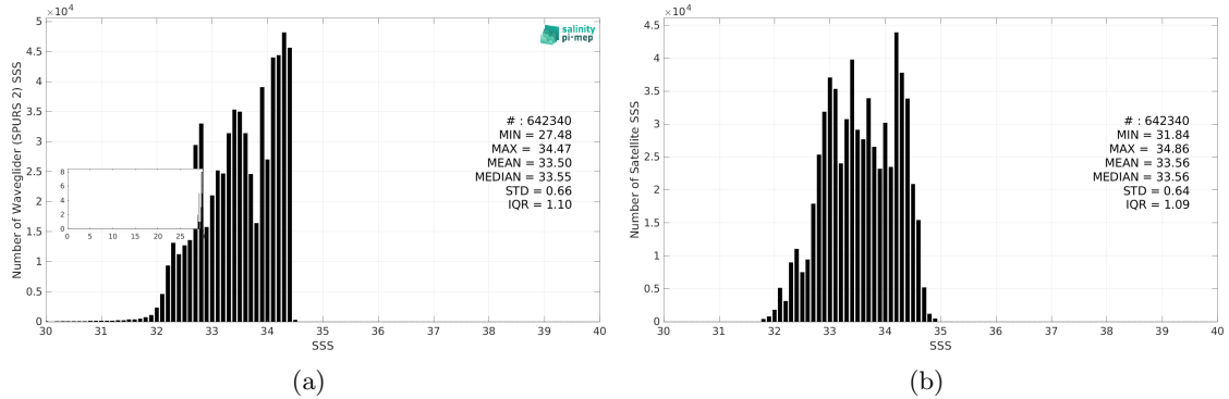
Figure 3: Histograms of SSS from Waveglider (SPURS 2) (a) and SMOS SSS L3 v9 - 9 Days (CATDS-CEC-LOCEAN) (b) considering all match-up pairs per bins of 0.1 over the SPURS 2 Pi-MEP region and for the full satellite product period.
