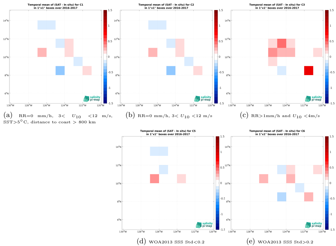
Figure 14: Temporal mean gridded over spatial boxes of size 1^\circ \times 1^\circ of \Delta SSS (SMOS SSS L3 v9 - 9 Days (CATDS-CEC-LOCEAN) - Waveglider (SPURS 2)) for 5 different subdatasets corresponding to:RR=0 mm/h, 3 < U_{10} < 12 m/s, SST>5°C, distance to coast > 800 km (a), RR=0 mm/h, 3 < U_{10} < 12 m/s (b), RR>1mm/h and U_{10} < 4 m/s (c), WOA2013 SSS Std<0.2 (d), WOA2013 SSS Std>0.2 (e).
